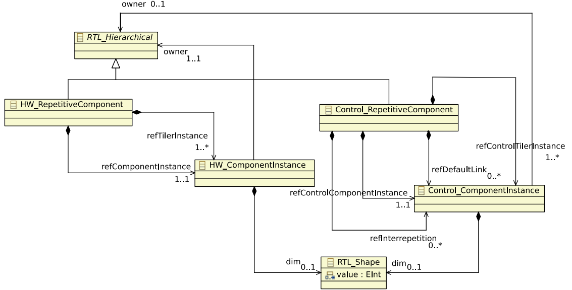
Figure 7.10: Concepts related to repetitive components in the RTL metamodel
