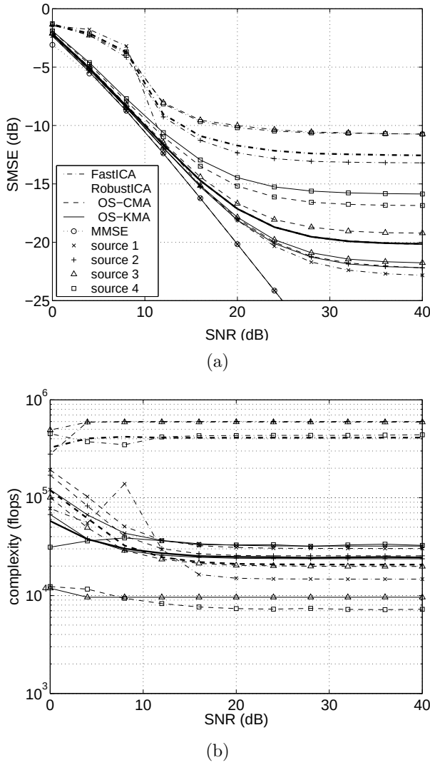
Figure 1: Performance of deflationary ICA algorithms for single-tap initialization: (a) signal extraction quality, (b) computational complexity. Unmarked thick lines represent performance indices averaged over the 4 sources.
