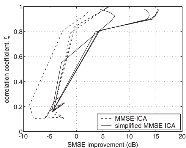
Figure 5. ICA performance gain vs correlation coefficient \zeta for the scenario of Figure 1 and different SNRs.
