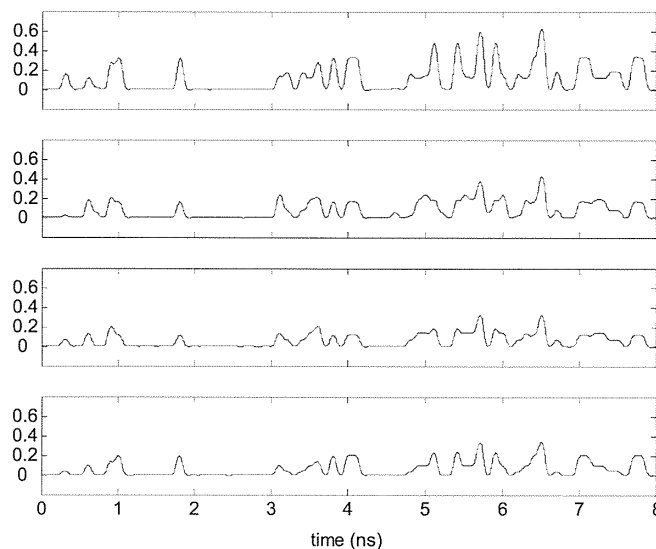
Fig. 4. Observed photocurrents in the four-channel experiment.
