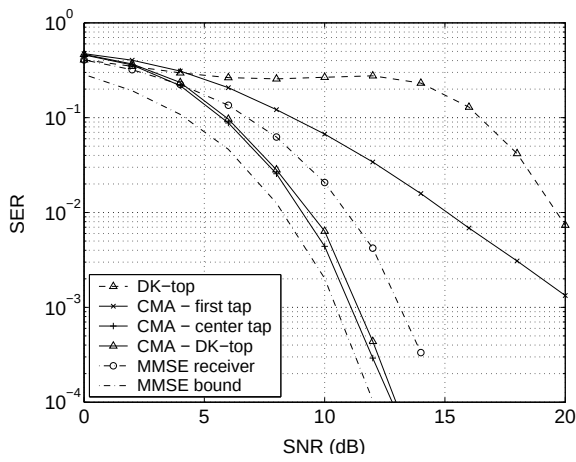
Fig. 1. Blind equalization performance. Solid lines: constant step-size gradient-descent CMA with different initializations.
