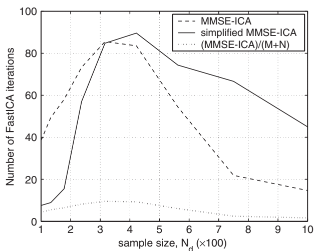
Figure 12. Number of FastICA iterations vs sample size in the simulation of Figure 9.
