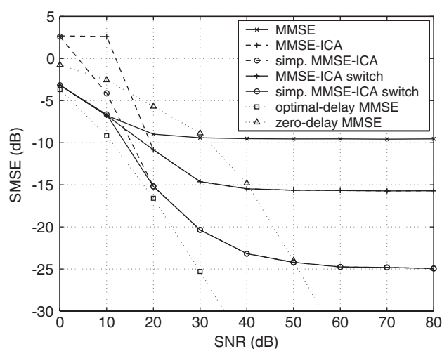
Figure 6. Equalization performance vs SNR, with \text{CMSE} = 0 , N_d = 500 .
