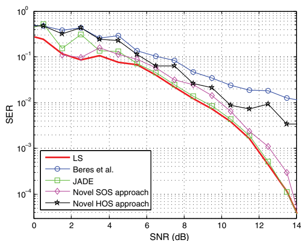
Figure 9. LOS scenario: SER performance versus SNR.
