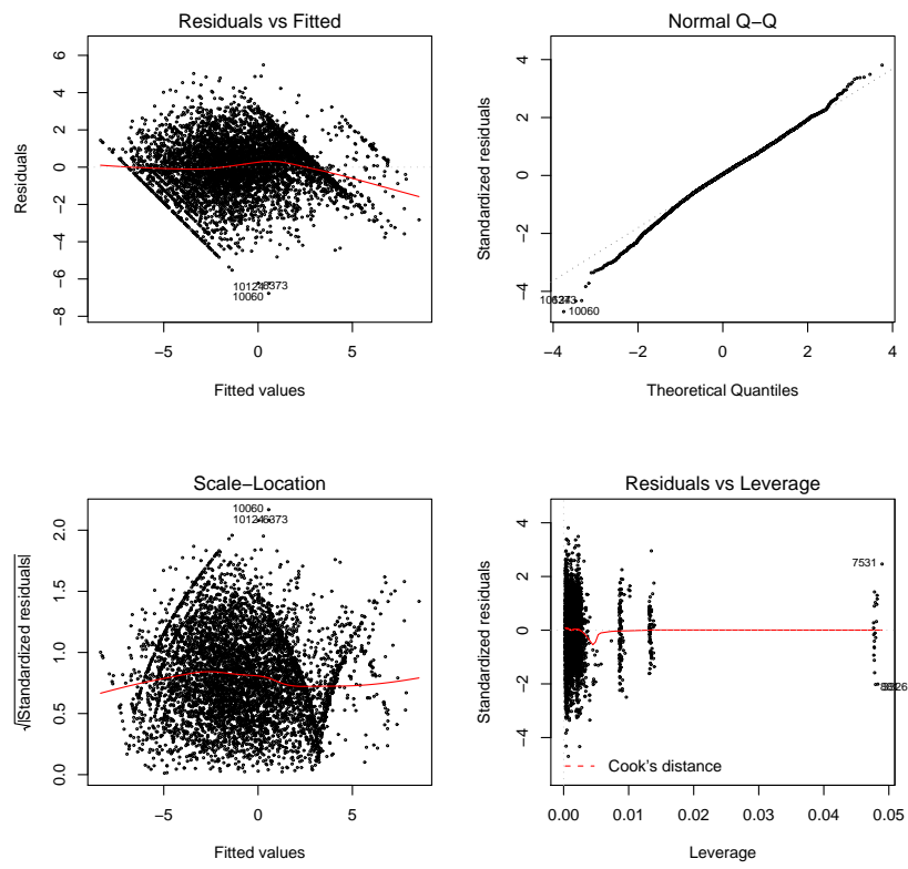
Figure B.1: Residuals of the EOQ model
