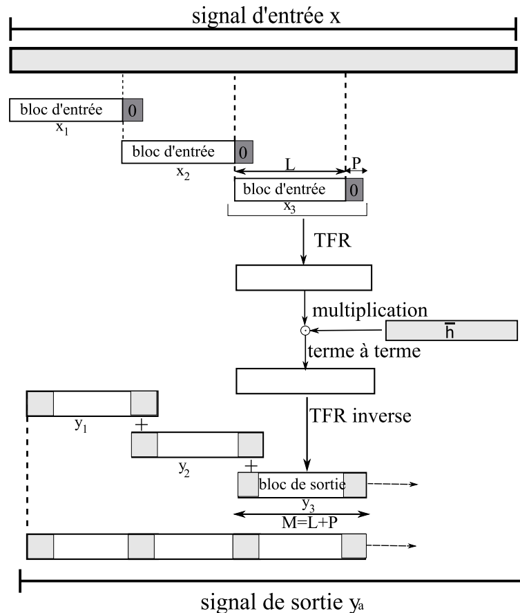
FIGURE 1.5 – Schéma d'overlap-add
