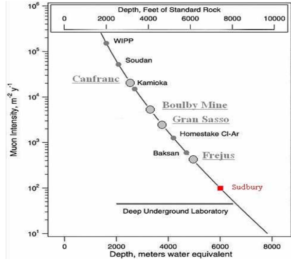
Figure 2.2: Muon intensity in m^{-2} \cdot y^{-1} as a function of depth (meters equivalent).
