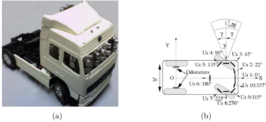
Figure 7.2: (a) The Minitruck platform. (b) Sonar locations. Images courtesy of Emmanuel Seignez [Seignez06].
