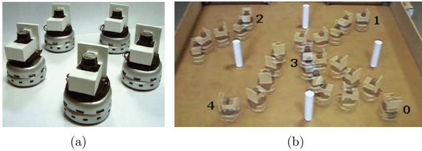
Figure 7.6: (a) 5 Khepera III robots. (b) Stroboscopic motion in the early steps of the experiment. Images courtesy of [Franchi09].
