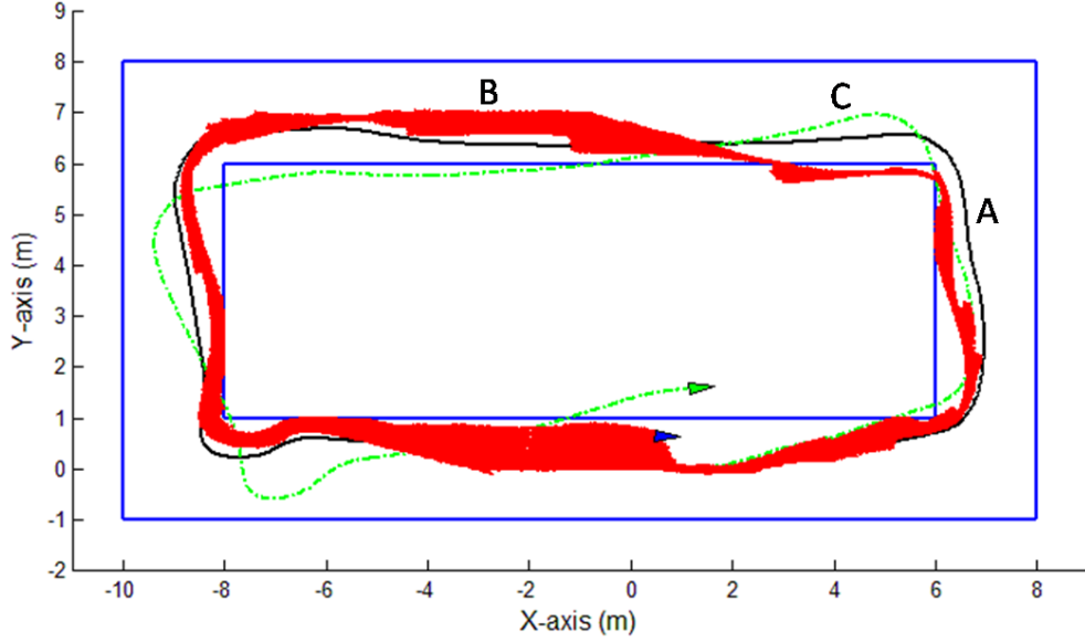
Figure 4.5: Position tracking using MCL in an absolutely symmetrical closed corridor. The trajectories of robot, odometry and particles are displayed by the black solid line (line A), the green dash-dot line (line C) and the red dotted line (line B), respectively.
