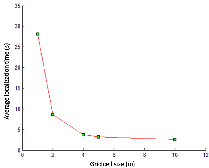
Figure 4.18: Average localization time needed for global localization as a function of grid resolution.
