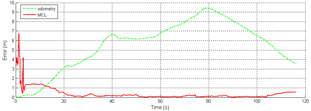
Figure 4.15: Localization errors of global localization using MCL in a quasi-symmetrical corridor. MCL errors and odometry errors are plotted by the red solid line and the green dash-dot line, respectively.
