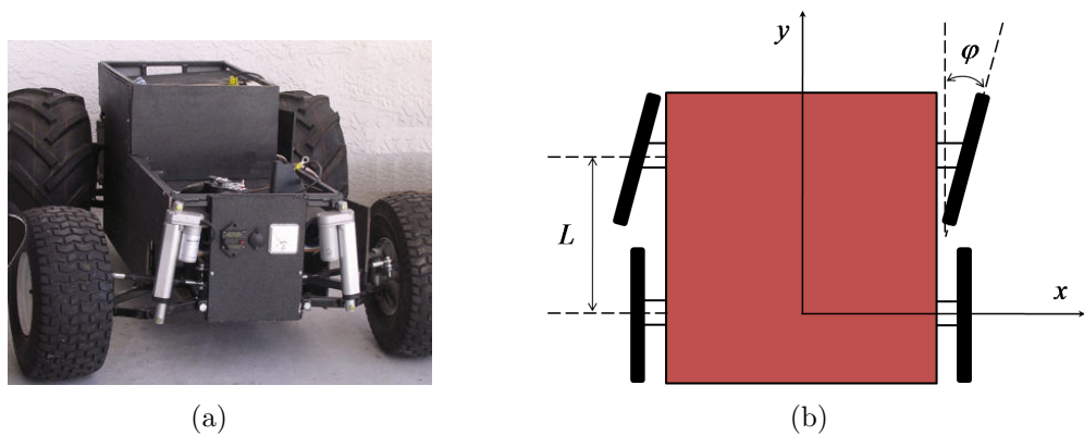
Figure 2.4: Car-like WMR.
