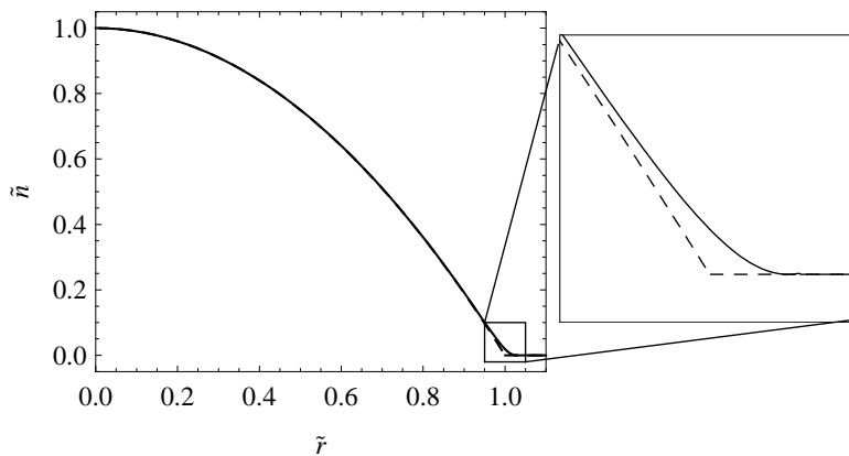
Figure 3.10: Density profile \tilde{n}(\tilde{r}) of a molecular Bose-Einstein condensate calculated using the Gross-Pitaevskii equation (solid line) and the Thomas-Fermi approximation (dashed line). The total molecule number is N = 5 \times 10^4 , the trap frequency is \omega = 2\pi \times 330 Hz, and the scattering length is a = 2000 a_0 (corresponding to a magnetic field B \simeq 750 G).
