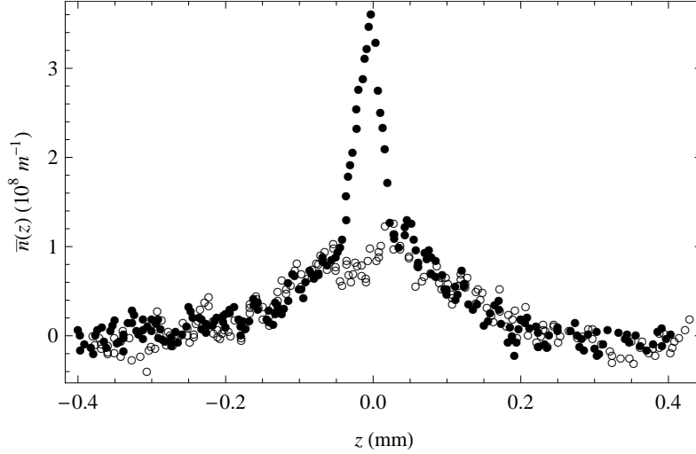
Figure 3.4: Doubly-integrated density profiles of {}^7\text{Li} (dots) and {}^6\text{Li} (open circles). The gas contains 3.5 \times 10^4 {}^7\text{Li} atoms and 2.5 \times 10^4 {}^6\text{Li} atoms.
