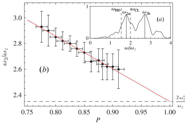
FIG. 4 (color online). (a) Frequency power spectrum of the minority spin state for P = 0.90(2) . The peak between \omega_{\text{HD}} and \omega_{\text{CL}} corresponds to the oscillation in phase with the majority, the other one to the polaron oscillation. (b) Frequency of the polaron component as a function of polarization. All frequencies are normalized to \omega_z .
