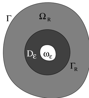
FIG. 4.1. The truncated domain.
