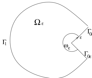
17 Fig. 2. The perturbed domain.
