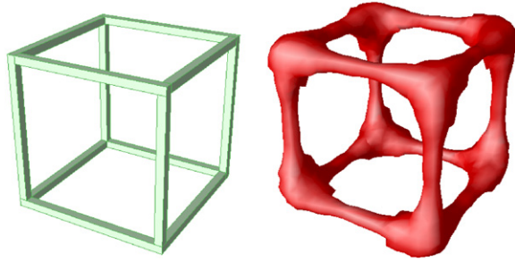
Figure 4. Metallic edges of a cube and an iso-value surface of the corresponding topological sensitivity (computed in free space as an initial guess).
