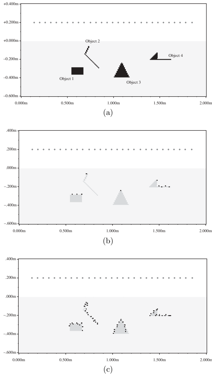
FIG. 7.3. (a) Redistribution of objects. The measures are computed on a dry flat inhomogeneous soil ( \epsilon_s = 2.3 ), 29 measurement points, and 20 frequencies ranging from 490MHz to 3.29GHz. (b) Iteration 10. (c) Iteration 55.
