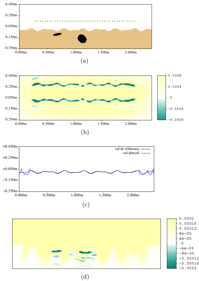
Figure 3. Topological sensitivity in two steps. (a) Reference distribution (41 measurement points; 30 frequencies in the range 0.33 GHz–1 GHz; wet soil ( \epsilon_s = 13 , \sigma_s = 0.05 )), (b) topological asymptotic computed on an empty initial guess (no soil at all), with respect to small balls of undergrass, (c) detected soil surface and (d) topological sensitivity taking into account the detected soil surface.
