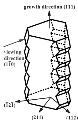
Figure 5.13: Schematic of the three dimensional structure of a wire. The cross section of each wire is a trigonal hexagon with three long and three short edges. One in two sidewall facets contains a periodic sawtooth faceting in the growth direction (Ross et al., 2005).
