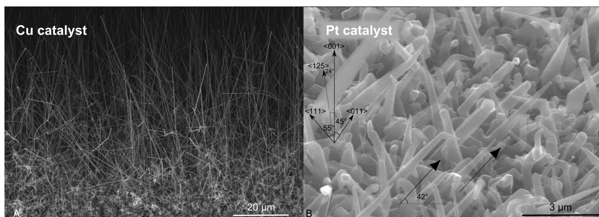
Figure 6.21: SEM image of nanowire grown with (A) a Cu catalyst on a silicon \langle 111 \rangle substrate, and (B) a Pt catalyst on a silicon \langle 100 \rangle substrate.
