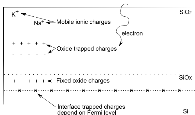
Figure 7.11: Schematic illustrating the different possible types of charges that can be present in the oxide or at the oxide-silicon interface (Nicollian and Brews, 1982).
