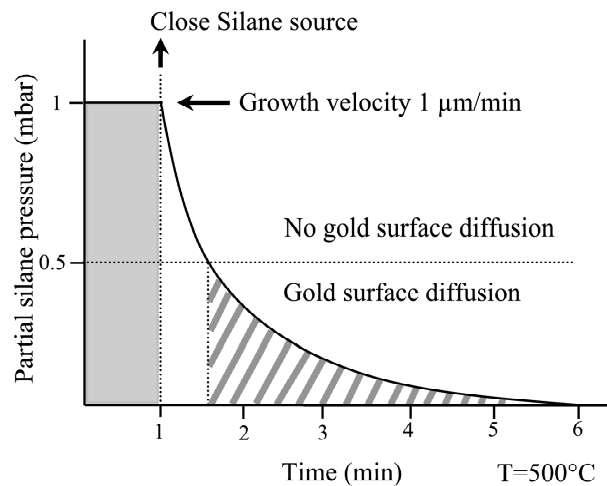
Figure 5.10: Estimated exponential decay of the silane partial pressure in the growth chamber. The silane flow is closed at time t = 1 min. The growth velocity at the starting partial pressure and the partial pressure below which gold surface diffusion can occur at this temperature (for a constant partial pressure value) are indicated. Comparison of the gray surface and the striped surface allows estimating the length the nanowire can grow, during which time gold diffusion can occur. Gold diffusion was observed at a partial pressure of 0.52 mbar (Figure 5.4), but was absent at a partial pressure of 1.023 mbar (Figure 5.7B-C). Somewhere between these two values the gold ceases to diffuse. The lower bound value is indicated in the figure.
