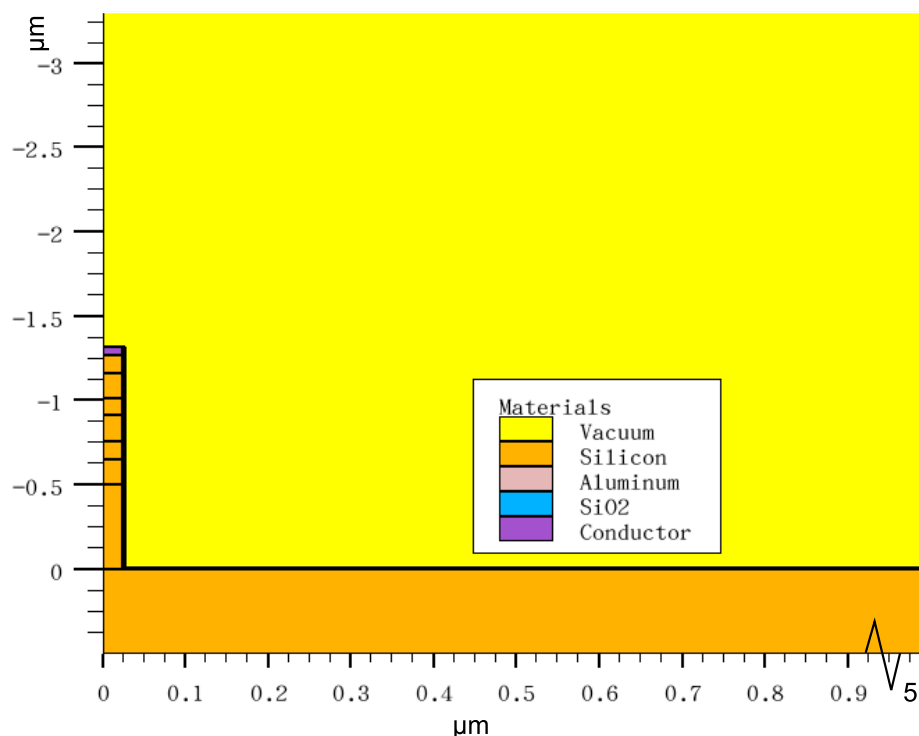
Figure 7.2: Schematic of a 2D cylindrical simulation. Half of the nanowire is visible with the different regions. Around the nanowire vacuum is defined. The catalyst was simulated by using another metal, being alumina, with the workfunction of gold. 3 nm silicon oxide was present on the nanowire sidewalls.
