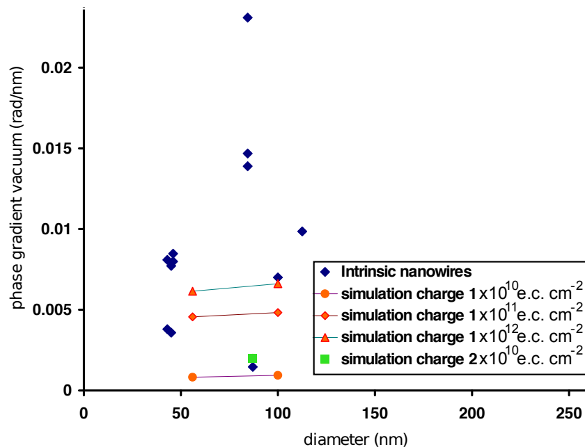
Figure 7.14: Gradient in the vacuum at the side of intrinsic nanowires (blue \diamond ) and simulation of the gradient in the vacuum for a charged nanowire with a sheet charge of 1 \times 10^{10} e.c. \text{cm}^{-2} (orange \circ ), 2 \times 10^{10} e.c. \text{cm}^{-2} (green \square ), 1 \times 10^{11} e.c. \text{cm}^{-2} (orange \diamond ) and 1 \times 10^{12} e.c. \text{cm}^{-2} (orange \triangle ). Lines are drawn between simulations of different wire diameters to guide the eye.
