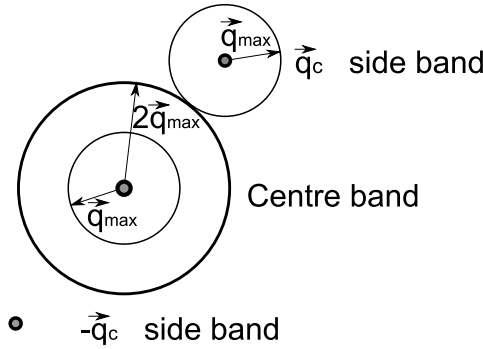
Figure 3.4: A schematic diagram showing the optimum masks in Fourier space for a normal object. The vector modulus \vec{q}_{max} is the largest frequency included in the mask and therefore defines the maximum spatial resolution in the reconstructed object. Adapted from (Midgley, 2001).
