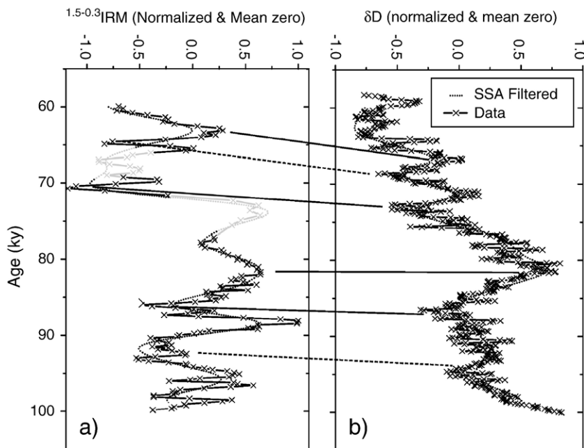
Fig. 10. a) The LAA hematite proxy (3-point running average), b) Vostok \delta\text{D} time series and their filtered counterparts using the first three terms of a SSA transform. The grey LAA data indicate field-identified intervals of resedimentation.
