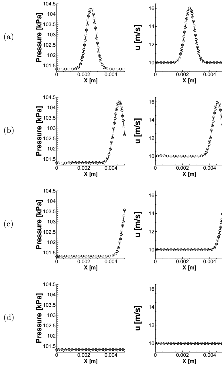
Figure 3.11: Acoustic wave passing through a non-reflective boundary. Pressure (left) and velocity (right) profiles are plotted for multi-component (symbols) and TTC (line) formalism at different times t^+ = tL/a_0 in the simulation. (a) Initial solution, t^+ = 0 ; (b) t^+ = 0.4 ; (c) t^+ = 0.54 ; (d) t^+ = 1.37 .
