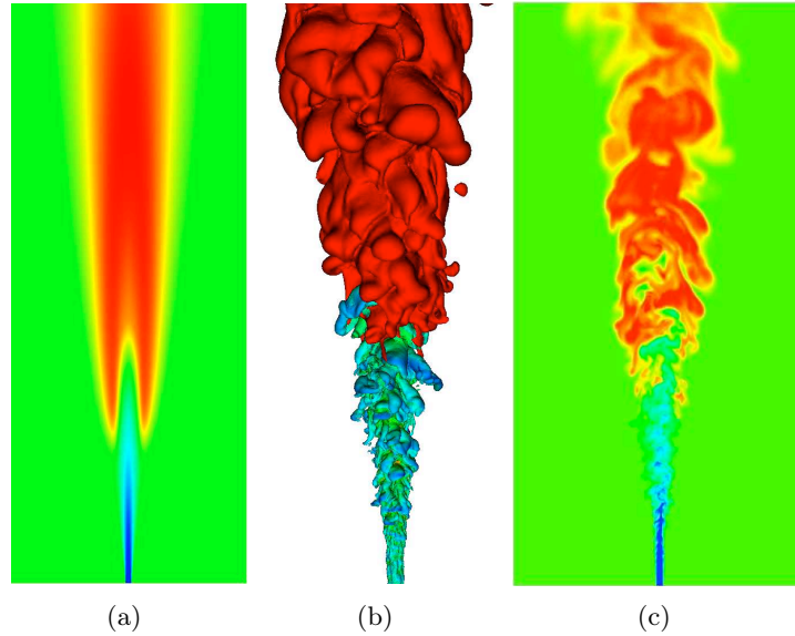
Figure 3: Numerical simulation of the Cabra flame (Cabra et al. , 2005) with RANS (a) and LES (b,c) approaches. (a,c) Plane colored by temperature. (b) Isosurfaces of temperature (colored in red) and mixture fraction (colored by axial velocity).
