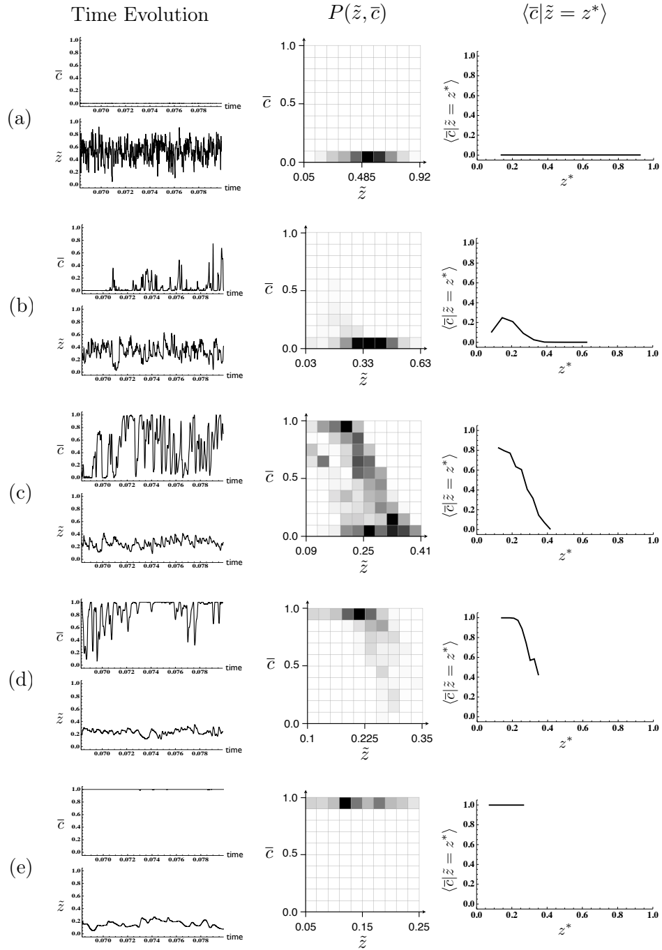
Figure 7.22: Statistical analysis of time signal of \bar{c} and \tilde{z} at several locations on the jet axis: (a) X/d = 20 ; (b) X/d = 30 ; (c) X/d = 40 ; (d) X/d = 50 ; (e) X/d = 75 . First column: time signals \bar{c}(t) and \tilde{z}(t) . Second column: color maps of the joint PDF P(\tilde{z}, \bar{c}) in the discretized \tilde{z} - \bar{c} plane. Third column: profiles of the progress variable conditional mean \langle \bar{c} | \tilde{z} = z^* \rangle .
