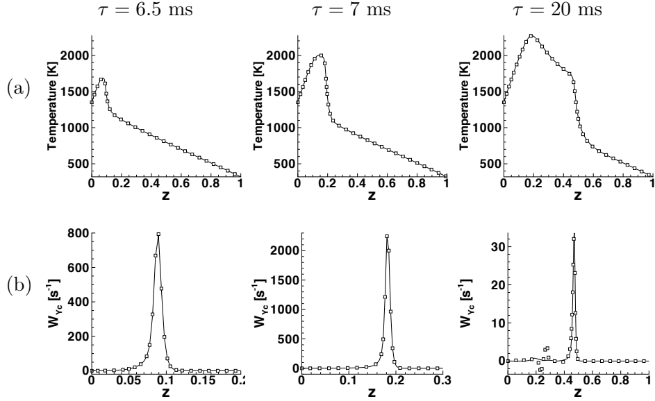
Figure 5.16: Profiles of temperature (a) and source term \dot{\omega}_{Y_c} in s^{-1} (b) at different instants: \tau = 6.5 ms ; 7 ms ; 20 ms. Plain line: reference solution computed with \chi_{st}(\tau) . Square symbols: solution interpolated in the database built for steady scalar dissipation rates.
