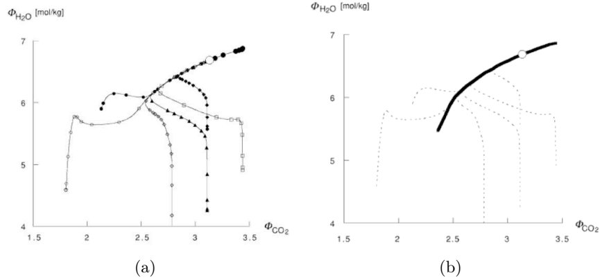
Figure 2.9: Trajectories of chemical reactions (a) and one-dimensional manifold (b) projected in the (CO_2, H_2O) plane. (a) Line with different symbols represents chemical paths from different initial point. (b) Line: 1D-ILDM ; dashed lines: trajectories. The plane coordinates are expressed in weighted mass fractions \phi_i = Y_i/W_i . \circ represents the equilibrium point. (Warnatz et al., 2006).
