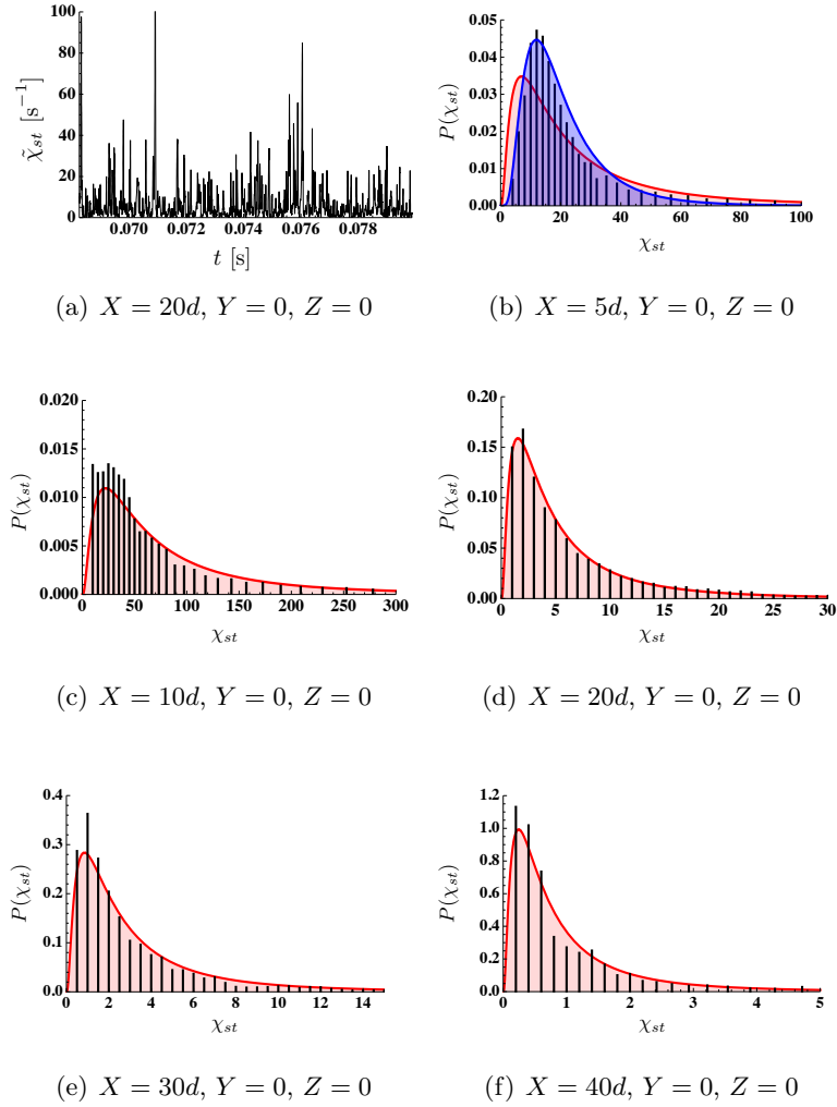
Figure 7.21: Computed PDF P(\chi_{st}) (black bins) compared with log-normal distribution P(\chi_{st}) = \text{LogNormal}(\chi_{st}; \mu, \sigma) (red curve) with \mu = \ln(\tilde{\chi}_{st}) - \sigma^2/2 and \sigma = 1.0 at different locations (b, c, d, e, f). The computed mean \tilde{\chi}_{st} are 31.1 (b), 99.0 (c), 6.8 (d), 3.8 (e) and 1.1 \text{ s}^{-1} (f). An example of the time signal \tilde{\chi}_{st}(t) is given in (a). The best fitting log-normal distribution ( \mu = 2.86, \sigma = 0.62 ) plotted with a blue curve is added in (b).
