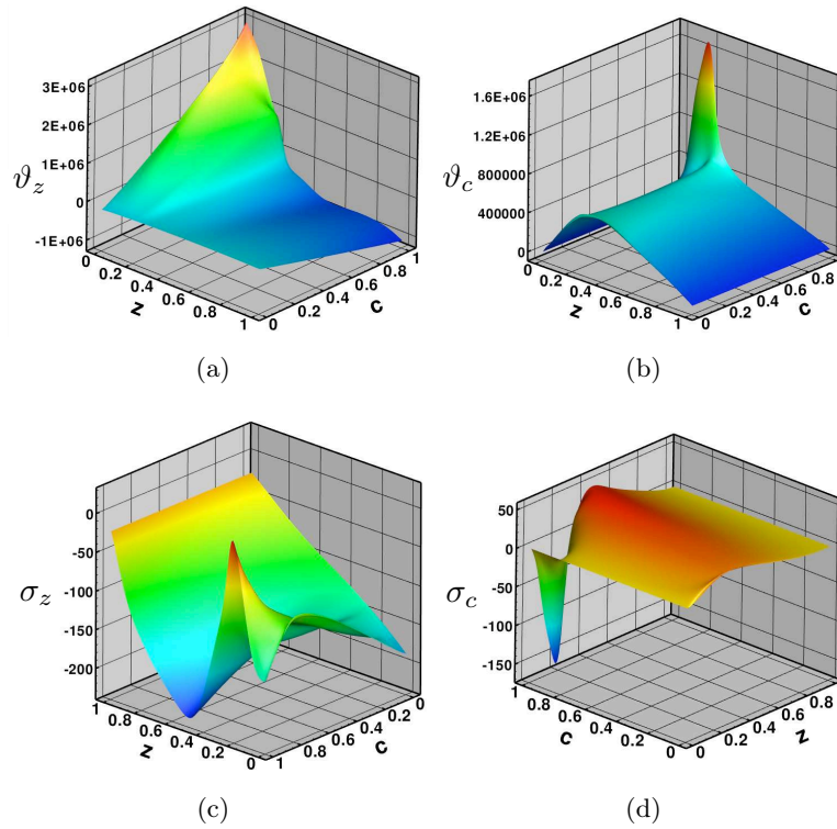
Figure 7.1: 3D view of the surfaces \vartheta_{\bar{z}}(\bar{z}, \bar{c}) (a), \vartheta_{\bar{c}}(\bar{z}, \bar{c}) (b), \sigma_{\bar{z}}(\bar{z}, \bar{c}) (c) and \sigma_{\bar{c}}(\bar{z}, \bar{c}) (d) with S_z = S_c = 0 and \chi_{st} = 20 \text{ s}^{-1} . The variables \vartheta_{\psi_i} are given in \text{J.kg}^{-1} and \sigma_{\psi_i} in \text{J.kg}^{-1}.\text{K}^{-1} . Beware of the change of axis orientation between subfigures.
