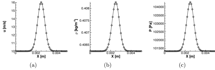
Figure 3.9: Initial solution created after adding an acoustic wave through the transformation matrix between conservative and characteristic variables. The gaussian wave amplitude A_2 is 0.01a_0 . Velocity (a), mass density (b) and pressure (c) are represented. Symbols: multi-component solution. Line: tabulated chemistry solution.
