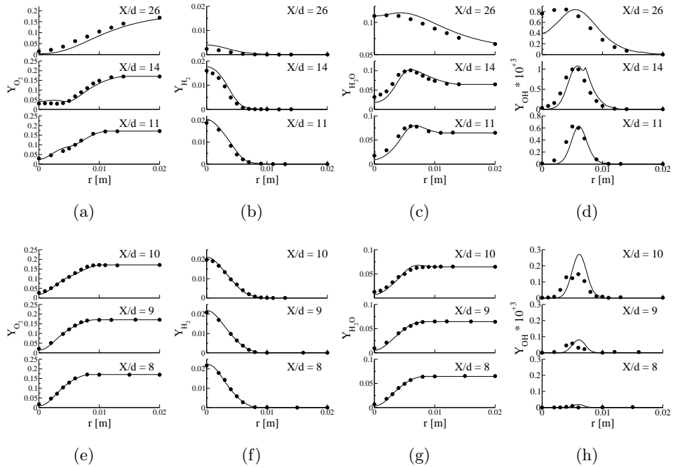
Figure 6.23: Profiles of Favre mean species mass fractions tabulated in the UTaC database (plain line) and measured (symbols). (a,e) Radial profiles of O_2 . (b,f) Radial profiles of H_2 . (c,g) Radial profiles of H_2O . (d,h) Radial profiles of OH .
