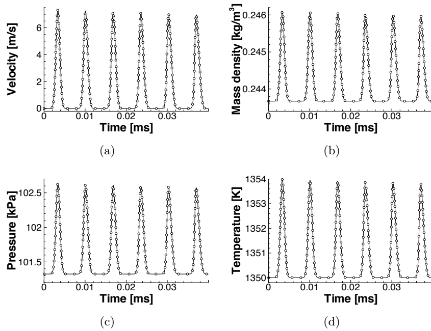
Figure 3.15: Variation in time at the probe ( x = 0 m) of velocity (a), mass density (b), pressure (c) and temperature (d). The initial gaussian profile is parametrized by A = 0.01a_0 , d = 5 \cdot 10^{-4} m and x_0 = 0.0025 m. Symbols: multi-component solution. Line: tabulated chemistry solution.
