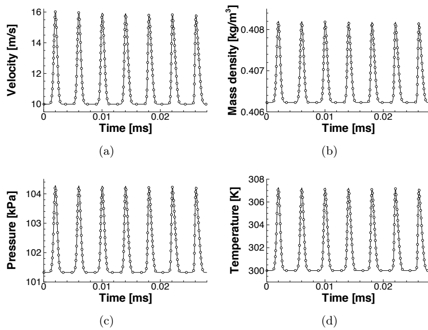
Figure 3.7: Time evolution of velocity (a), mass density (b), pressure (c) and temperature (d) at the point x = 0 m. Symbols: multi-component solution. Line: tabulated chemistry solution.
