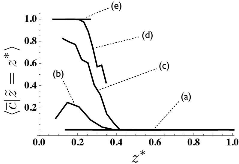
Figure 7.23: Profiles of the conditional mean \langle \bar{c} | \bar{z} = z^* \rangle at locations (a), (b), (c), (d), (e) defined in Fig. 7.22.
