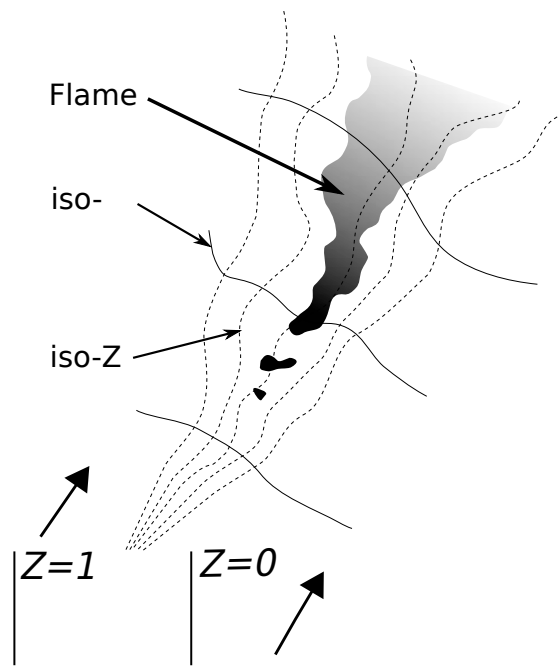
Figure 5.1: Schematic of auto-ignition in a partially non-premixed turbulent flow (left) and the corresponding non-premixed flamelets (right). Left: the flame (in grey) is stabilized between fuel ( z = 1 ) and oxidizer ( z = 0 ) streams ; isolines of lagrangian time (plain curves) and isolines of mixture fraction (dashed curves) are plotted. Right : temperature versus mixture fraction in a laminar non-premixed flamelet at three different times \tau = \tau_0, \tau_1, \tau_2 .
