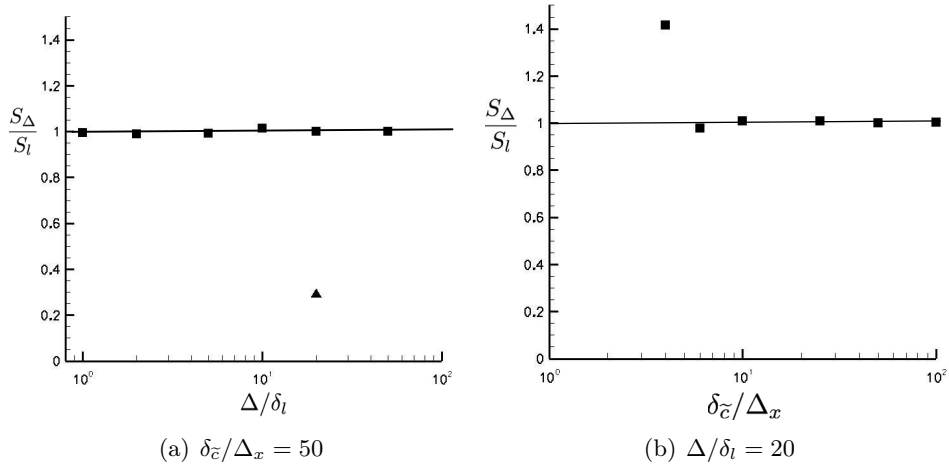
Figure 8.5: Predicted flame speed as a function of \Delta/\delta_l (left) and \delta_z/\Delta_x (right). Square symbols are the complete model solution and the triangle symbol is the solution with \alpha_\varphi = 1 .
