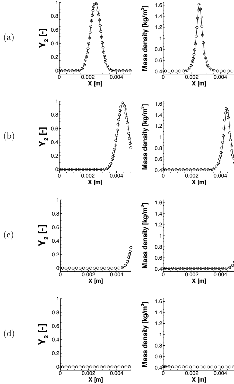
Figure 3.12: Composition wave passing through a reflective boundary. Mass fraction Y_2 (left) and mass density (right) profiles are plotted for multi-component (symbols) and TTC (line) formalism at different times t^+ = tL/u_0 in the simulation. (a) Initial solution, t^+ = 0 ; (b) t^+ = 0.4 ; (c) t^+ = 0.62 ; (d) t^+ = 0.85 .
