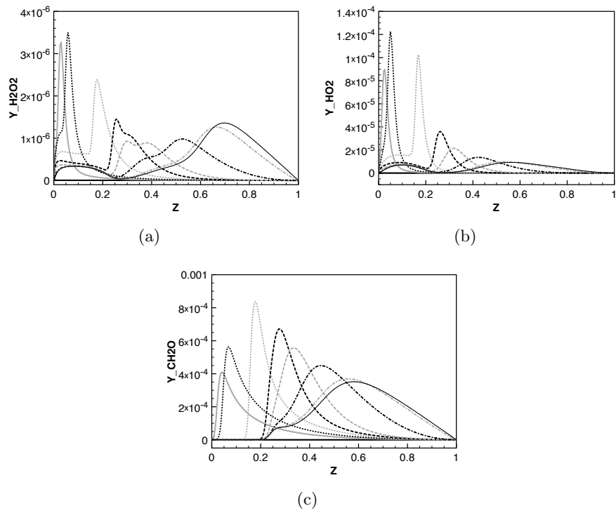
Figure 5.4: Unsteady mass fractions profile of precursor species in auto-ignition in mixture fraction space: (a) H_2O_2 (b) HO_2 (c) CH_2O . The flamelet was generated with \chi_{st} fixed to 30 \text{ s}^{-1} . The legend is the same as in Fig. 5.2.
