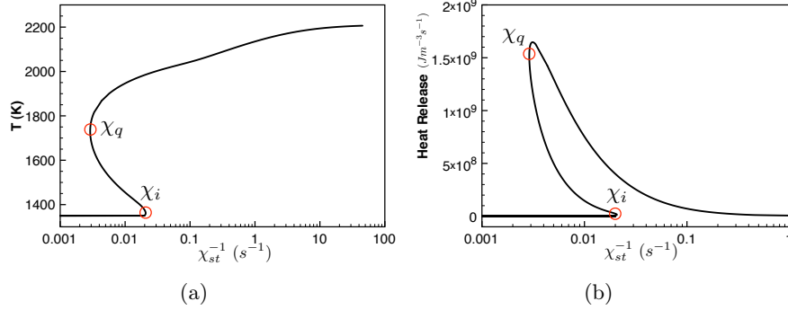
Figure 5.12: The maximum temperature (a) and the maximum heat release (b) of the steady solution flamelets is plotted in function of the inverse of the stoichiometric scalar dissipation rate. Two singular points are represented by circles: \chi_i the ignition scalar dissipation rate and \chi_q the quenching scalar dissipation rate.
