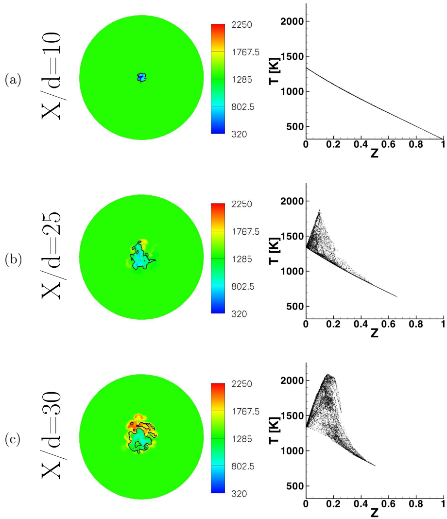
Figure 7.18: Instantaneous temperature color maps and scatter plots in mixture fraction space at different slice planes: (a) X/d = 10 ; (b) X/d = 25 ; (c) X/d = 30 ; (d) X/d = 35 ; (e) X/d = 40 ; (f) X/d = 60 . Black line: iso-line \tilde{z} = z_{st} = 0.175 .
