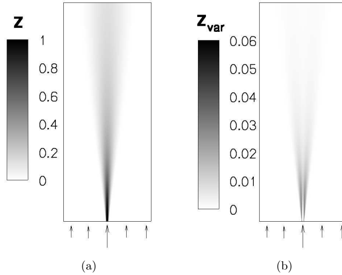
Figure 6.8: Planar contour of mean mixture fraction \bar{z} (a) and mixture fraction variance z_v = \tilde{z}''^2 (b).
