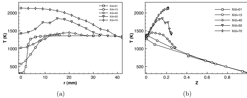
Figure 6.3: Radial profile of Favre averaged temperature for different position (a) and as function of mixture fraction (b) (Cabra et al., 2005).
