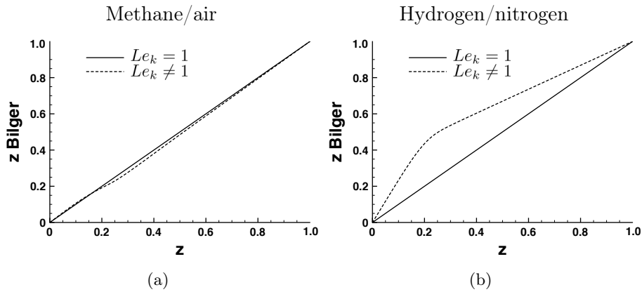
Figure 5.9: Mixture fraction defined by Bilger z_{\text{Bilger}} is plotted versus z in both Cabra flame configurations: methane/air (a) and hydrogen/nitrogen (b). Plain line: unity Lewis numbers. Dashed line: non-unity Lewis numbers.
