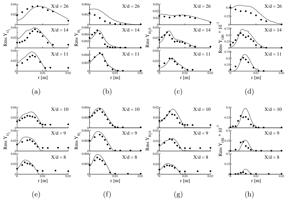
Figure 6.25: Profiles of species mass fractions RMS tabulated in the UTaC database (plain line) and measured (symbols). (a,e) Radial profiles of O_2 . (b,f) Radial profiles of H_2 . (c,g) Radial profiles of H_2O . (d,h) Radial profiles of OH .
