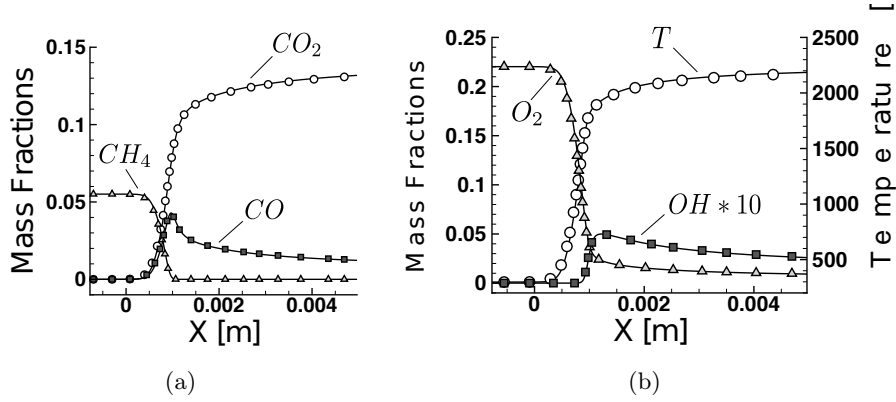
Figure 3.24: Mass fractions and temperature in a 1-D stoichiometric laminar premixed methane-air flame. Symbols: detailed chemistry solution. Line: TTC solution.
