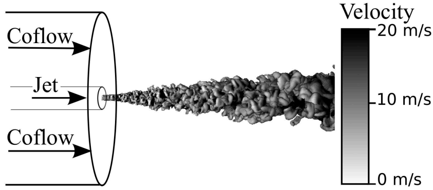
Figure 3.20: Mixture fraction isosurface z = 0.1 colored by longitudinal velocity.
