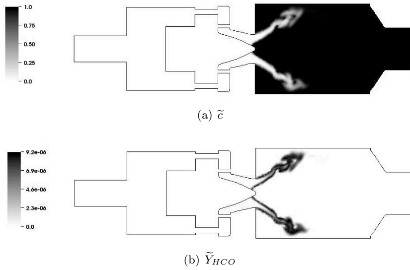
Figure 8.10: 2-D instantaneous view of \tilde{c} and \tilde{Y}_{HCO} .
