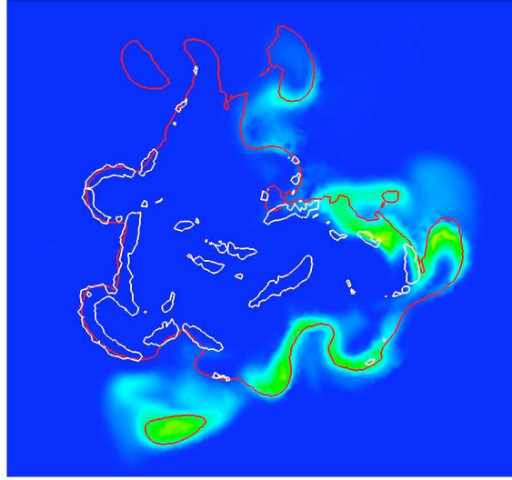
Figure 7.19: Plane at X/d = 25 colored by the source term \widetilde{\omega}_{\gamma_c} . White line: iso-line \tilde{\chi} = 25 \text{ s}^{-1} . Red line: iso-line \tilde{z} = 0.1 .
