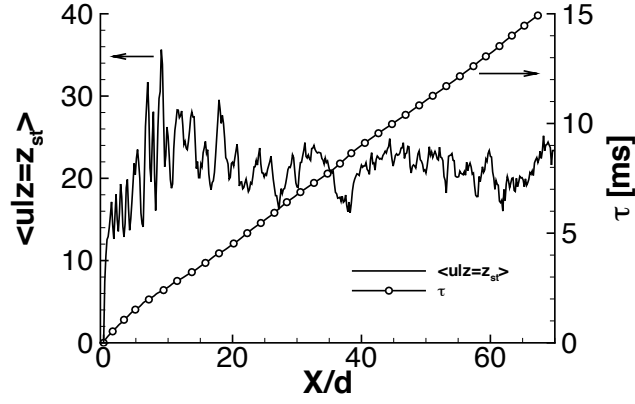
Figure 5.13: The conditional mean \langle \tilde{u}_{\tilde{z}} | \tilde{z} = z_{st} \rangle (plain line) and the flamelet Lagrangian time \tau (line + symbols) are plotted in function of the axial coordinate x/d where d the fuel pipe diameter.
