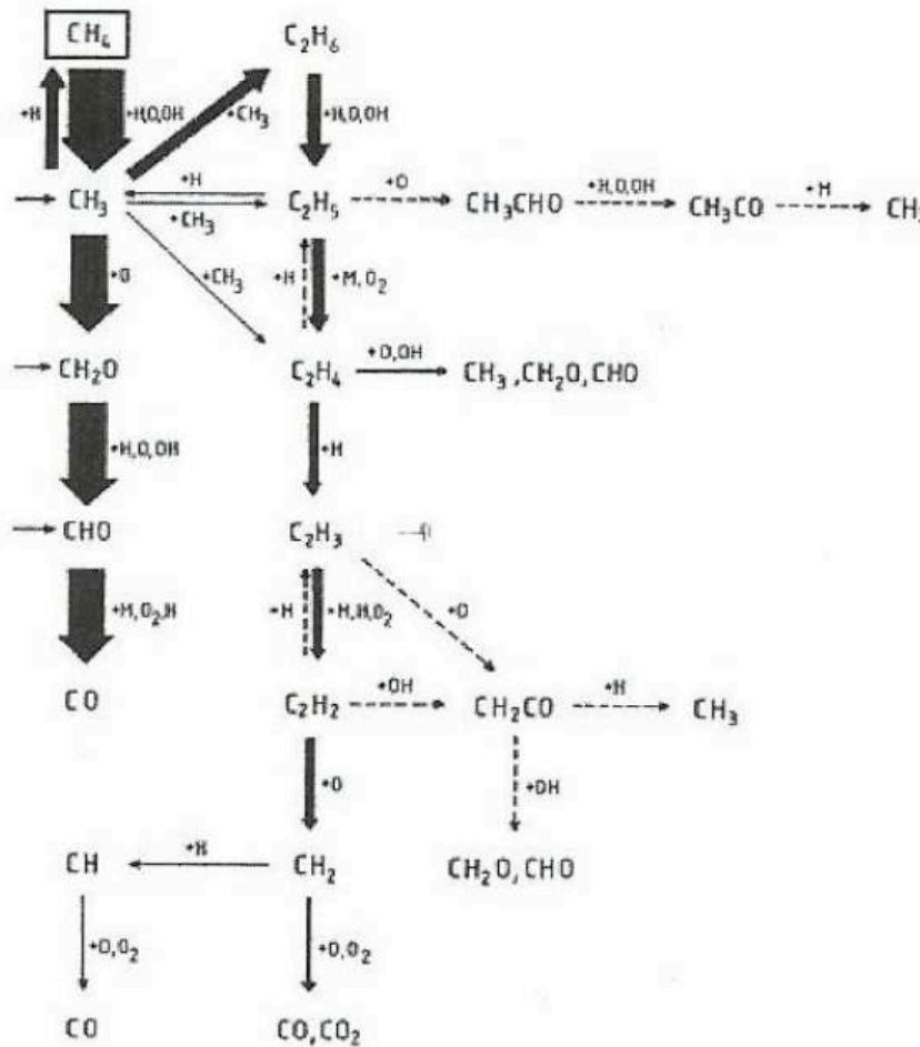
Figure 2.7: Integral reaction flow analysis in a premixed stoichiometric CH 4 -air flame with atmospheric pressure and a fresh gases temperature of 298K (Warnatz et al., 2006).
