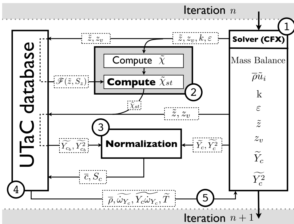
Figure 6.5: Scheme of the coupling between the UTaC database and the RANS solver between two iterations. Main steps are indicated by circled numbers.
