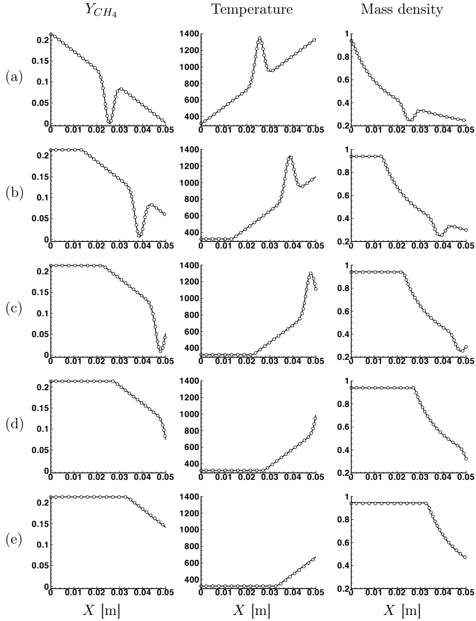
Figure 3.19: Composition wave passing through a reflective boundary. Methane mass fraction, temperature [K] and mass density [kg/m 3 ] profiles are plotted for multi-component (symbols) and TTC (line) formalism at different times t^+ = tL/u_0 in the simulation. (a) Initial solution, t^+ = 0 ; (b) t^+ = 0.27 ; (c) t^+ = 0.45 ; (d) t^+ = 0.54 ; (e) t^+ = 0.63 .
