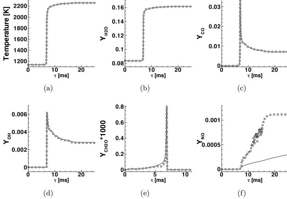
Figure 5.15: Time evolution at z = z_{st} of temperature (a) and species mass fractions: Y_{H_2O} (b), Y_{CO} (c), Y_{OH} (d), Y_{CH_2O} (e) and Y_{NO} (f). Plain line: reference solution computed with \chi_{st}(\tau) . Square symbols: solution interpolated in the database built for steady scalar dissipation rates.
