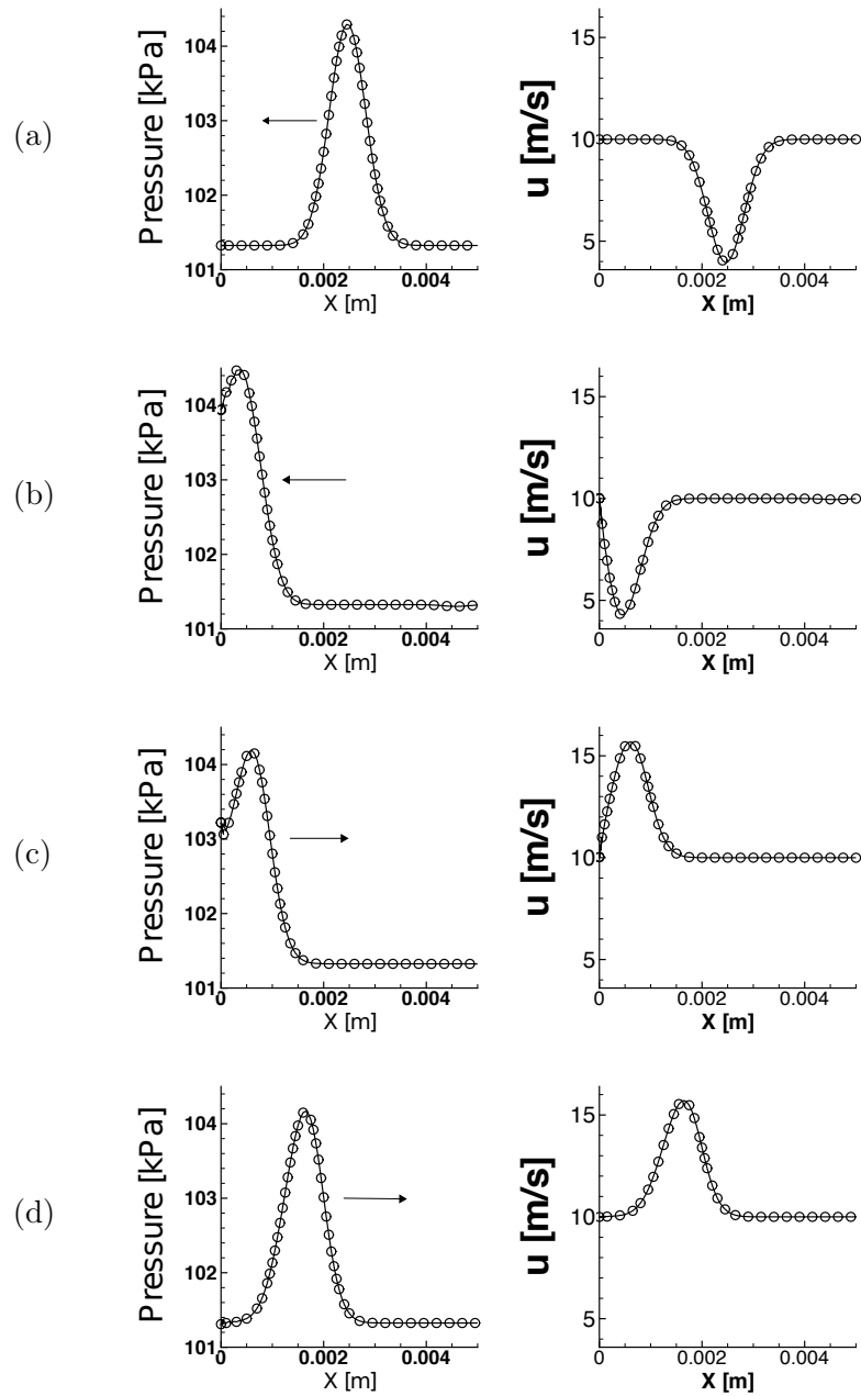
Figure 3.13: Acoustic wave reflected by an inlet boundary. Pressure (left) and velocity (right) profiles are plotted for multi-component (symbols) and TTC (line) formalism at different times t^+ = tL/a_0 in the simulation. (a) Initial solution, t^+ = 0 ; (b) t^+ = 0.41 ; (c) t^+ = 0.62 ; (d) t^+ = 0.82 .
