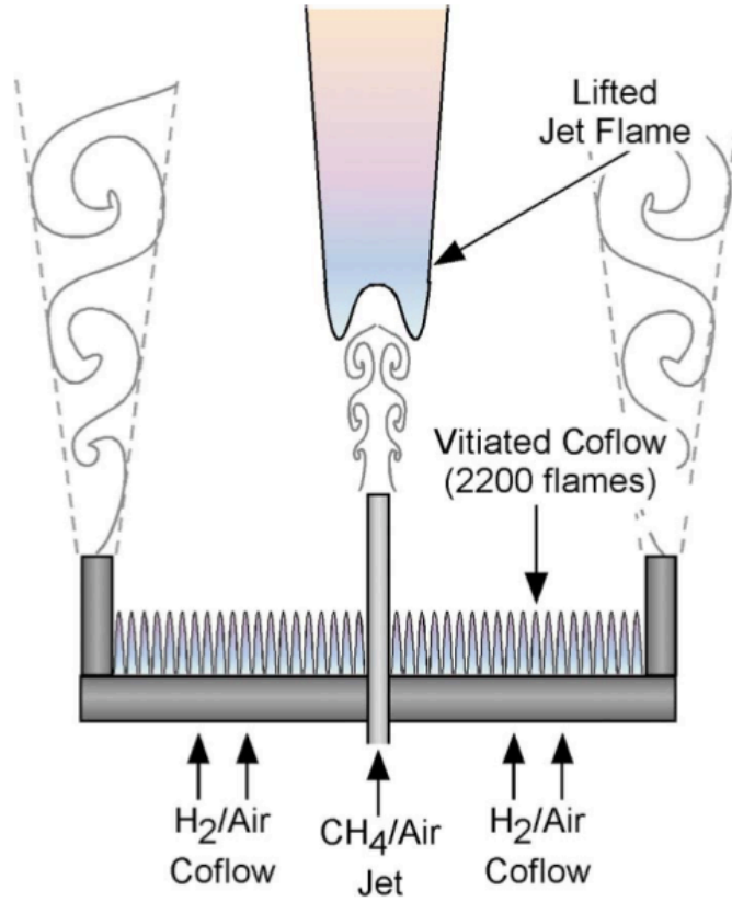
Figure 6.1: Lifted CH 4 /air jet into a coflow of hot products from a lean H 2 /air flame (Cabra et al., 2005).
