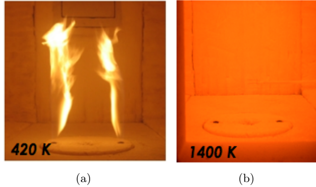
Figure 2: Photographs of a laboratory scale furnace (Rottier, 2010). Transition from a conventional flame (a) to the flameless combustion mode (b) as the furnace power and temperature increase. The nominal power is 18.6 kW.
