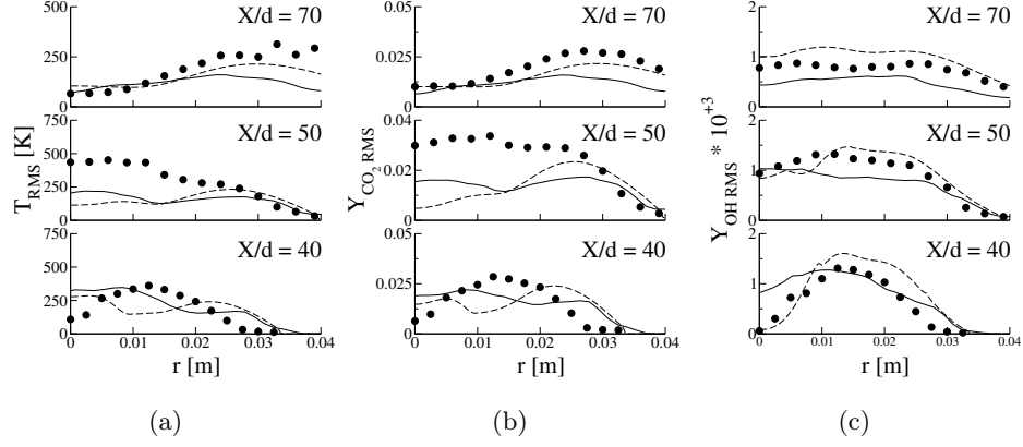
Figure 7.16: Radial profiles of temperature (a), \text{CO}_2 and \text{OH} mass fraction RMS in reactive LES (plain line) and RANS simulations (dashed line). Symbols: experimental data.
