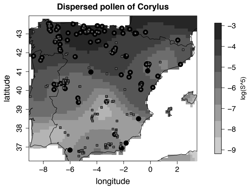
Figure 3.5: Posterior mean of the dispersed pollen of Corylus (Hazel tree, S^5 ) over Spain. Black dots show sites where Corylus pollen is present (i.e. in the data > 0\% ) and squares show sites where Corylus presence has been simulated by the vegetation model. The scale is logarithmic.
