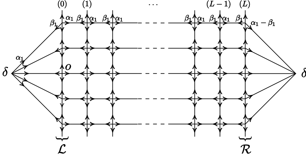
FIGURE 5.1. Definition of the weighted graph G . The top and bottom rows are identified (the graph is based on a cylinder) and the weights are the same on each line. Both vertices called \delta are the same.
