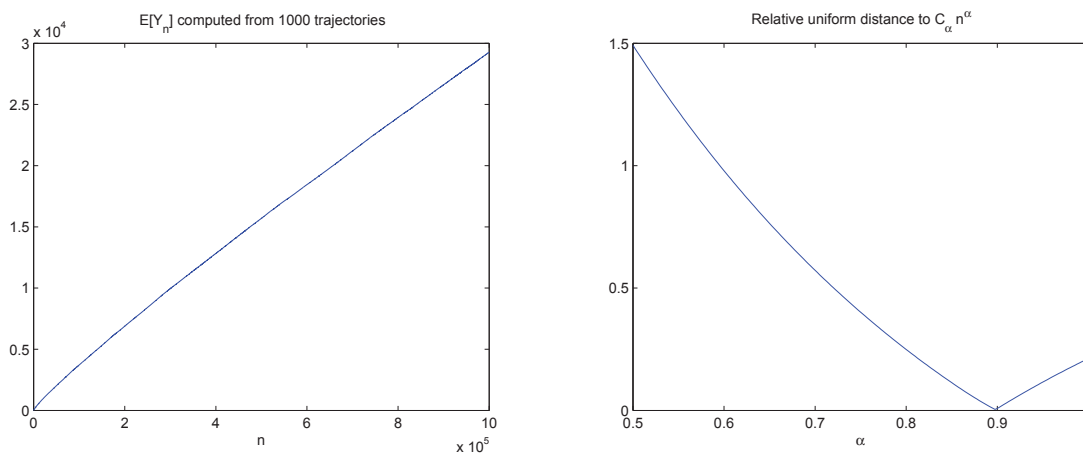
FIGURE 4.1. These plots refer to computer simulation: averages are taken over 10^3 trajectories up to time 10^6 (see section 4.5)
