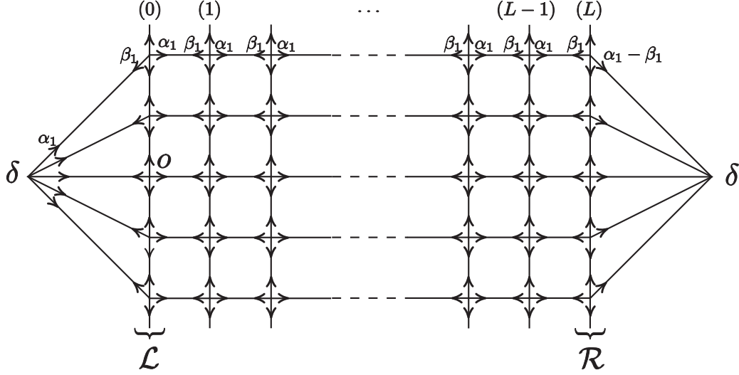
FIGURE 5.1. Definition of the weighted graph G . The top and bottom rows are identified (the graph is based on a cylinder) and the weights are the same on each line. Both vertices called \delta are the same.
