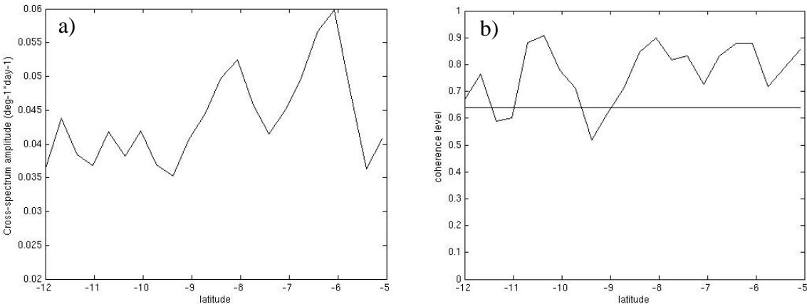
Fig. 6 - (a) Cross-spectral SSH-Chlorophyll amplitude peak (in \text{deg}^{-1} \cdot \text{day}^{-1} ) and (b) Coherence associated with the maximum amplitude of cross-spectrum SSH-Chlorophyll, vs latitude. The horizontal line indicates the threshold of significance level.
