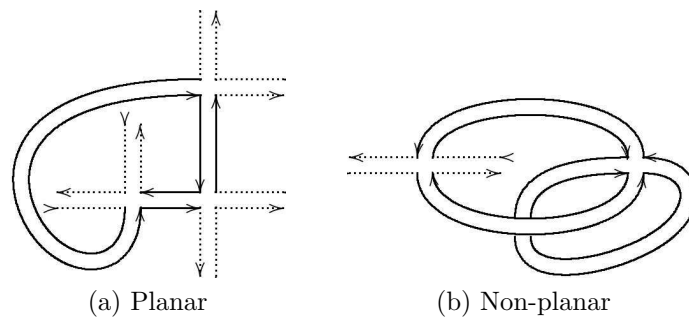
Figure 4.1: Ribbon graphs
