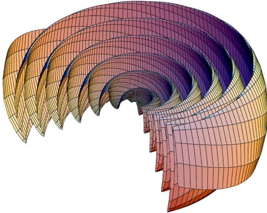
FIG. 49. The striped current sheet produced by an oblique rotator obtained with the split monopole model by Bogovalov (1999). Picture extracted from Kirk et al. (2009).
