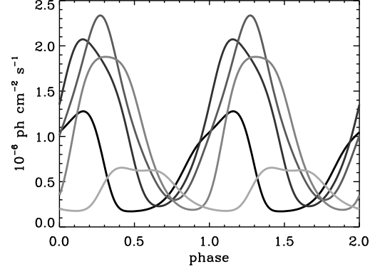
Figure 4. Impact of jet precession on the gamma-ray lightcurve for the best-fit model shown in Figure 2. The jet azimuth \theta_j is rotated in steps of 72^{\circ} from its best fit value of 319^{\circ} , with lighter lines as \theta_j moves away from this value.
