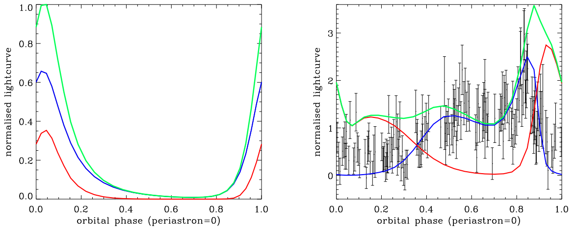
FIG. 69. Theoretical gamma-ray lightcurves in LS 5039, in the Fermi energy range (flux > 1 GeV left panel) and HESS energy range (flux > 100 GeV, right panel). HESS data points are taken from Aharonian et al. (2006). The 1D cascade component (red line) is compared with the primary absorbed contribution (blue line). The sum of both component is shown by the green line.
