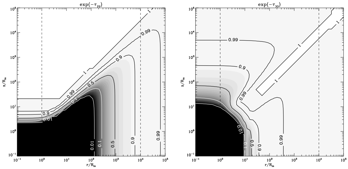
FIG. 112. Same as in Fig. 111 in the (r, z) plane for a viewing angle \psi = 0^\circ (left panel) and \psi = 45^\circ (right panel). The black dashed lines indicate r = R_{in} and r = R_{ext} .
