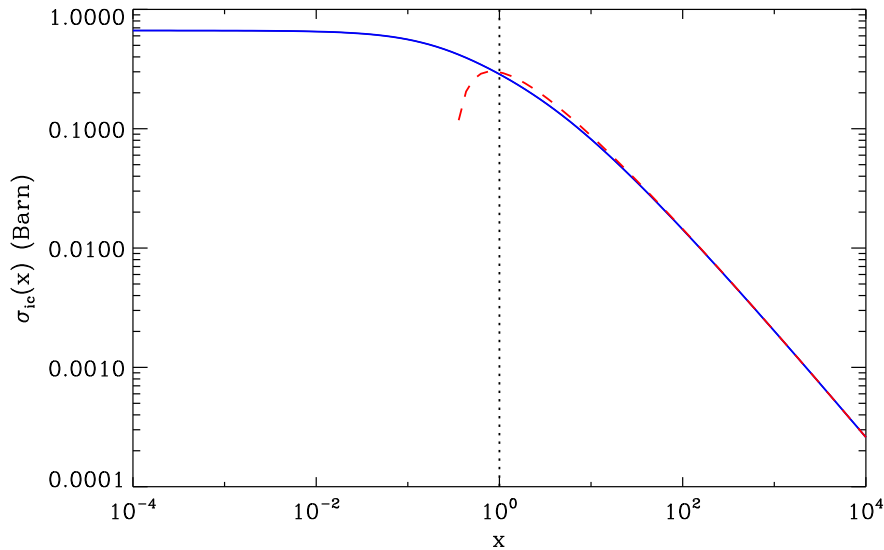
FIG. 4. Total cross section for inverse Compton scattering as a function of x = \epsilon'_0 / m_e c^2 . The dashed line separates the Thomson ( x \ll 1 ) to the Klein-Nishina regime ( x \gg 1 ). The approximate formula given in Eq. (5.3) is shown with a red dashed line.
