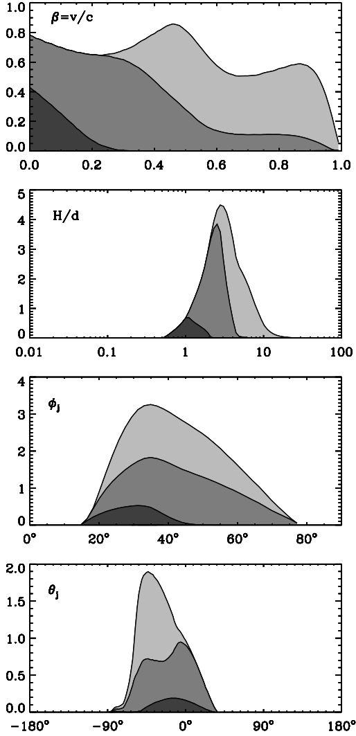
Figure 3. Distribution of jet parameters for models in the 90% confidence region given by \chi^2 statistics. Orbit O1 ( 20 M_{\odot} black hole, i=30^{\circ} ) is assumed. The various regions correspond to a power in high energy electrons P_e \leq L_{\text{Edd}} (light grey), \leq 0.1L_{\text{Edd}} (grey), \leq 0.01L_{\text{Edd}} (dark grey). Here, L_{\text{Edd}} is 2 \cdot 10^{39} \text{ erg s}^{-1} .
