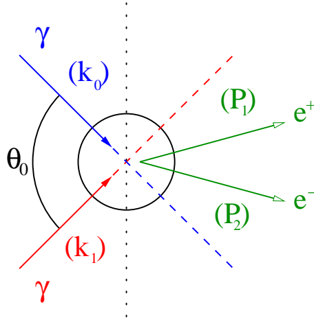
FIG. 50. Kinematics for pair production. The photons annihilate and produce a pair electron-positron if the total energy available in the center-of-mass frame is greater than the rest mass energy of the pair.
