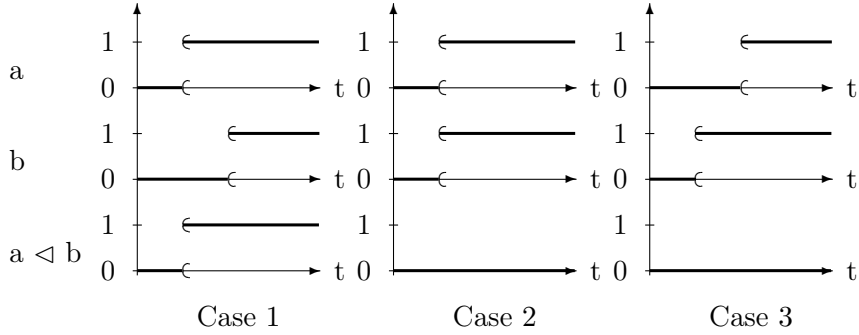
Figure 3.5: Timing diagrams of operator non-inclusive BEFORE (BF)
