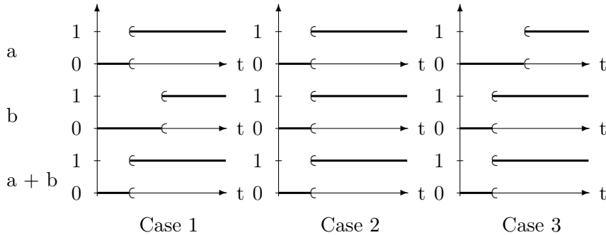
Figure 3.3: Timing diagrams of Boolean operator OR
