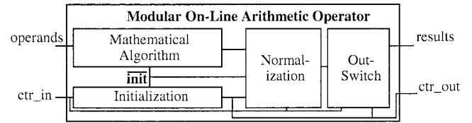
Fig. 3. Modular on-line arithmetic operator.
