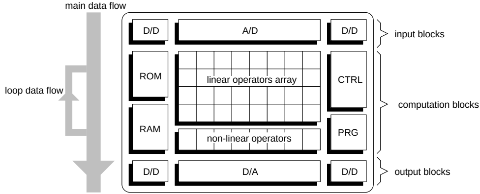
FIGURE 2.2.: Architecture de FPOP.
