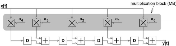
Fig. 6. The transposed form of an FIR filter.
