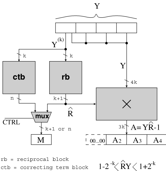
Fig. 2. Organization of the reduction module. M depends on the function being computed.
