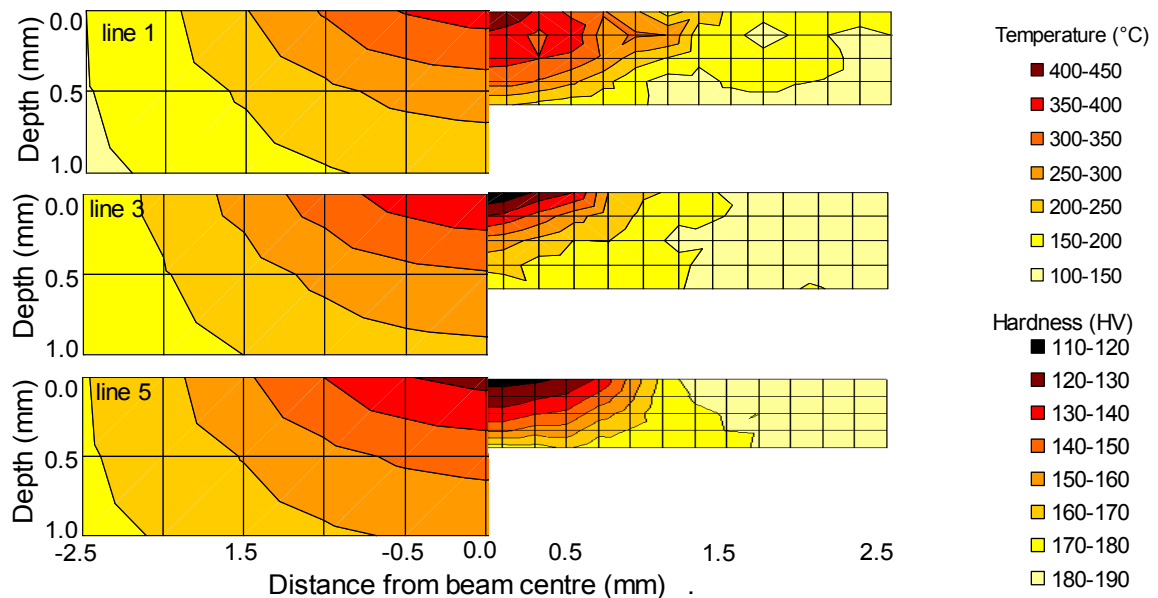
Fig. IV.23. Superimposition of temperature and hardness maps
