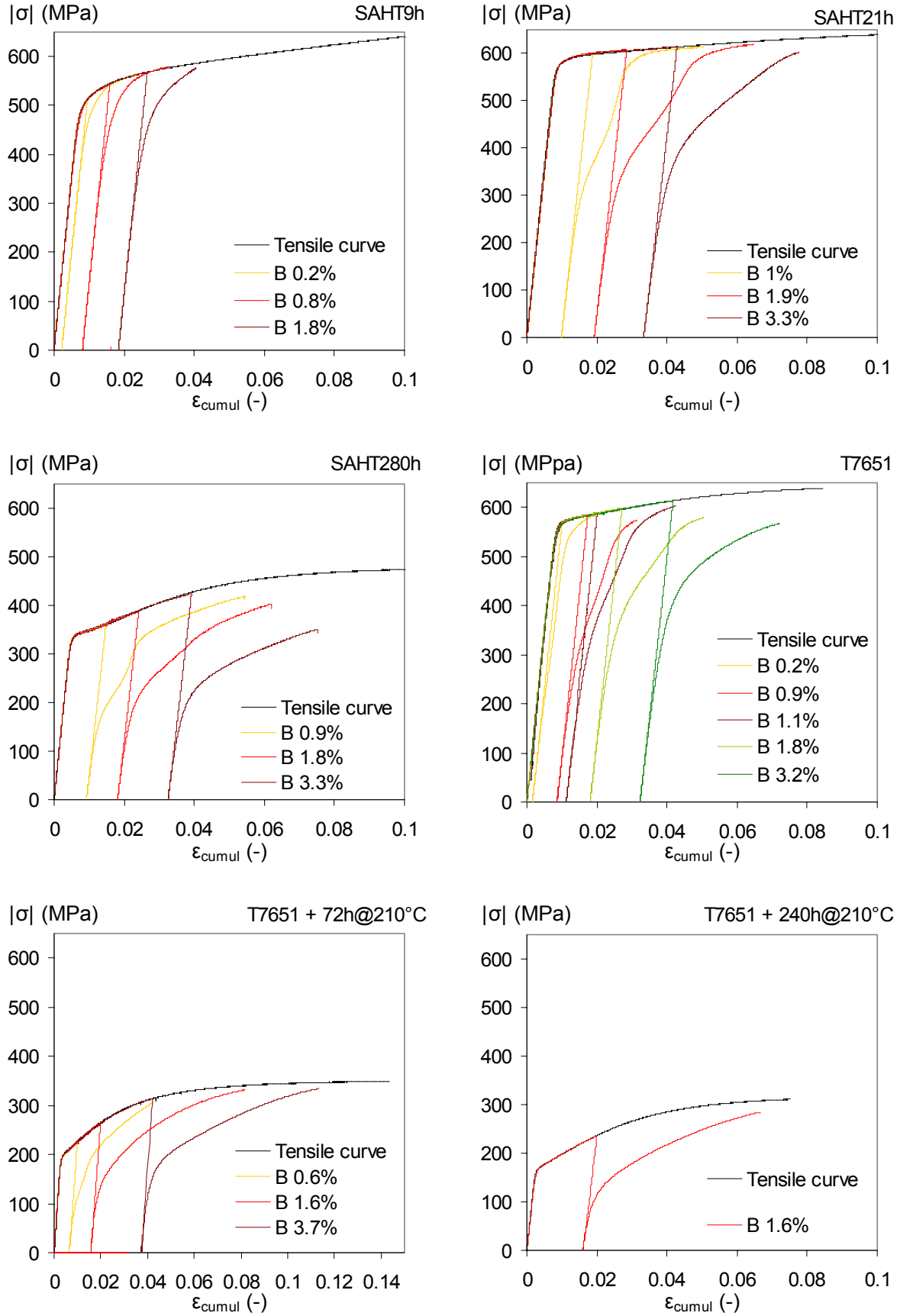
Fig. III.28. Bauschinger curves for various tempers
