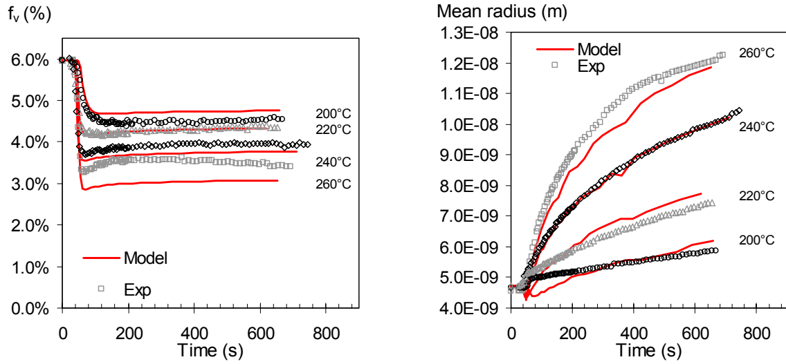
Fig. IV.30. Precipitation kinetics modelling during reversion at various temperatures
