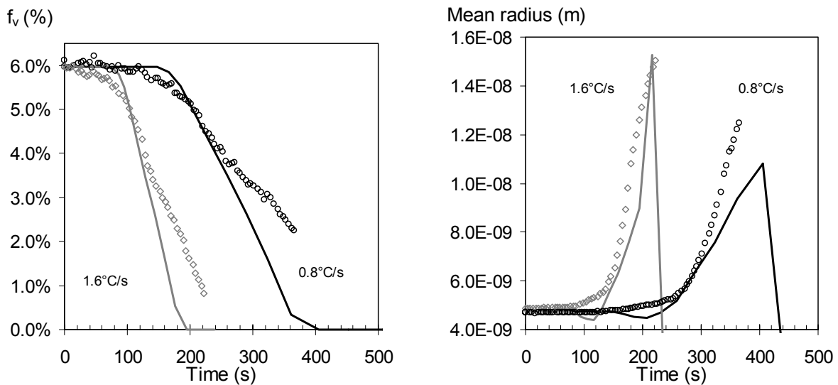
Fig. IV.31. Precipitation kinetics modelling during heating ramps
