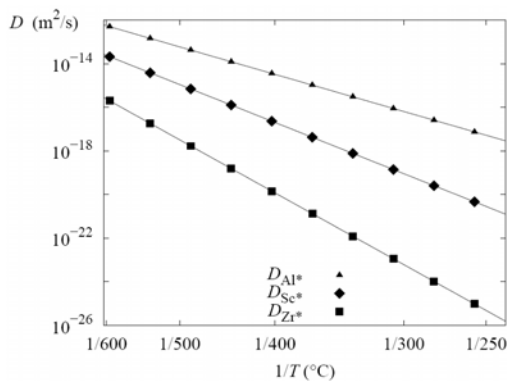
Fig. I.19. Diffusion coefficients of Al, Sc and Zr in Al
