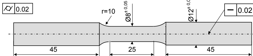
Fig. II.12. Drawing of the Bauschinger specimen #1
