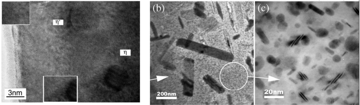
Fig. I.15. \eta' and \eta precipitates
