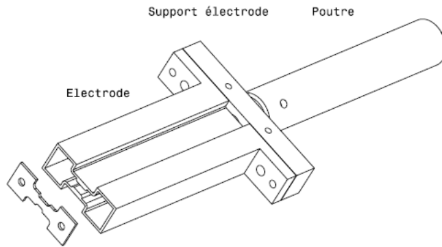
Fig. II.28. TSAXS specimen electrode
