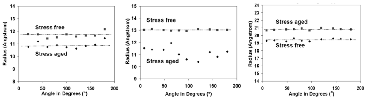
Fig. V.11. Effect of stress aging on the precipitate radius of AA7475
