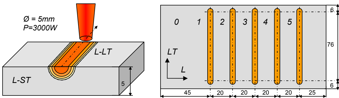
Fig. IV.8. Specimen and laser processing
