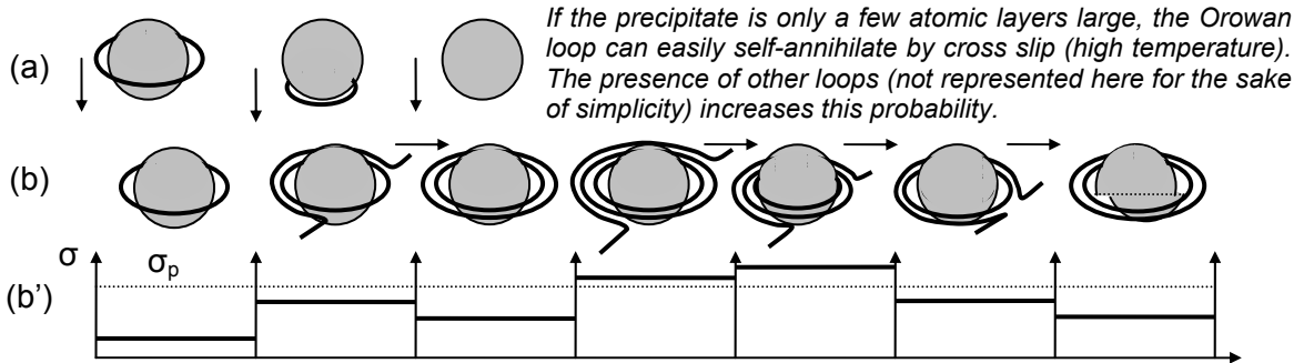
Fig. III.51. Self-annihilation mechanisms
