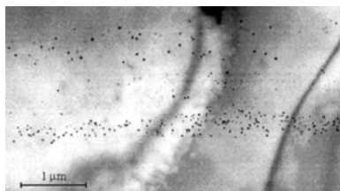
Fig. I.20. Dispersoids bands
