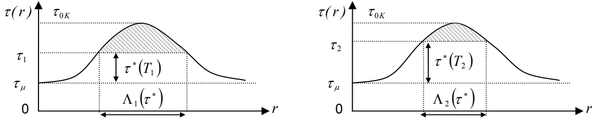
Fig. III.45. Thermal activation of obstacle bypassing
