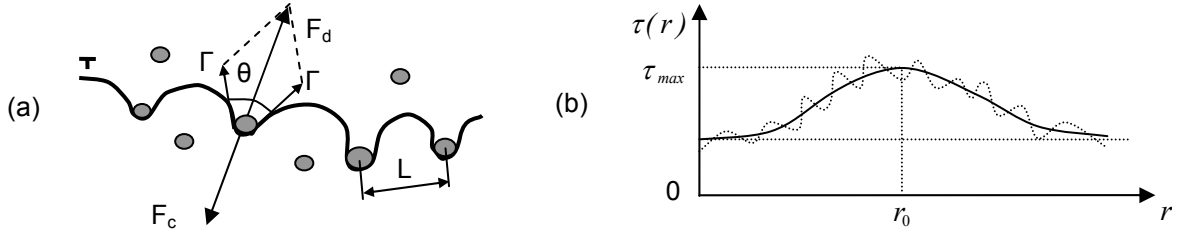
Fig. I.26. Schematic of the obstacle force
