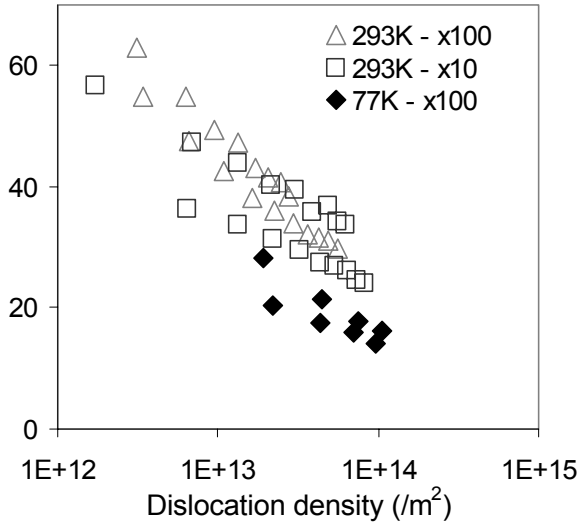
Fig. III.42. Activation volume of T7651
