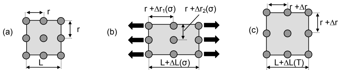
Fig. I.22. Schematic of the effect of temperature and elastic stress on inter-atomic distance
