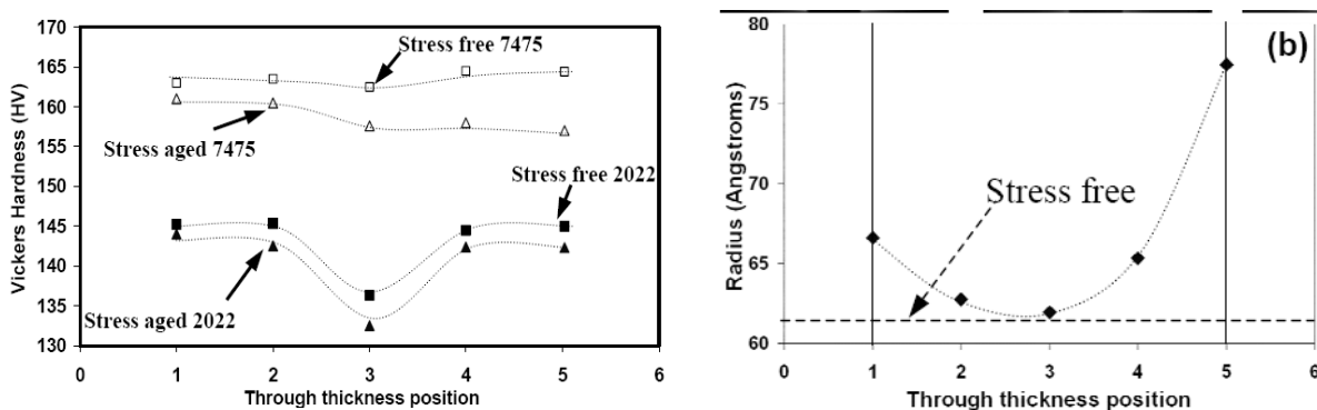
Fig. V.1. Through thickness properties of two aluminium alloys after industrial CAF
