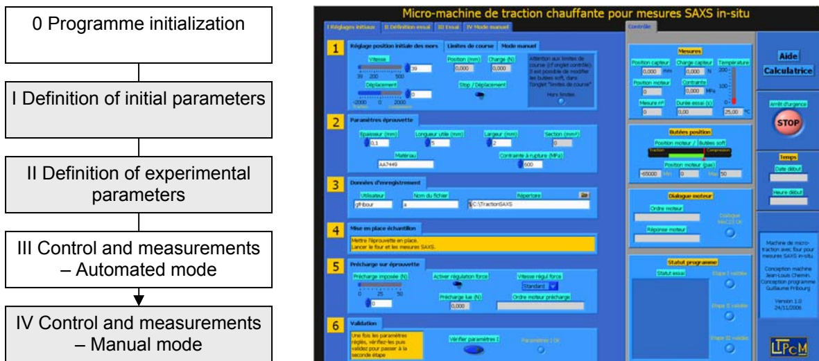
Fig. II.30. TSAXS programme
