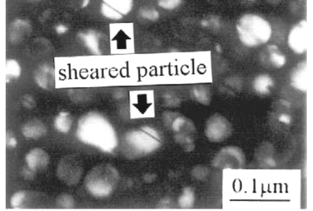
Fig. I.30. Sheared precipitates
