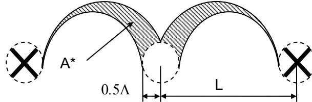
Fig. III.41. Definition of the activation volume
