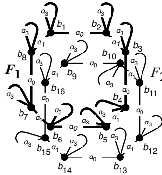
FIGURE 1.23 – Deux 2-cellules
