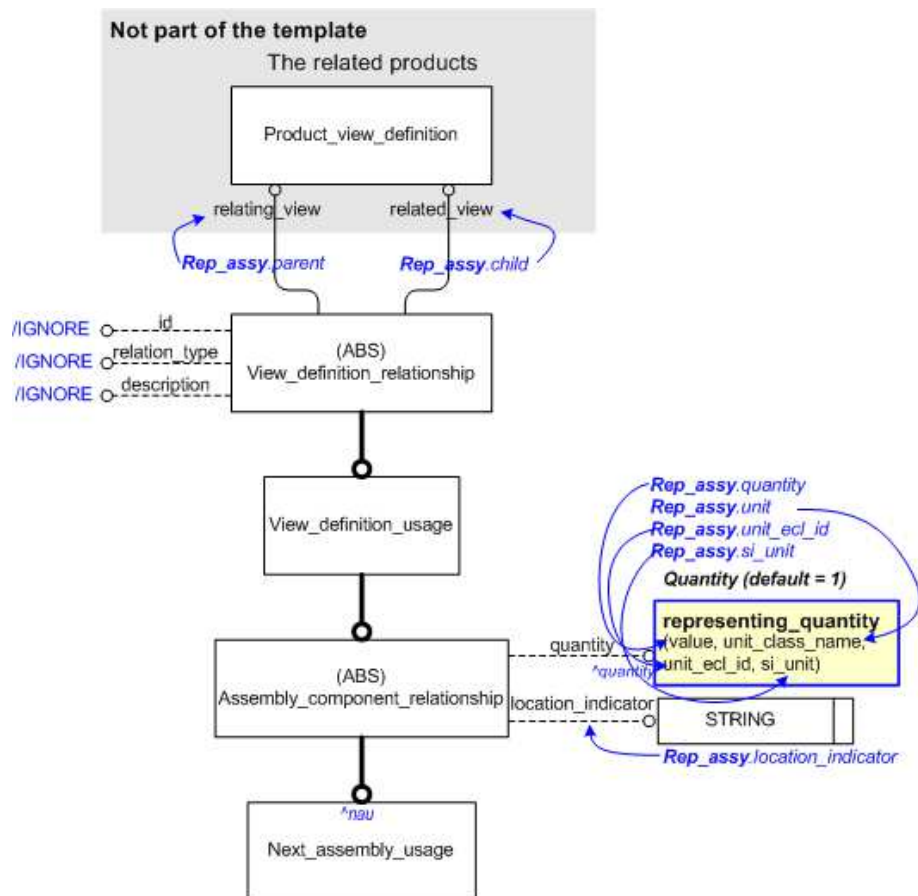
FIGURE 3.3.6.: Modèle EXPRESS-G representing_assembly_structure
