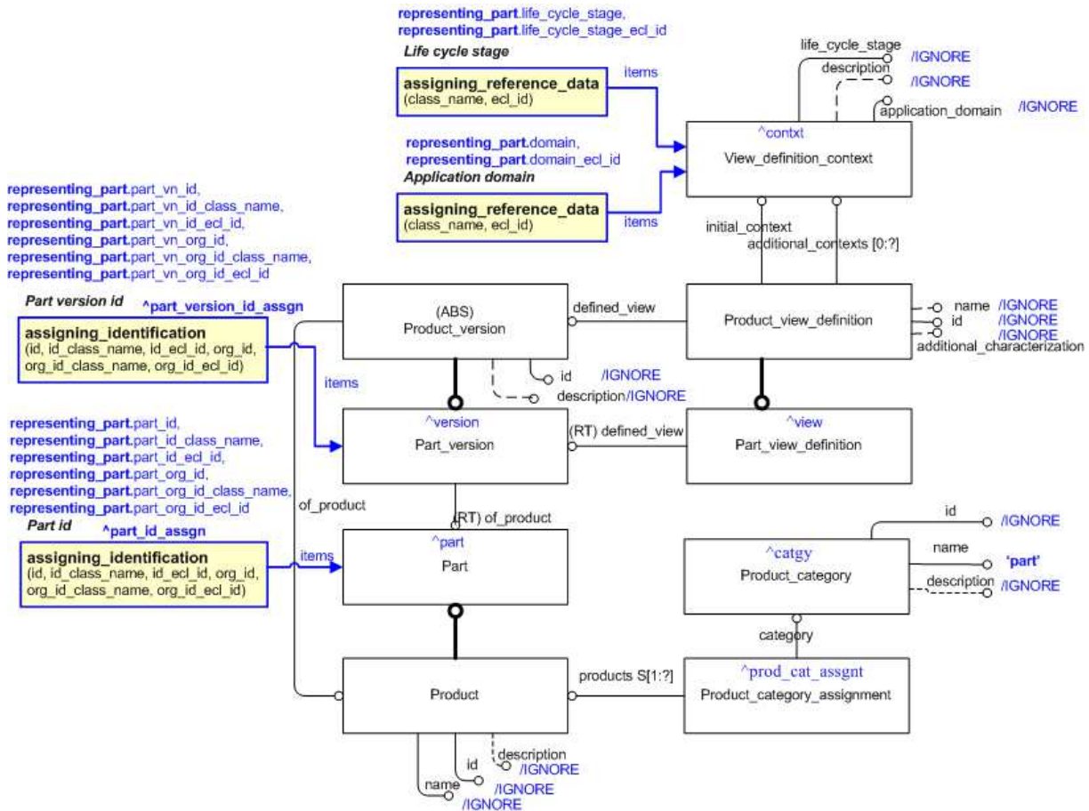
FIGURE 3.3.5.: Modèle EXPRESS-G representing_part
