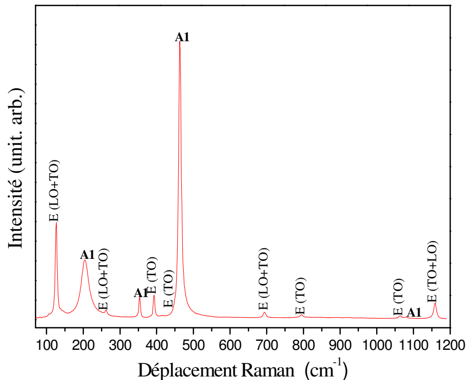
Figure V.1. Spectre Raman du quartz- \alpha
