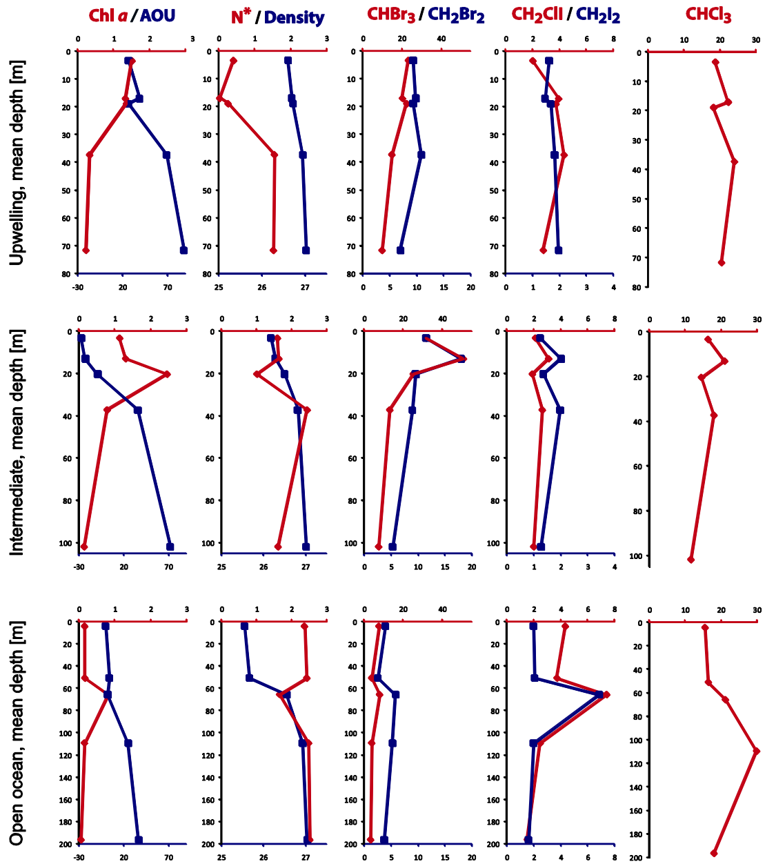
Figure 6 Depth profiles of chlorophyll \alpha [ \mu\text{g L}^{-1} ], AOU [ \mu\text{mol L}^{-1} ], \text{N}^* [ \mu\text{mol L}^{-1} ], density [ \sigma ] and selected VHOC [ \text{pmol L}^{-1} ] in the three defined water masses at five depth.
