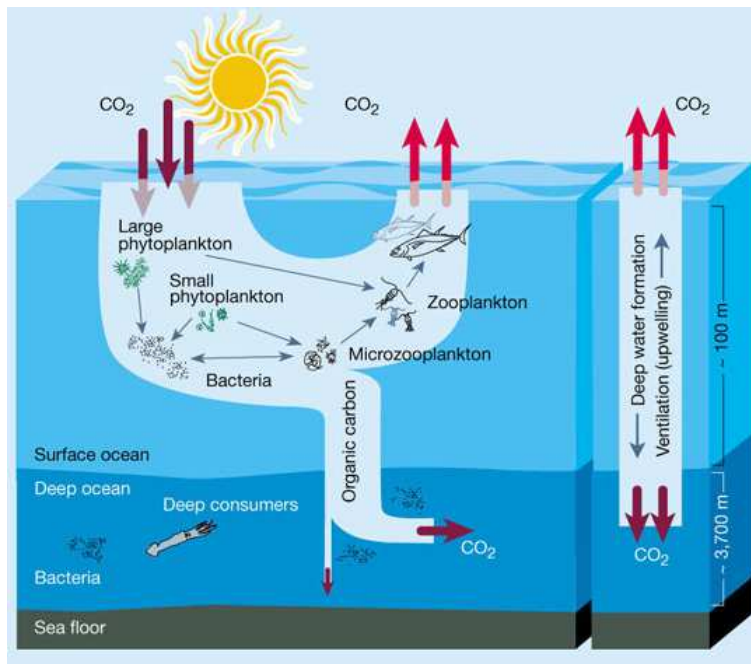
Figure 1.1: Schematic representation of the two oceanic carbon pumps: on the right hand side, the "solubility pump", which is driven by chemical and physical processes ; on the left hand side, the "biological pump" where planktonic ecosystems in the upper ocean play a key role (From Chisholm [2000]).
