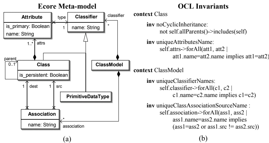
Figure 4.2: (a) Simple UML Ecore Meta-model (b) OCL constraints on the Ecore meta-model
