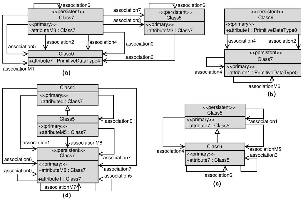
Figure 3.20: (a) Model conforming to Meta-model (b) Model conforming to Meta-model + Pre-condition (c) Model conforming to Meta-model + Pre-condition + Test Model Objective (d) Model conforming to Meta-model + Pre-condition + Model Fragment
