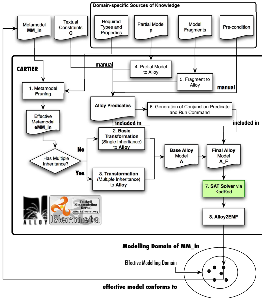
Figure 3.2: PRAMANA Architecture
