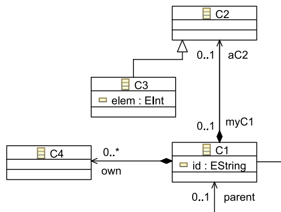
Figure 2.10: Metamodel M' .
