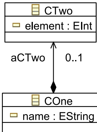
Figure 2.9: Metamodel M .
