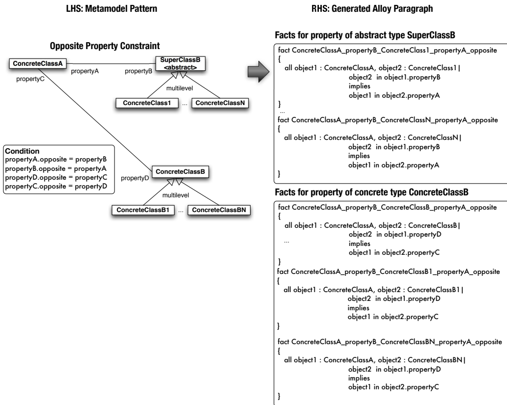
Figure 3.17: Transforming Opposite Properties to ALLOY Facts in Metamodel with Multiple Inheritance
