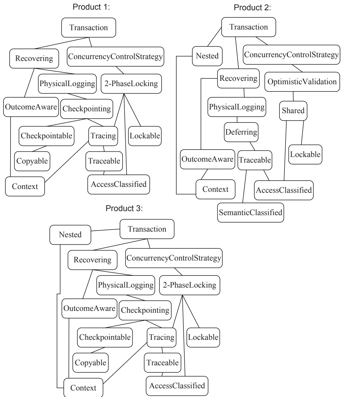
Figure 2.8: Three Products from the AspectOPTIMA feature diagram
