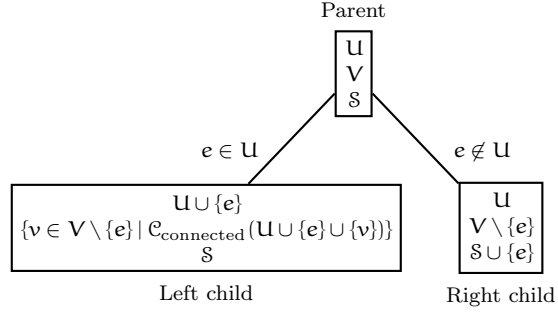
Figure 14: Enumeration of any element e \in V . \mathcal{C}_{\text{connected}} removes elements from V . \mathcal{C}_{\text{closed}} is checked on U \sqcup V extended with every element in S .
