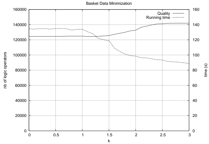
Figure 26: Time to minimize, under \mathcal{C}_k -summary, a QUEST-generated dataset.
