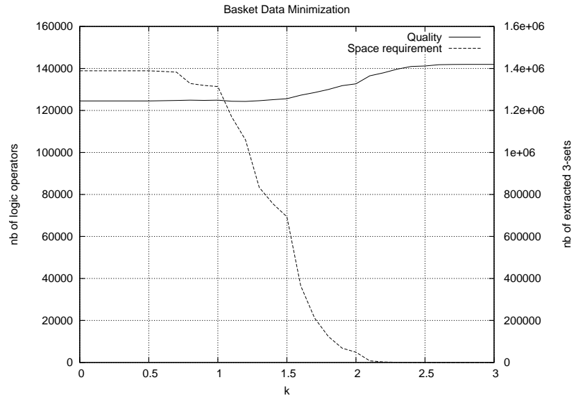
Figure 27: Space to minimize, under \mathcal{C}_k -summary, a QUEST-generated dataset.
