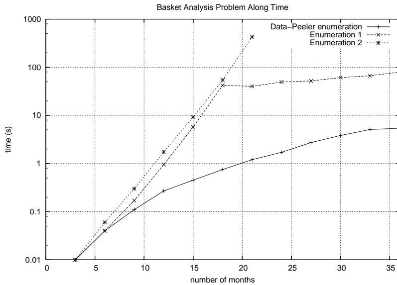
Figure 23: Comparing sensible enumeration strategies.
