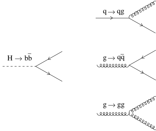
Figure 2.10: Higgs signal vs QCD backgrounds
