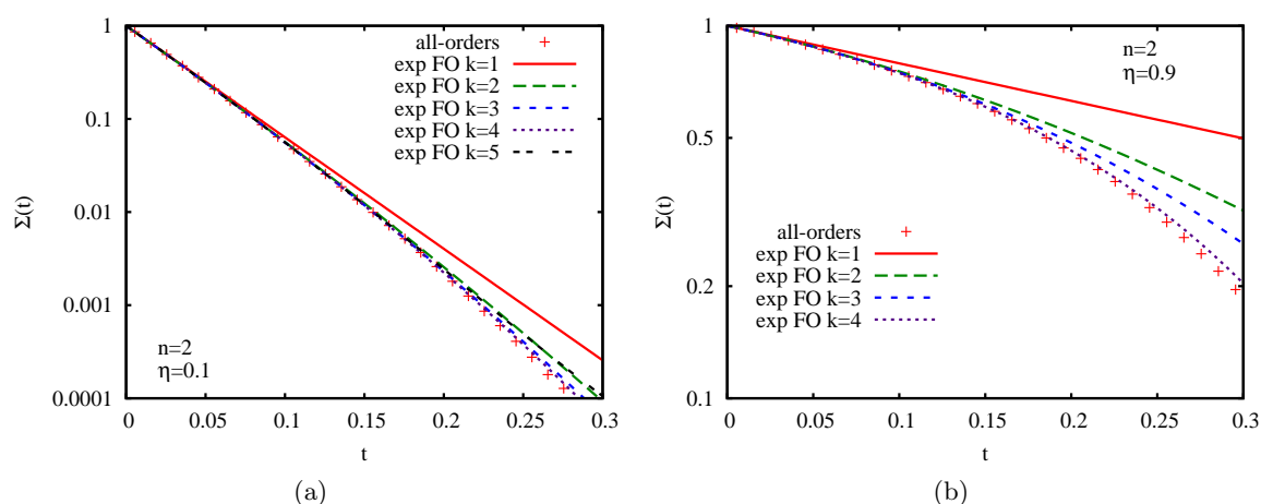
Figure E.3: Comparison between exponentiated fixed-order (exp FO) expansion and all-orders result when n = 2 for (a) \eta = 0.1 and (b) \eta = 0.9 .
