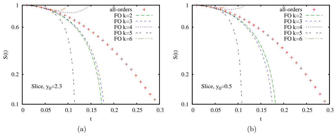
Figure E.7: Comparison between all-orders and fixed-order results for the purely non-global part S(t) of the Slice when (a) y_0 = 2.3 and (b) y_0 = 0.5 .
