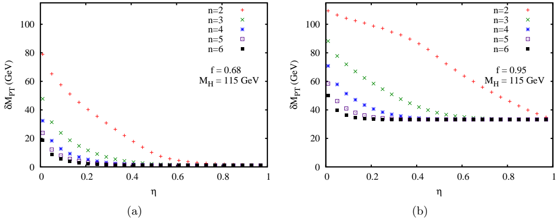
Figure 4.6: Perturbative width of the Higgs boson (in GeV) as a function of \eta for several values of n when (a) f = 0.68 and (b) f = 0.95 .
