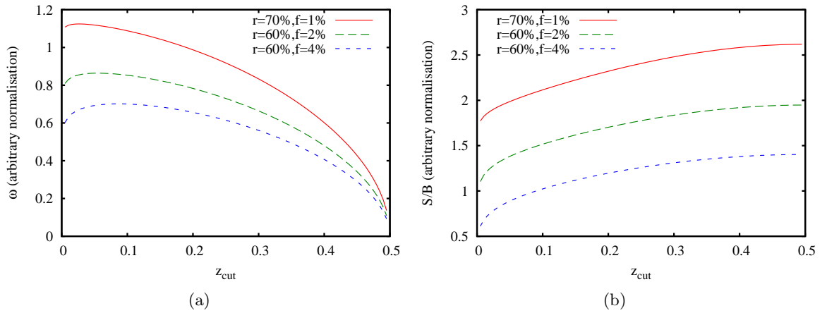
Figure 2.12: (a) The significance of the signal as a function of z_{cut} for 3 different values of the couple (r, f) ; (b) \frac{S}{B} as a function of z_{cut} for the same values of (r, f) .
