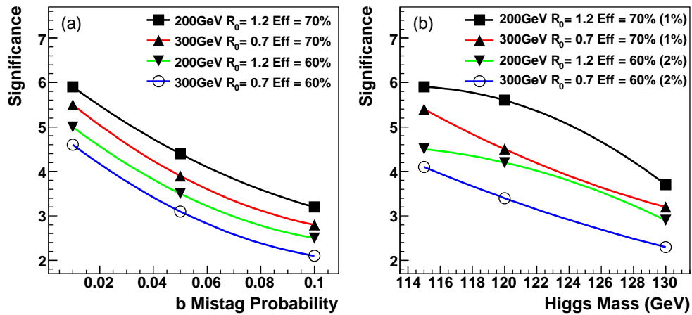
Figure 3.11: (a) Expected significance as a function of the mistag rate for different b -tag efficiencies and p_{t,min} (shown at optimal R_0 values). (b) Expected significance as a function of the Higgs mass.
