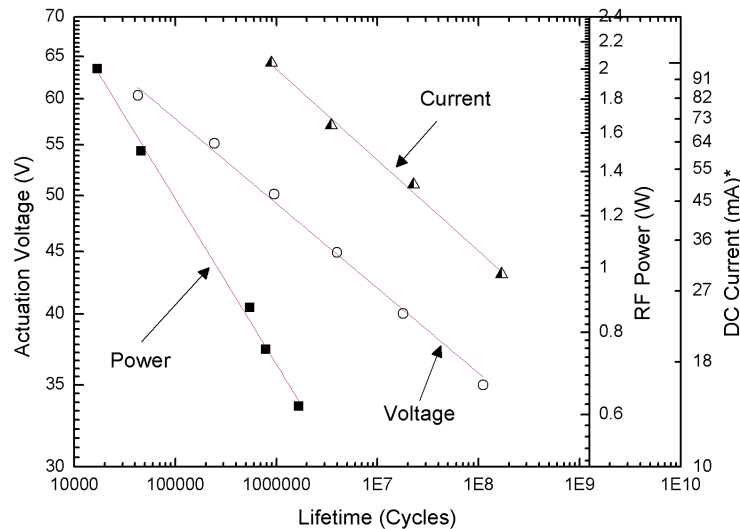
FIGURE 2.12: Operating parameters vs. device's operation time.
