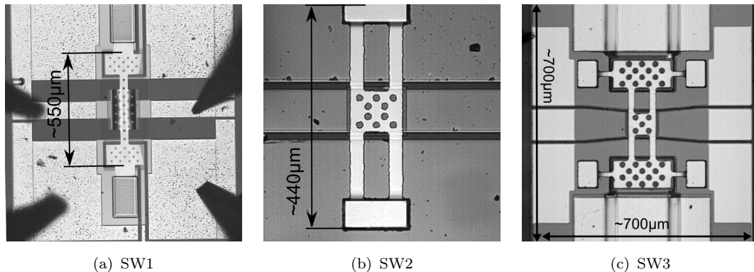
FIGURE 3.13: Tested devices.
