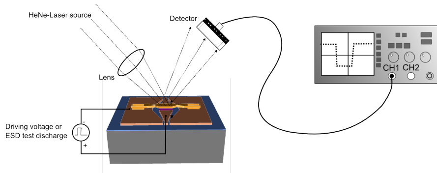
FIGURE 3.16: Simple experimental apparatus employed here to measure mechanical variation of the movable membrane.
