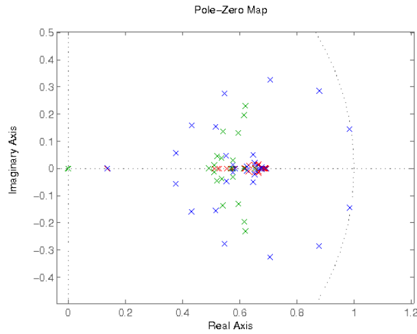
Figure 4-6: Closed-loop time-evolution by considering the full-order observer-based output feedback controller.
