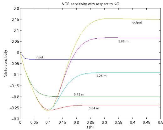
(e) Sensitivity of NO_2 with respect to K_C .
