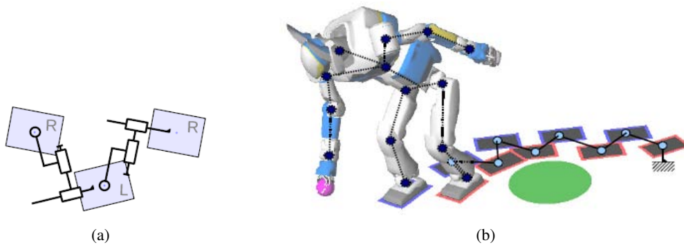
Figure 2.17: (a) Virtual kinematic chain. (b) The kinematic model of the robot plus virtual kinematic chain. Cited from [Kanoun et al. 2009]
