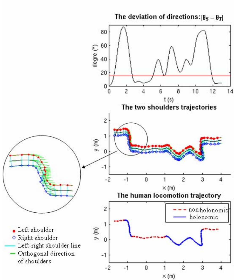
Figure 4.5: A demonstration of the segmentation function during a hybrid movement
