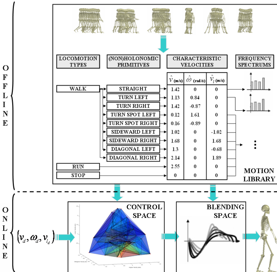
Figure 6.1: Architecture of the locomotion controller.
