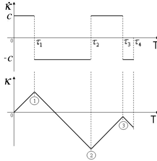
Figure 3.5: The concatenation point between two clothoid arcs is called a “switching point”. At each switching point the curvature function contains a local extremum and the derivative of the curvature has a discontinuity.
