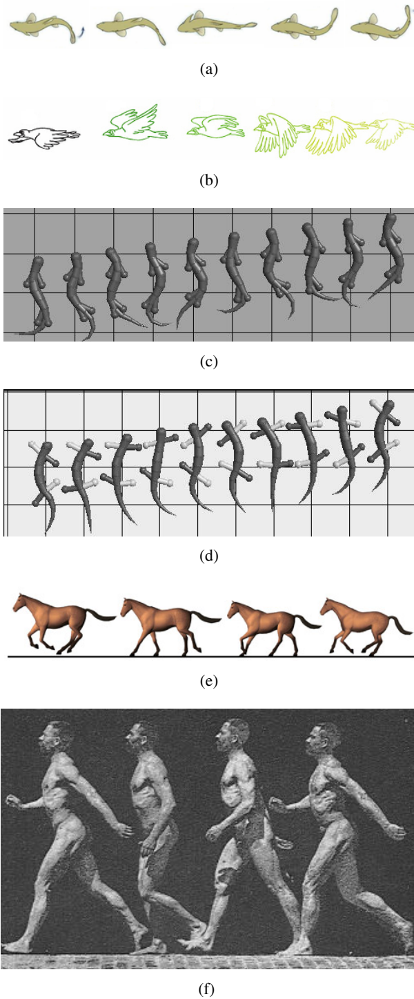
Figure 2.1: Vertebrate locomotions in instantaneous frames of fish (a) (from Michigan Science Art), bird (b) ( www.flickr.com ), horse (e) (from Visual Dictionary Online), and human (f) (borrowed from Etienne-Jules Marey in Le mouvement , 1894). Salamanders can perform two different types of locomotions corresponding to two different mechanisms (swimming (c) and stepping (d) [Ijspeert 1995]).
