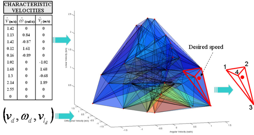
Figure 6.13: Tetrahedron selection process from an input (desired speed). The red tetrahedron is selected from the tetrahedra data structure in the control space.
