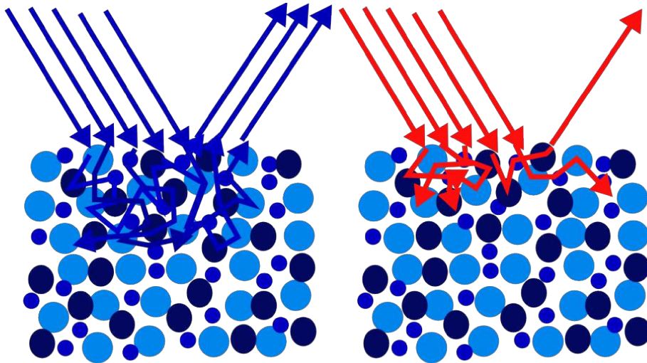
Figure 3.2: For this blue surface, more blue light is reflected than red light. Different colors, and thus different wavelengths, probe different depths of the surface. (This figure is modified from a similar figure by W. Grundy)
