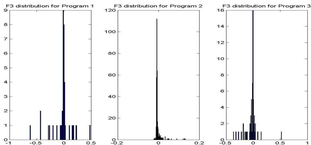
Figure A.4: Distribution of Feature F3 for the same 3 consecutive programs.
