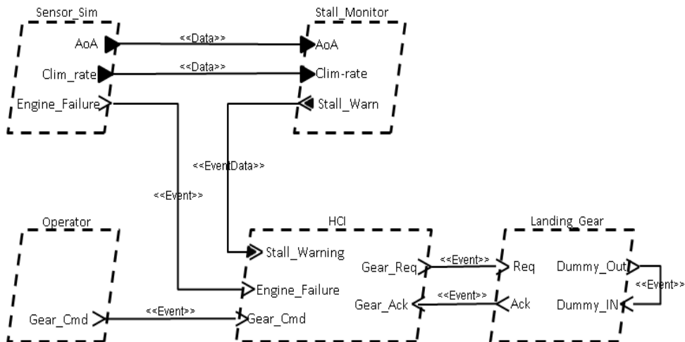
FIG. 8.4 – Architecture du Flight Computer en AADL
