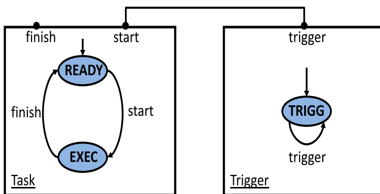
FIG. 7.5 – Architecture du PeriodicTask
