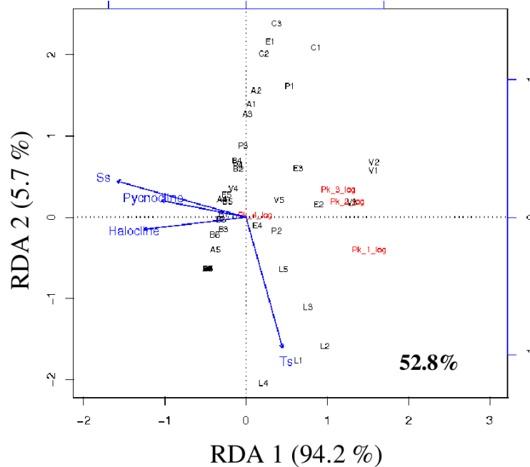
Figure 1.15: RDA biplot diagrams of the abundances of the different larval stages of Pectinaria koreni in May 2008 in the northern Bay of Biscay. Blue arrows represent the biplot scores of hydrological variables. Sampling sites are in black and larval stages in red. The percentage of the total variance explained by the RDA is indicated.
