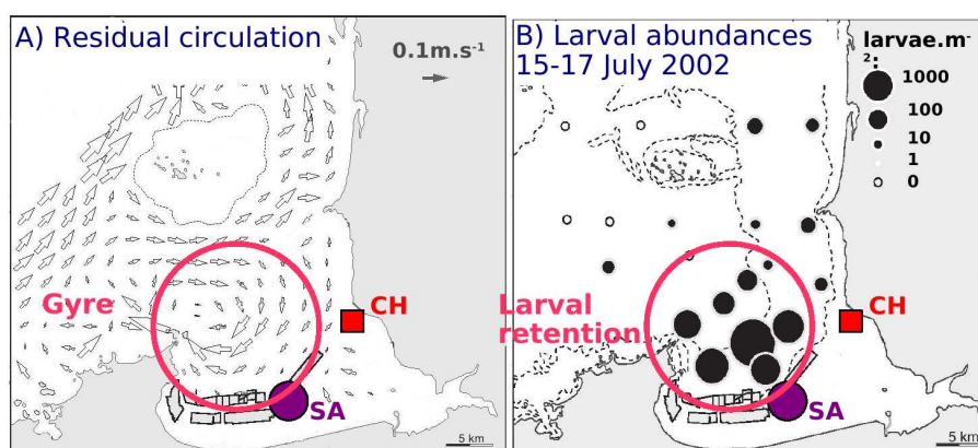
Figure 4.14: Hypothesis of larval retention in the Bay of Mont-Saint-Michel due to the perennial gyre, from Dubois et al. (2007). (A) Residual circulation and (B) In situ distribution of Sabellaria alveolata larvae on 15 to 17 July 2002 in the Bay of Mont-Saint-Michel. Diameters of the circles are proportional to the log-transformed abundance data.
