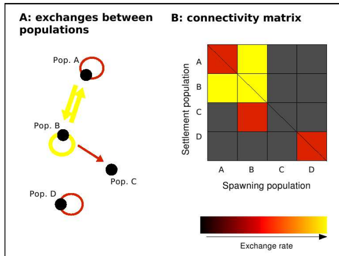
Figure 2.6: Connectivity and connectivity matrix. (A) Example of connectivity patterns for a metapopulation of 4 local populations (Pop. A to Pop. D). Arrows indicate larval exchanges between populations. The arrow width and color are proportional to the intensity of larval exchanges. (B) Corresponding connectivity matrix between the 4 populations. Lighter colors indicate stronger exchanges.
