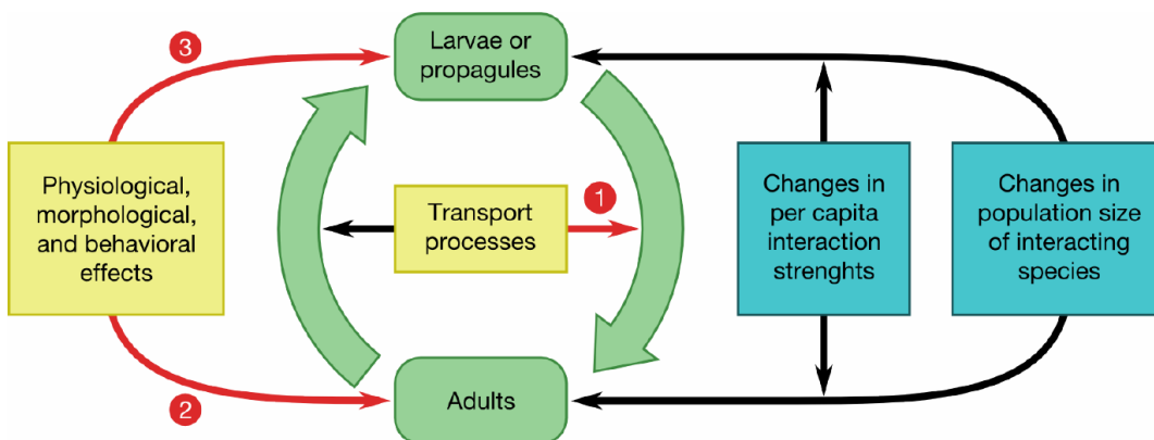
Figure E.1: Potential effects of climate change on a generic marine population (adapted from Harley et al. (2006)). The life cycle of this generic organism is in green. The effects of climate change are in yellow (direct effects) and blue (indirect effects). The arrows in red highlight the effects more specifically investigated in this paper. Numbers are used in the text to refer to these arrows.
