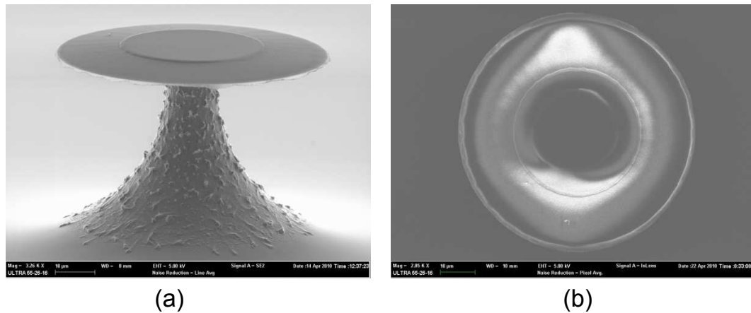
Figure 5.7: SEM graphs of a produced neodymium implanted microdisk. (a) 76^\circ angle view; (b) 90^\circ top view.
