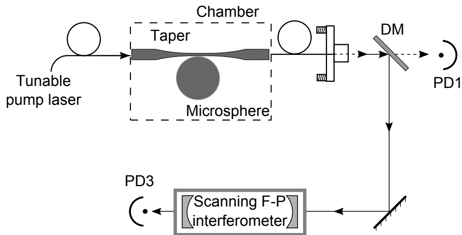
Figure 4.21: Schematic of experimental setup using scanning F-P interferometer.
