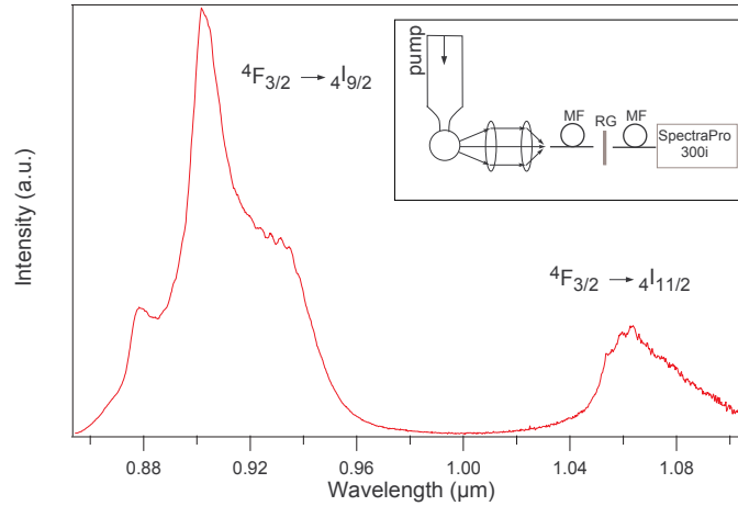
Figure 4.6: Emission spectrum of \text{Nd}^{3+}:\text{Gd}_2\text{O}_3 nanocrystals on a silica microsphere with pump laser coming from its stem (corrected for CCD QE). The two bands around 910 nm and 1060 nm correspond to {}^4F_{3/2} \rightarrow {}^4I_{9/2} and {}^4F_{3/2} \rightarrow {}^4I_{11/2} transitions, respectively. Inset: Schematic of the experimental setup.
