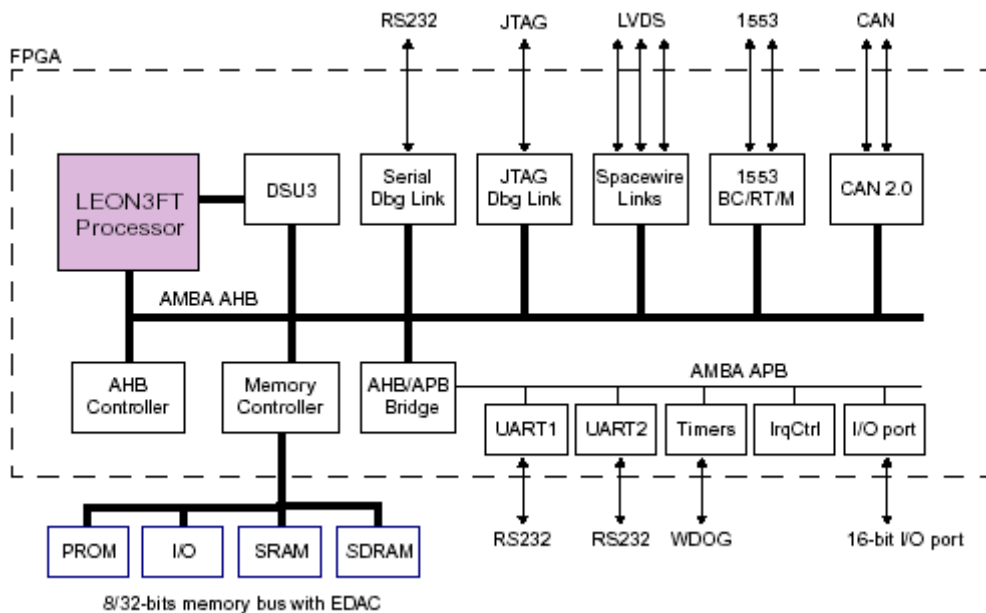
Figure 3-7 : Architecture LEON3
