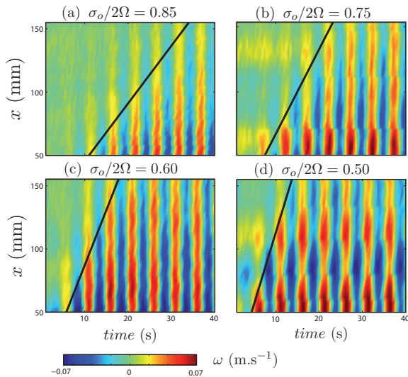
FIG. 6. (Color) Spatiotemporal representation of the vorticity \omega_y along the wave beam, where space is the distance x to the oscillating cylinder, for experiments performed at \sigma_o/2\Omega=0.85, 0.75, 0.60, 0.50 . Black lines originating at (x=0, t=0) trace the front velocity V_f=\sigma(\lambda/2\pi)\tan\theta estimated from the apparent wavelength (see Sec. V A). t=0 corresponds to the start of the oscillation.
