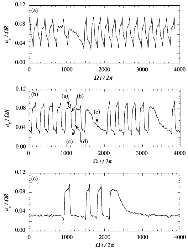
FIG. 10. Time series of u_x(x=-R/2, z=0) , corresponding to the near-heteroclinic cycle state (Het), for Re \approx 452, 469, and 478 . The labels (a)–(e) in the second time series refer to the velocity fields in Fig. 11.
