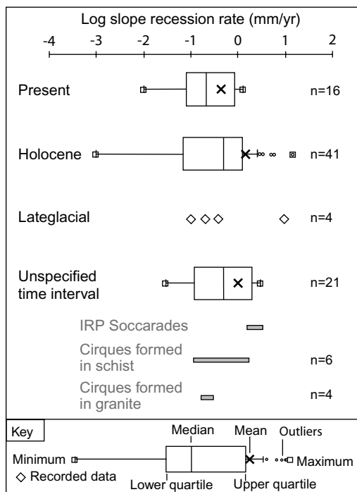
Fig. 10. Box and whiskers plots highlighting variability in slope recession rates (see Suppl. Table 7). Note homogeneity of IQR ( 1-10^{-1} \text{ mm yr}^{-1} ) irrespective of measurement interval. Wider spread of Holocene series is probably linked to a mix of data from environments where deglacial debuttressing occurred at different times during the Holocene. This relates, therefore, to the issue of periodization discussed in Section 6.2. This may also be due to disparities in the sensitivity of bedrock materials to detachment. However, a reclassification of the data based on lithology did not reveal any clear trends, suggesting that the key factors could be other defining parameters of rock mass strength such as fracture density.
