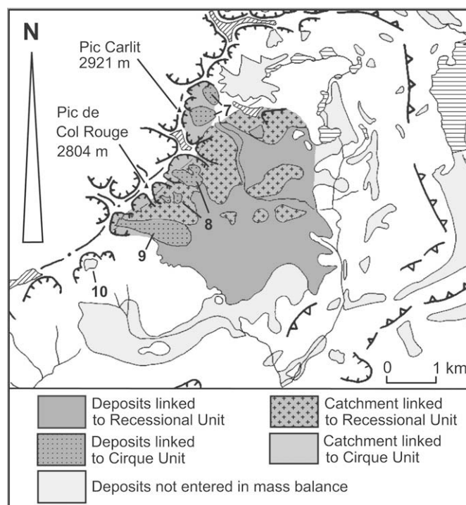
Fig. 8. Close-up of the Soccarades area (see Fig. 6 for location).
