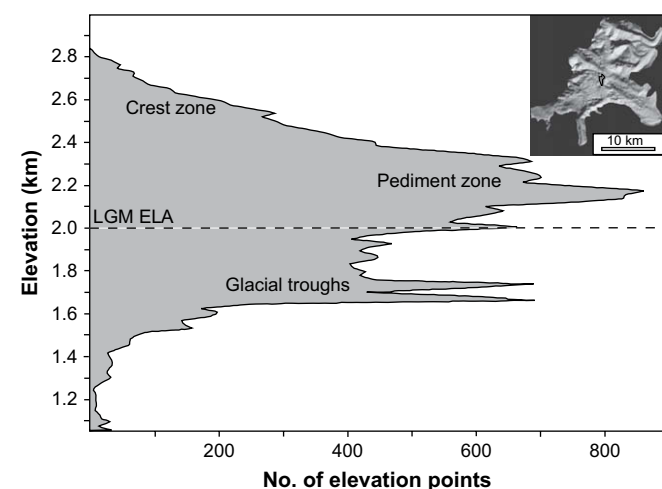
Fig. 4. Hypsometry of the area glaciated during the Pleistocene. Note low-gradient topography between 2.4 and \sim 2.0 km a.s.l. corresponding to the pediment zone visible in Fig. 3. Inset shows area relevant to the hypsometric curve (digital elevation data from the Shuttle Radar Topography Mission).
