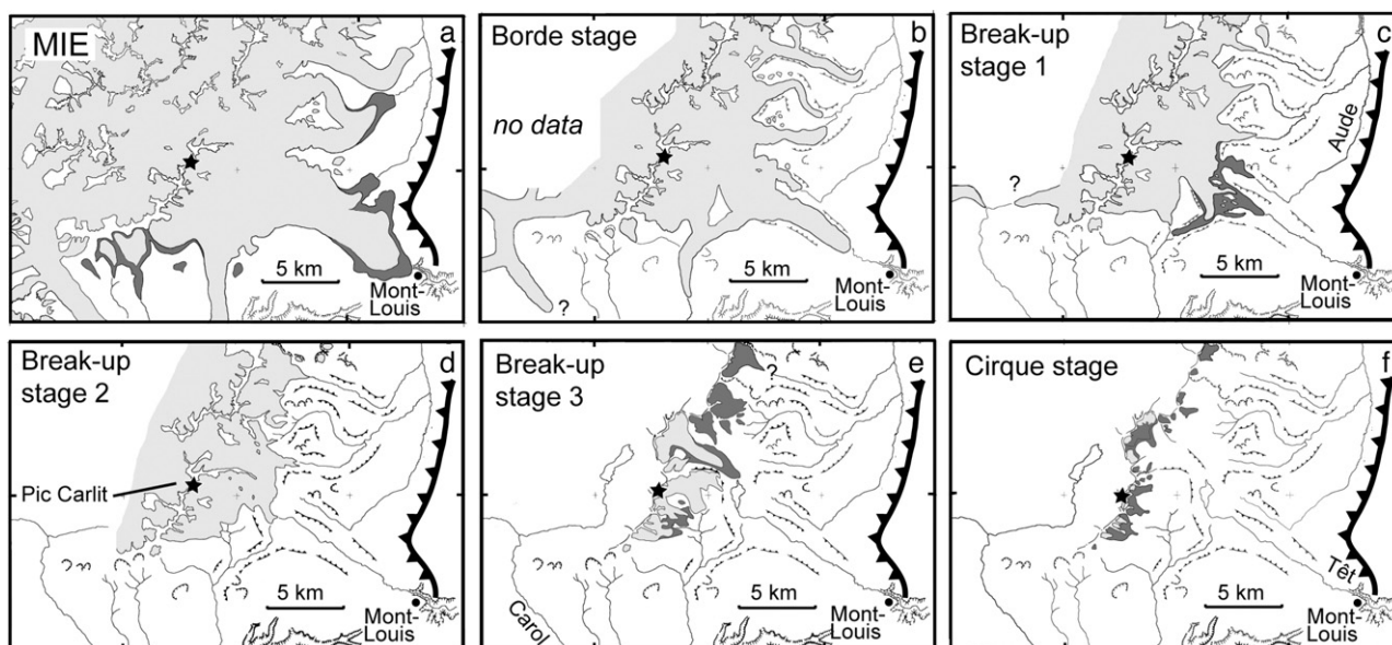
Figure 4. Reconstruction of the Carlit ice cap at successive recessional stages (a to f) based on detailed geomorphological mapping from aerial photographs and field reconnaissance. Symbols, ornaments and lat/long tick marks as in Figure 3. At each stage, dark gray and light gray shading define the uncertainty of glacier extent (i.e., maximum and minimum position of ice fronts, respectively) linked to the mapping method.
