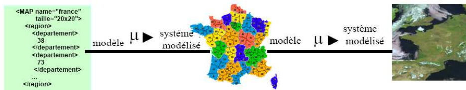
FIG. 4.2: La relation \mu [BBB + 05]
