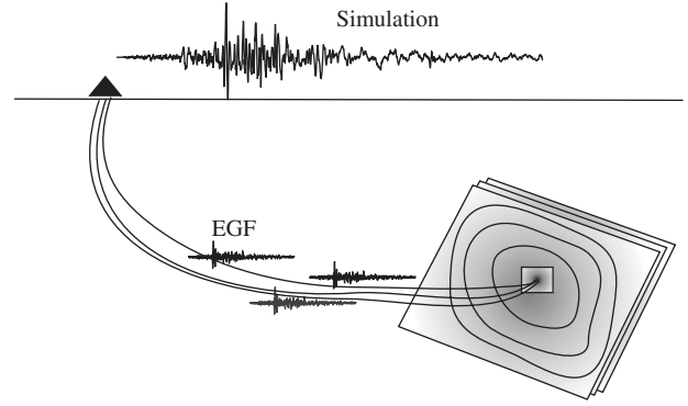
Figure 1. Principle of the EGF summation method. The recordings of a single small earthquake are combined several times to produce simulated recordings for a larger event at a given station.
