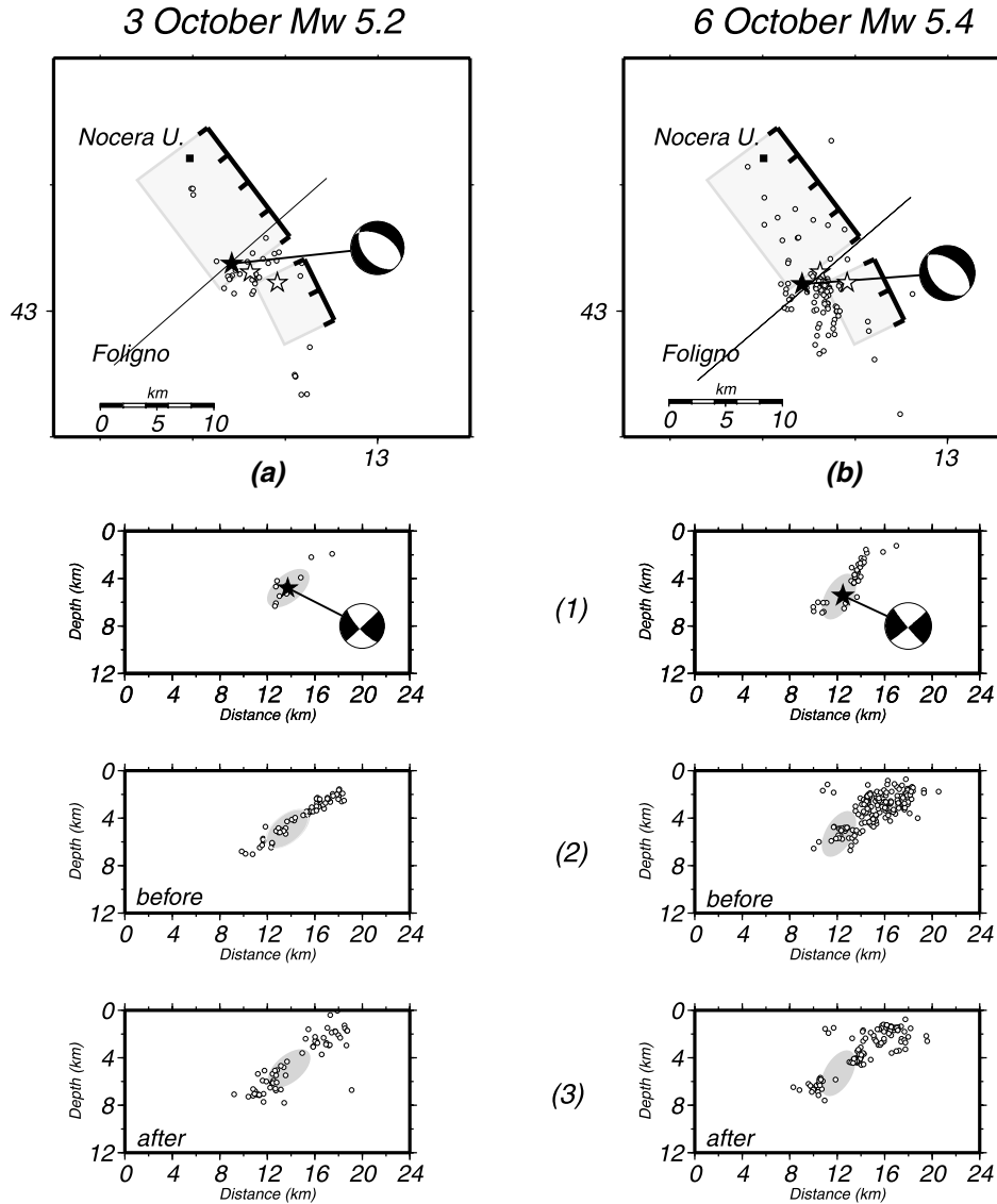
Figure 12. Distribution of seismicity associated with the (a) 3 October and (b) 6 October earthquakes. The maps show the mainshock epicenters (solid stars) and the fault-plane solutions for these two events (in a and b, respectively), the location of the two main events of 26 September (open stars), and their surface projection. The straight line in the map shows the position of the northeast–southwest vertical cross section used to image seismicity in the panels below. The cross sections show the seismicity that occurred in three time intervals: (1) 12 hr following the mainshock, (2) the previous 7 days, and (3) 12 hr after the mainshock through November 1997. The shaded areas depict the inferred portion of the fault planes ruptured during the (a) 3 October and (b) 6 October earthquakes.
