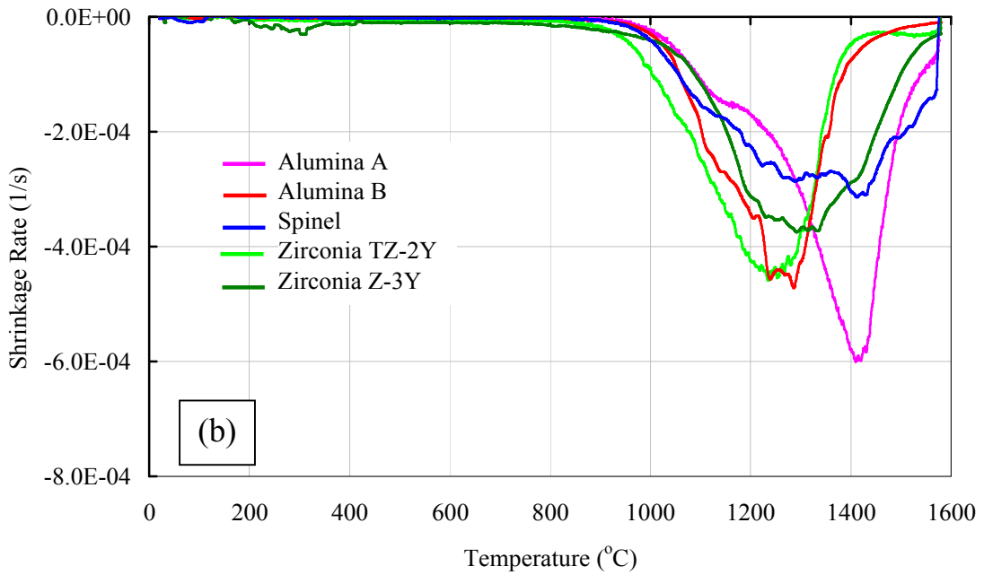
Figure 5.4. Shrinkage behaviors of powder compacts (UP 250MPa) of alumina B, alumina A, zirconia Z-3Y, zirconia TZ-2Y and spinel (a) relative shrinkage and (b) shrinkage rate curves during sintering up to 1580°C with heating rate of 3.3°C/min.
