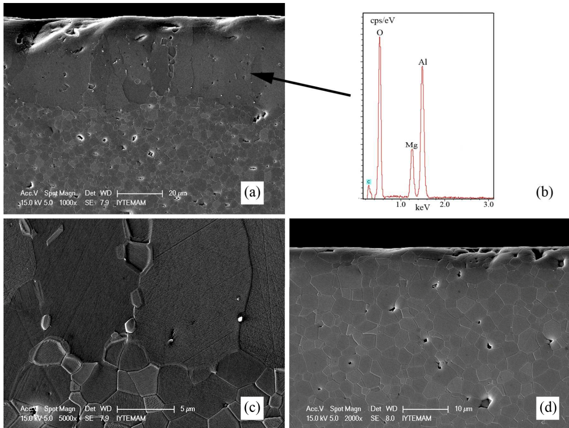
Figure 6.20. Cross-sectional images of alumina end-member and the EDS result (Experiment no 1); the width of spinel columnar grains ( 8\ \mu\text{m} ) is larger than in the co-sintering case ( < 5\ \mu\text{m} ).
