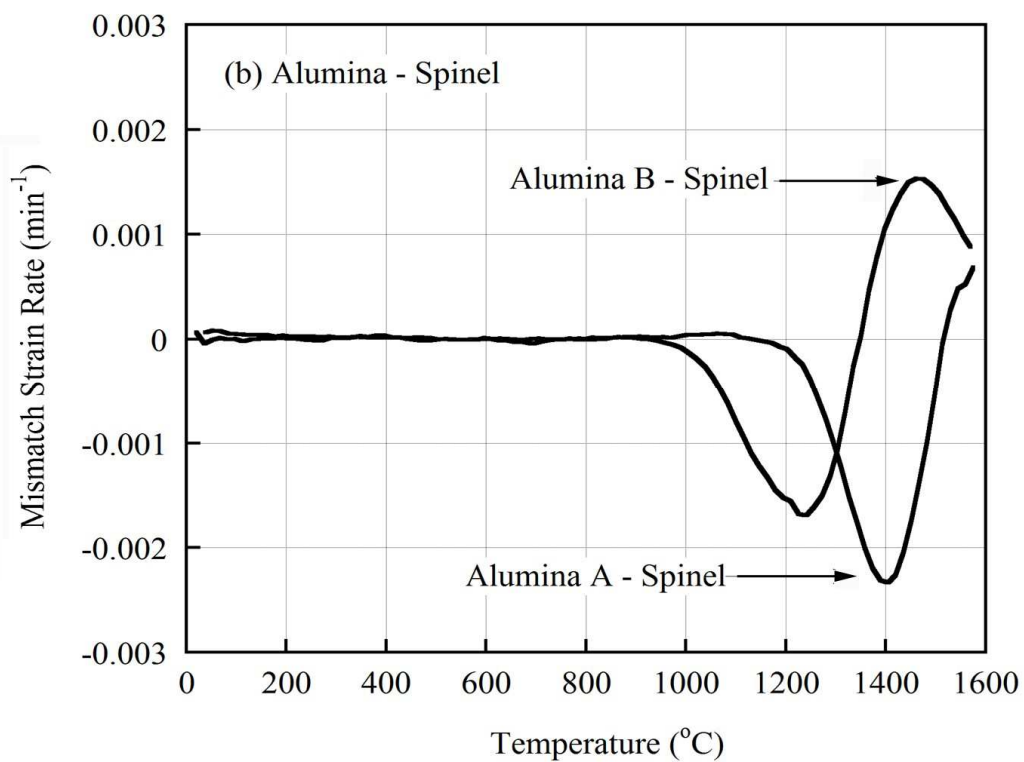
Figure 5.6. Mismatch strain rates of individual powder compacts (UP 250 MPa) of (a) alumina – zirconia, (b) alumina – spinel sintered up to 1580 ^{\circ}\text{C} with heating rate of 3.3 ^{\circ}\text{C}/\text{min} .
