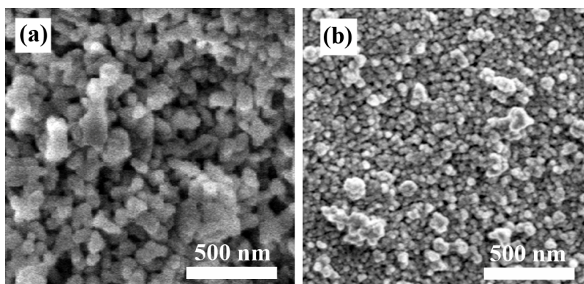
Figure 3.7. SEM images of powder compacts, CIPed at 250MPa (a) alumina B, (b) zirconia TZ-2Y.
