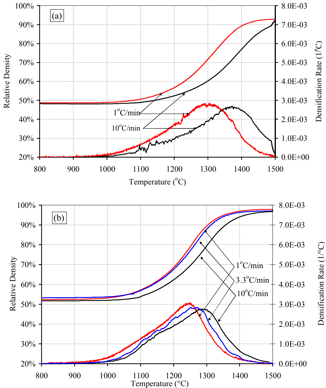
Figure 3.13. Densification curves during sintering at heating rates of 1, 3.3 and 10°C/min for powder compacts of (a) alumina A and (b) alumina B. The upper and lower curves in all (a) and (b) are the relative densities, \rho , and their temperature derivatives, d\rho/dT , respectively (all the samples were CIPed at 250 MPa).
