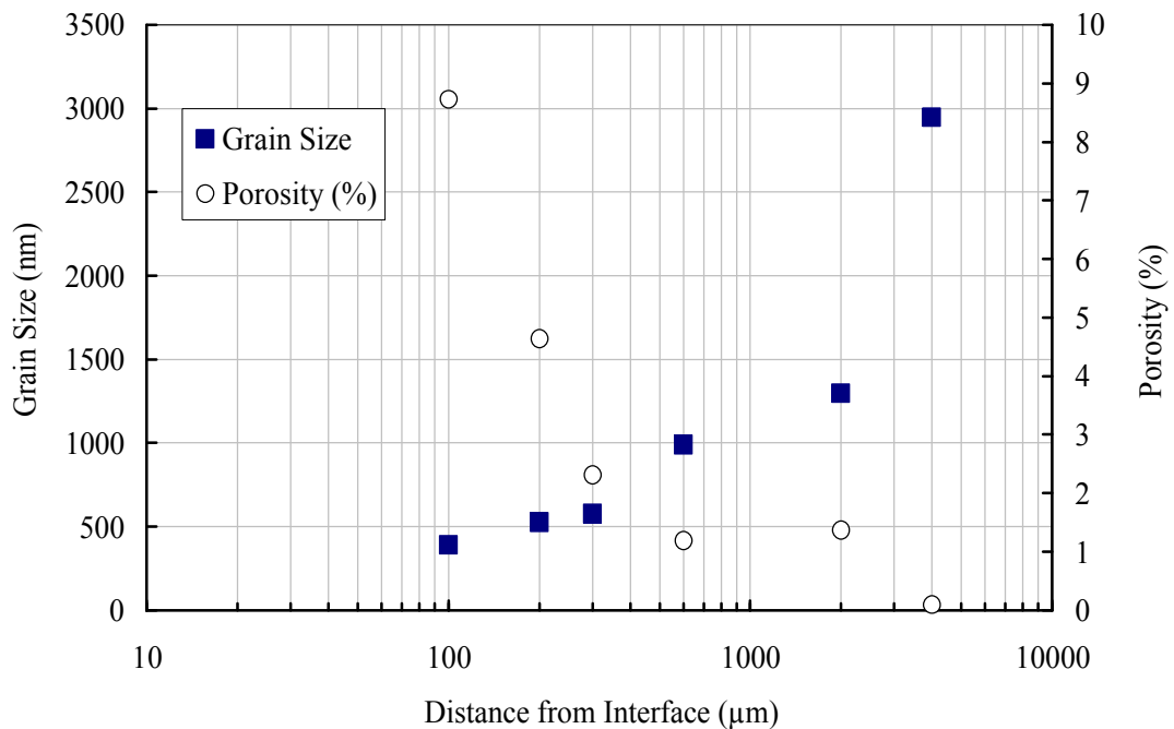
Figure 6.11. Porosity and grain size profiles from interface to interior of spinel for alumina A – spinel bi-material. The two sintering steps were done at 1400°C for 16 hours followed by another sintering at 1500°C for 16 hours. Sample was chemically etched at 140°C for 15 min in orthophosphoric acid.
