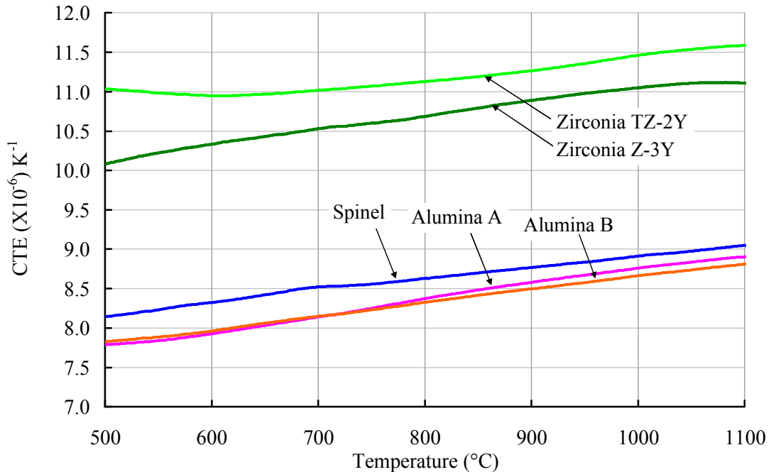
Figure 5.11. Thermal Expansion Coefficients of mono-materials up to 1100°C. Dilatometric data obtained with nearly fully dense samples during the heating step of a thermal cycle (10°C/min).
