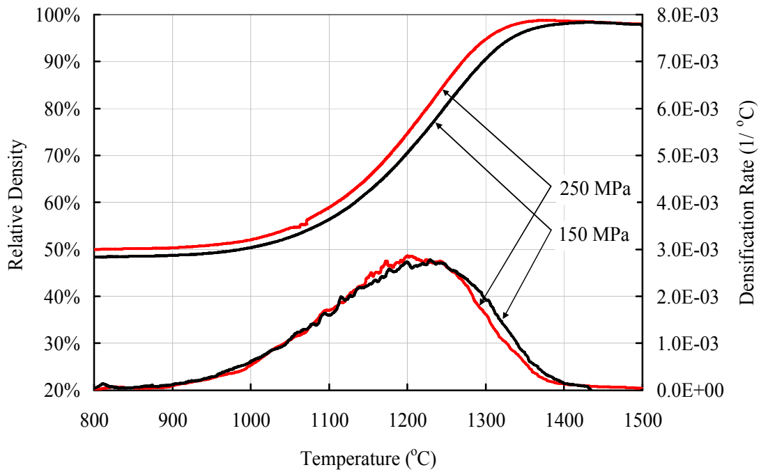
Figure 3.17. Effect of CIP compaction pressure on the sintering of zirconia TZ-2Y, 1°C/min heating rate.
