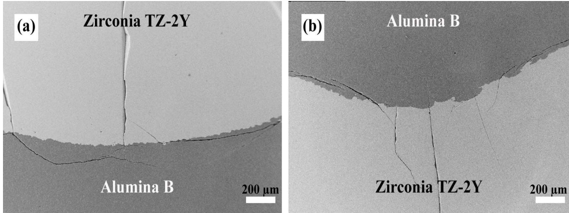
Figure 5.10. Compaction (Co-UP 250 MPa) order and cracks formation on the alumina B – zirconia TZ-2Y bi-materials (a) alumina B – zirconia TZ-2Y bi-material, (b) zirconia TZ-2Y – alumina B bi-material.
