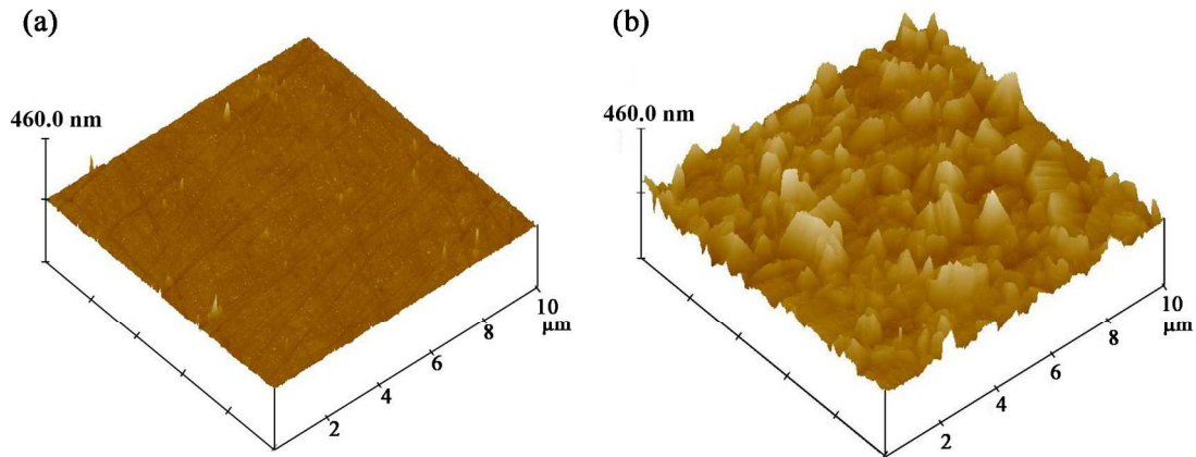
Figure 4.4. Effect of thermal etching on the roughness of spinel (99% dense) surface (a) as-polished and un-etched surface and (b) thermally etched surface.
