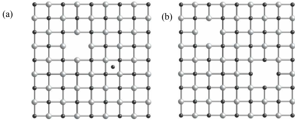
Figure 2.5. Schematic of (a) a Frenkel defect and (b) a Schottky defect drawn in 2D (Source : Carter and Norton 2007).
