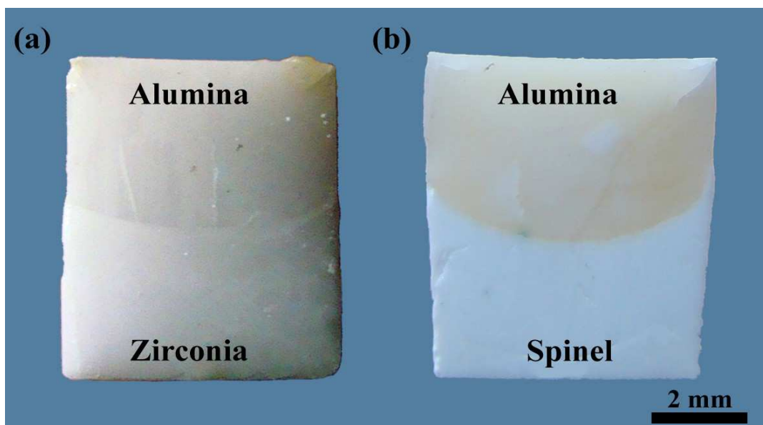
Figure 5.7. Shapes of the bi-materials (a) zirconia TZ-2Y – alumina B (Co-UP 150 MPa), (b) spinel – alumina B (Co-UP 250 MPa). (alumina part at the top in all photos). Co-sintering conditions : 1°C/min up to 1580°C.
