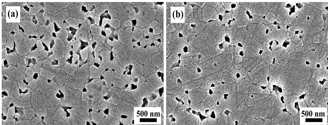
Figure 4.25. SEM images of the spinel specimens sintered with (a) SSS-I and (b) TSS-I.
