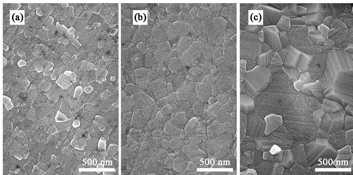
Figure 4.10. Scanning electron micrographs of spinel ceramic sintered at 1500°C for (a) 1 hour, (b) 4 hours and (c) 16 hours (3.3°C/min heating rate up to 1500°C).
