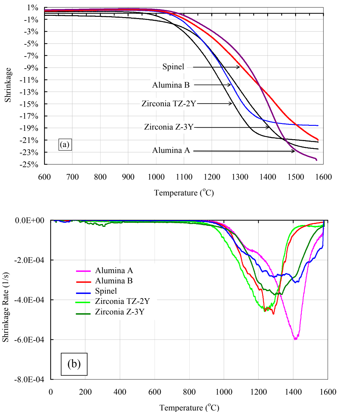
Figure 5.4. Shrinkage behaviors of powder compacts (UP 250MPa) of alumina B, alumina A, zirconia Z-3Y, zirconia TZ-2Y and spinel (a) relative shrinkage and (b) shrinkage rate curves during sintering up to 1580°C with heating rate of 3.3°C/min.
