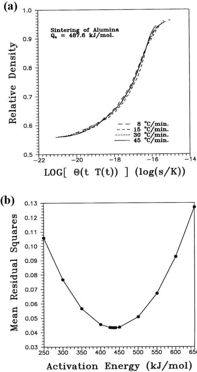
Figure 2.9. (a) Master Sintering Curves of alumina and (b) Mean of Residual Square versus activation energy (Source: Su and Johnson 1996).
