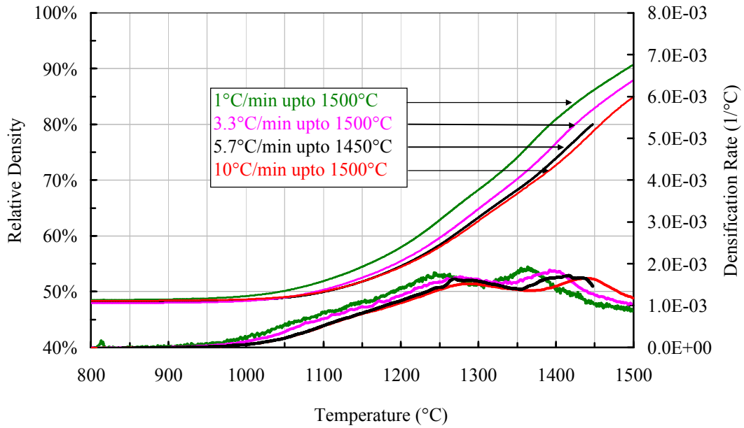
Figure 4.8. Densification and densification rate curves of spinel powder compacts (50 MPa Uniaxial Pressing + 250 MPa Cold Isostatic Pressing).
