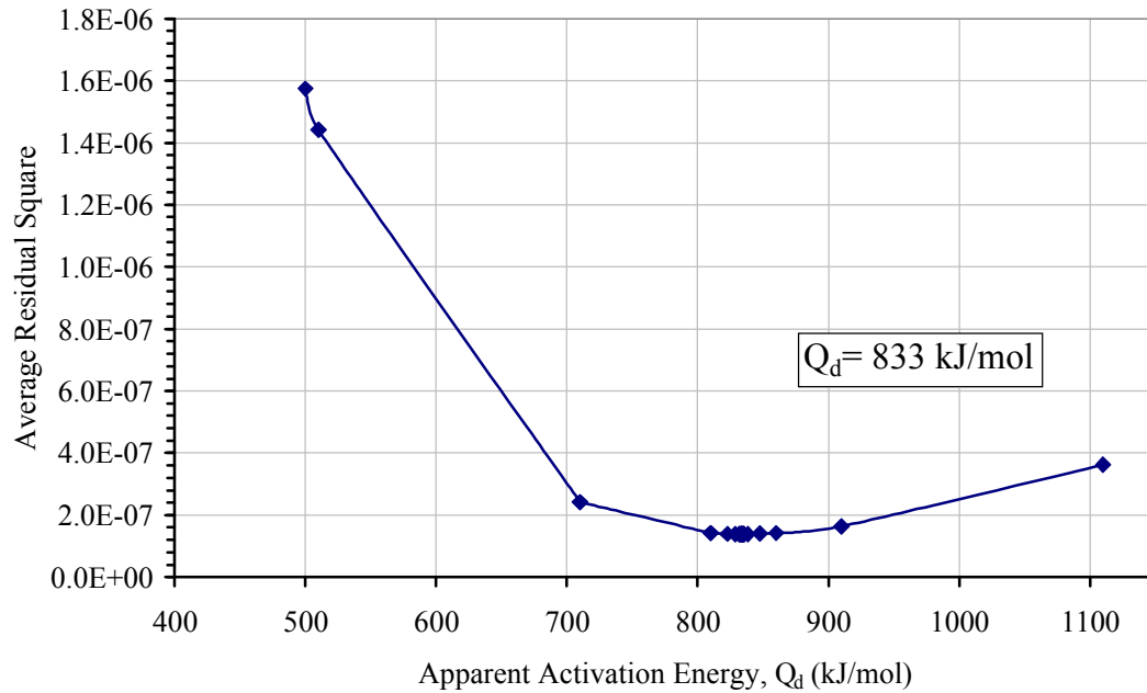
Figure 4.16. Master Sintering Curve : Average residual square versus apparent activation energy ( Q_d ).
