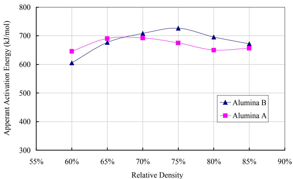
Figure 3.23. Apparent activation energies for densification versus relative densities of alumina A and alumina B powders.
