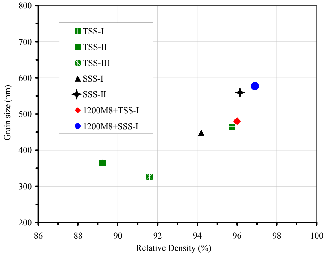
Figure 4.24. Sintering paths of spinel specimens : grain size vs. relative density for Single Step Sintering (SSS) and Two Steps Sintering (TSS).
