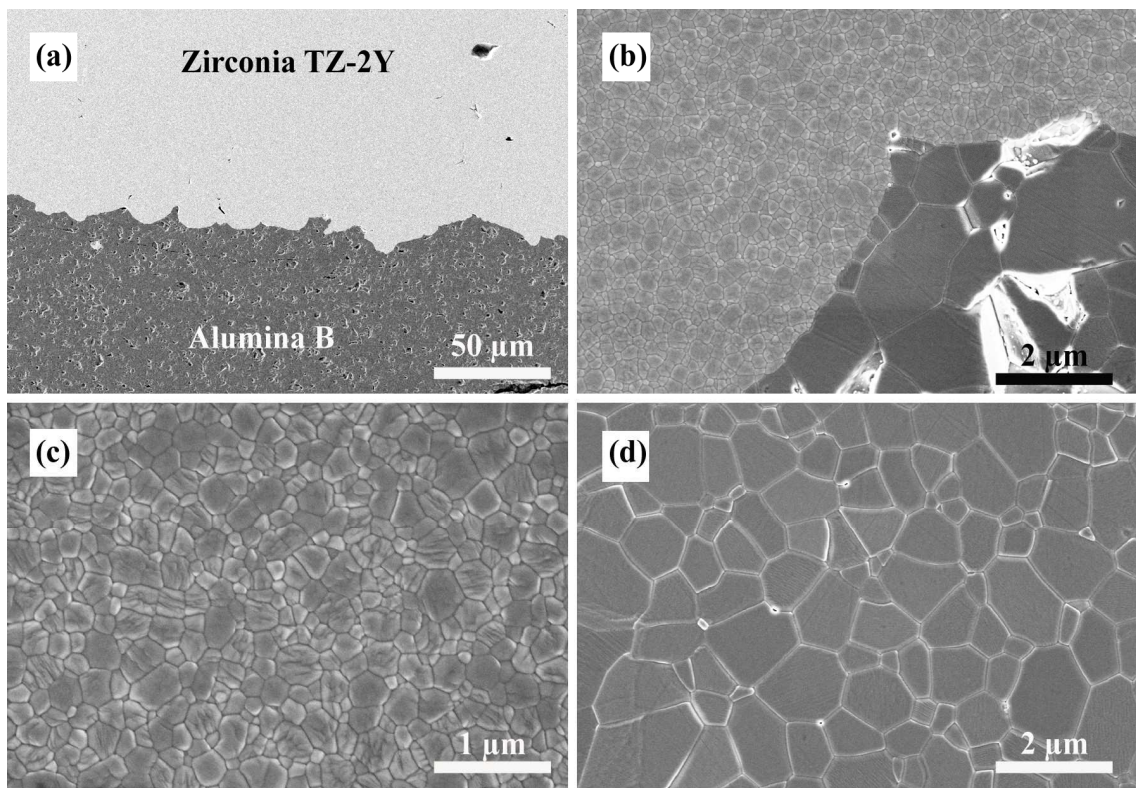
Figure 5.12. SEM micrographs of alumina B – zirconia TZ-2Y bi-material interface and components (a) interface, (b) interface at higher magnification, (c) zirconia TZ-2Y region, (d) alumina B region. (Co-UP at 250 MPa) and co-sintered up to 1580°C at 3.3°C/min.
