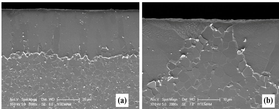
Figure 6.21. SEM cross-sectional images of alumina end-member (a) general cross section view and (b) a non-contact region among the nodules (Exp. no 2).
