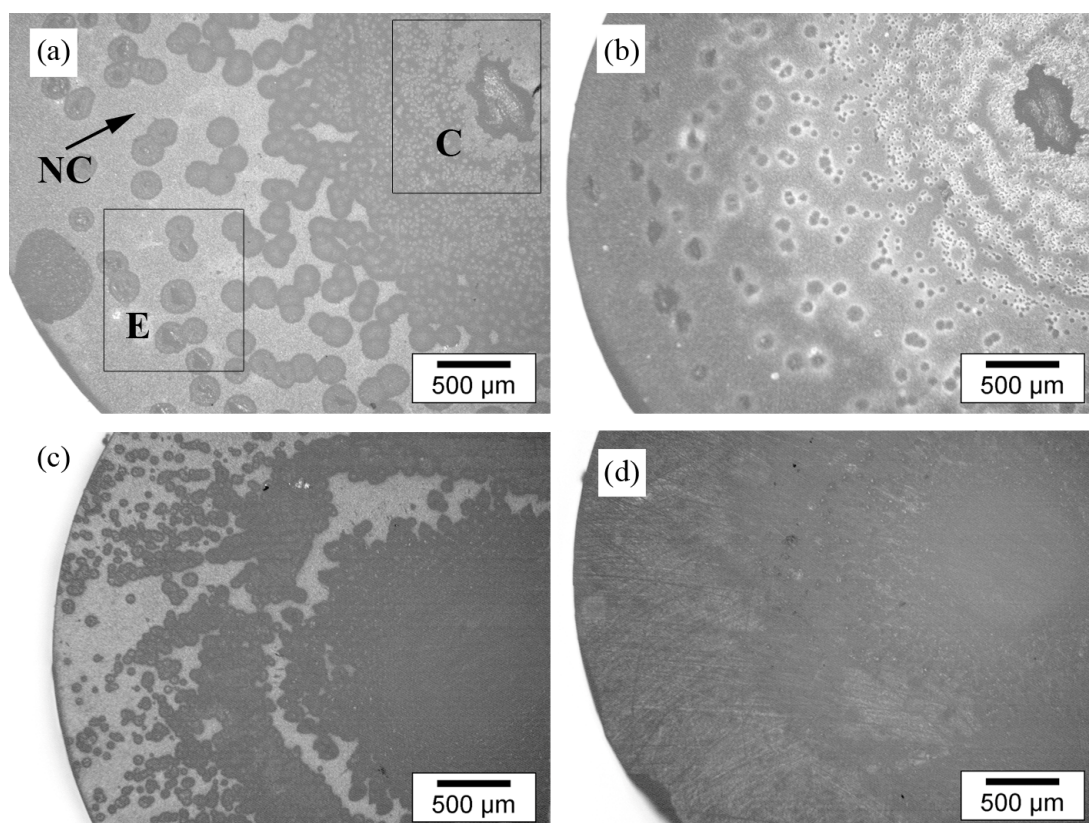
Figure 6.13. Contact surfaces of the end-members (a) predensified (95 %) alumina A (E: external part, C: central part of the sample) and (b) predensified (95%) spinel after diffusion couple test 1. Photographs show (c) predensified alumina A and (d) spinel after diffusion couple test 2 (1500°C 16 hours).
