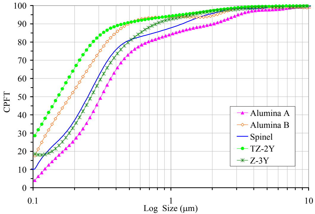
Figure 3.3. Particle size distribution curves of the powders.
