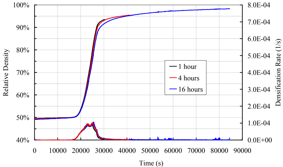
Figure 4.9. Densification and densification rate curves during isothermal sintering cycles at 1500°C for the study of spinel grain growth (3.3°C/min heating rate up to 1500°C).
