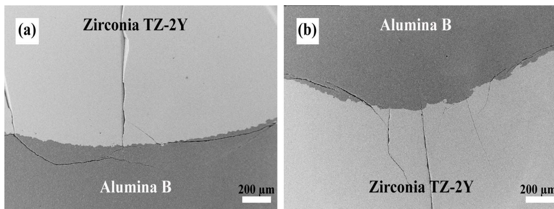
Figure 5.10. Compaction (Co-UP 250 MPa) order and cracks formation on the alumina B – zirconia TZ-2Y bi-materials (a) alumina B – zirconia TZ-2Y bi-material, (b) zirconia TZ-2Y – alumina B bi-material.
