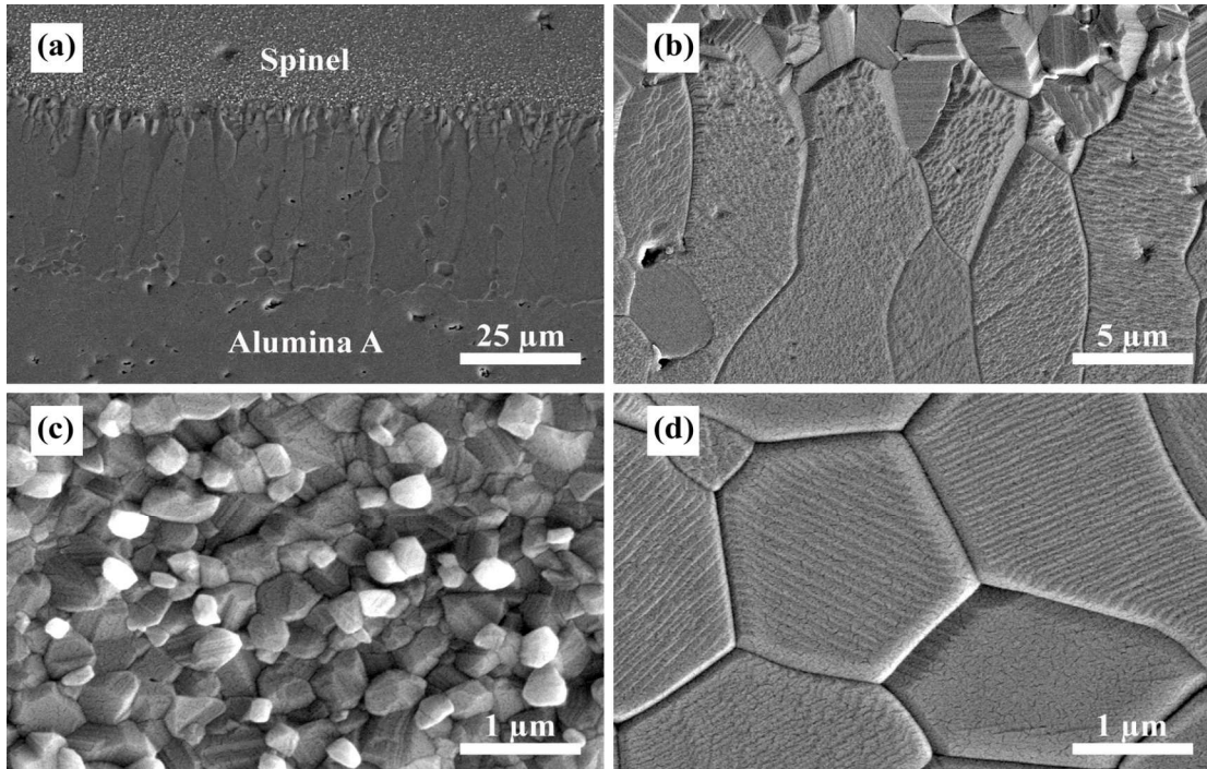
Figure 5.15. Alumina A – spinel bi-material, produced by double-action mode of uniaxial pressing at 250 MPa (Co-UPFlo) (a) general view of interlayer, (b) columnar grains at the interlayer (c) spinel grains in spinel and (d) alumina grains in alumina. Co-sintering conditions : 1500°C for 16 hours.
