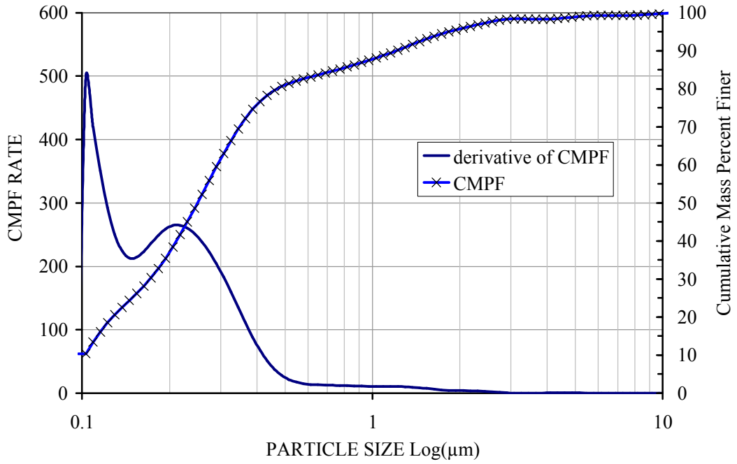
Figure 4.1. Particle size distribution of spinel powder measured by Sedigraph method.
