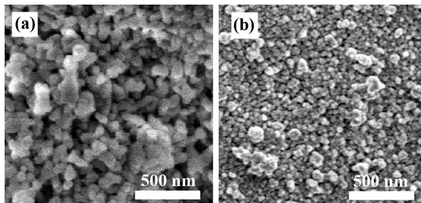
Figure 3.7. SEM images of powder compacts, CIPed at 250MPa (a) alumina B, (b) zirconia TZ-2Y.
