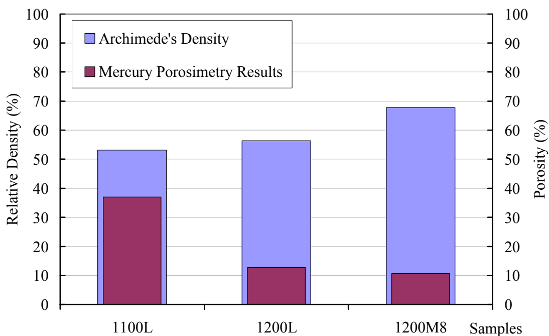
Figure 4.21. Density and porosity measurements (Archimedes and Mercury) showing the effect of a pretreatment on the structure of spinel compacts.
