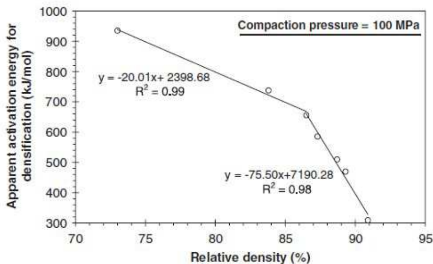
Figure 3.1. Apparent activation energy versus relative density for for yttria-doped zirconia (Source: Bernard-Granger and Guizard 2007b).
