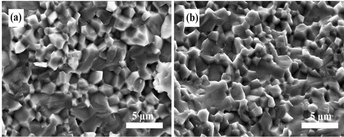
Figure 3.14. SEM micrographs of fracture surfaces of sintered alumina B powder specimens (CIP 250 MPa) treated at different heating rates (a) 1°C/min and (b) 10°C/min, without a soaking time at 1500°C.
