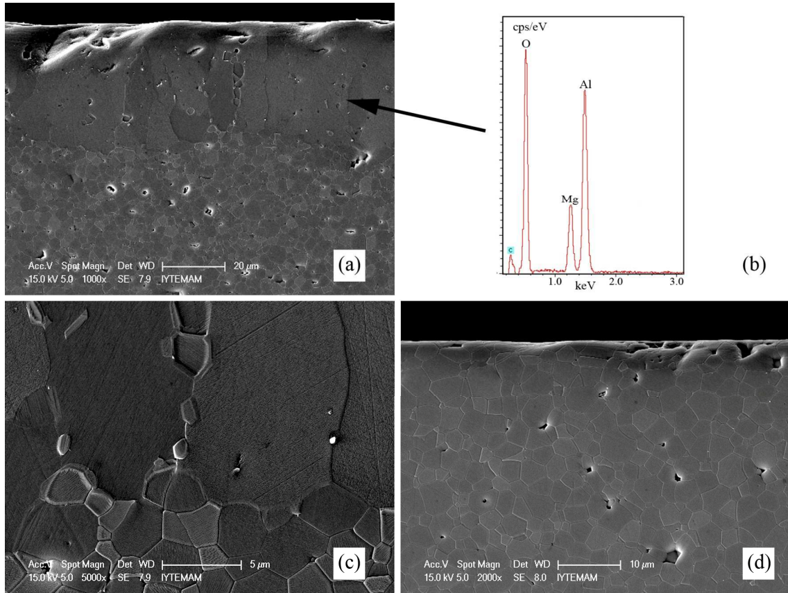
Figure 6.20. Cross-sectional images of alumina end-member and the EDS result (Experiment no 1); the width of spinel columnar grains (8 μm) is larger than in the co-sintering case (< 5 μm).
