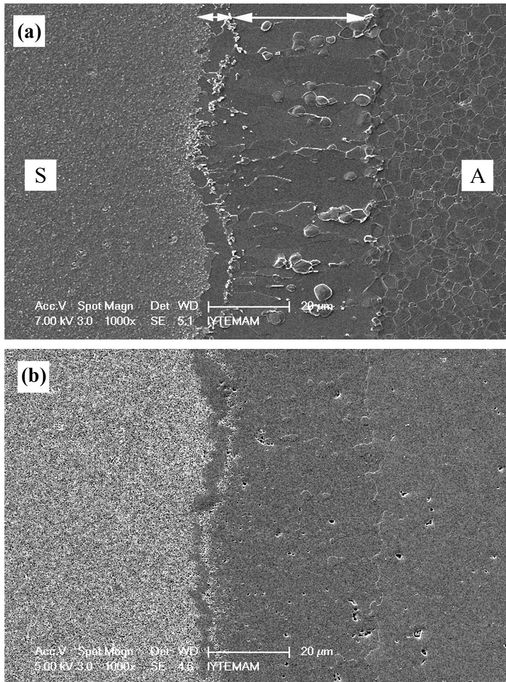
Figure 6.9. SEM image of alumina A – spinel bi-material interlayer after two isothermal steps co-sintering (16 hours at 1400°C + 16 hours at 1500°C) (a) thermally etched surface (b) chemically etched surface.
