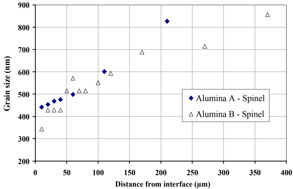
Figure 6.6. Spinel grain size profiles from interface to interior of spinels for each type of co-sintered bi-material for 16 hours at 1500°C. Polished cross sections were thermally etched at 1450°C for 30 min.
