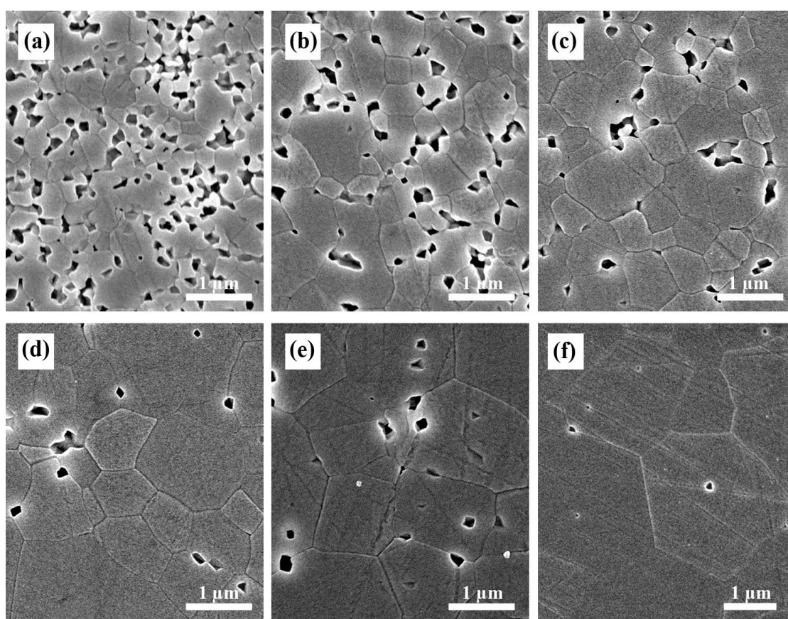
Figure 6.10. SEM images of parent spinel end-member in alumina A – spinel bi-material (a) 100 \mu\text{m} , (b) 200 \mu\text{m} , (c) 300 \mu\text{m} , (d) 600 \mu\text{m} away from the interlayer into bulk of the parent spinel and (e) at the center and (f) at the edge of parent spinel. The two sintering steps were done at 1400°C for 16 hours followed by another sintering at 1500°C for 16 hours. Sample was chemically etched at 140°C for 15 min in orthophosphoric acid.
