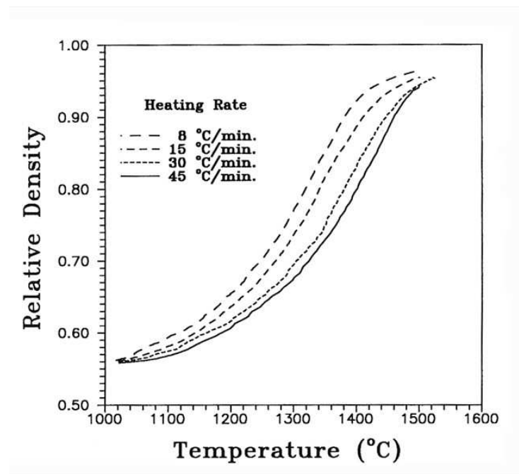
Figure 2.8. Relative densities versus temperature curves of alumina, sintered with different heating rates (Source: Su and Johnson 1996).
