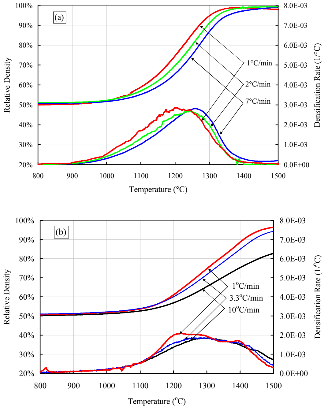
Figure 3.16. Densification curves during sintering at different heating rates for powder compacts of (a) zirconia TZ-2Y and (b) zirconia Z-3Y. In both graphs, the upper curves are the relative densities, \rho , and the lower curves are their temperature derivatives, d\rho/dT , respectively.
