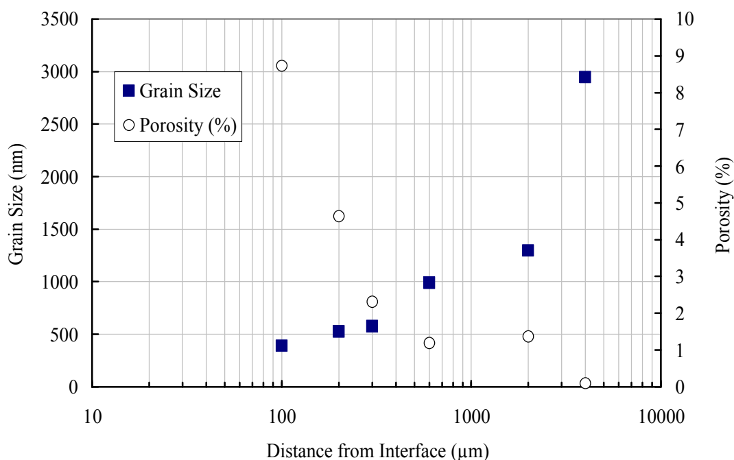
Figure 6.11. Porosity and grain size profiles from interface to interior of spinel for alumina A – spinel bi-material. The two sintering steps were done at 1400°C for 16 hours followed by another sintering at 1500°C for 16 hours. Sample was chemically etched at 140°C for 15 min in orthophosphoric acid.
