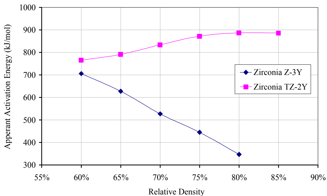
Figure 3.22. Apparent activation energies for densification versus relative densities of zirconia Z-3Y and TZ-2Y powders.
