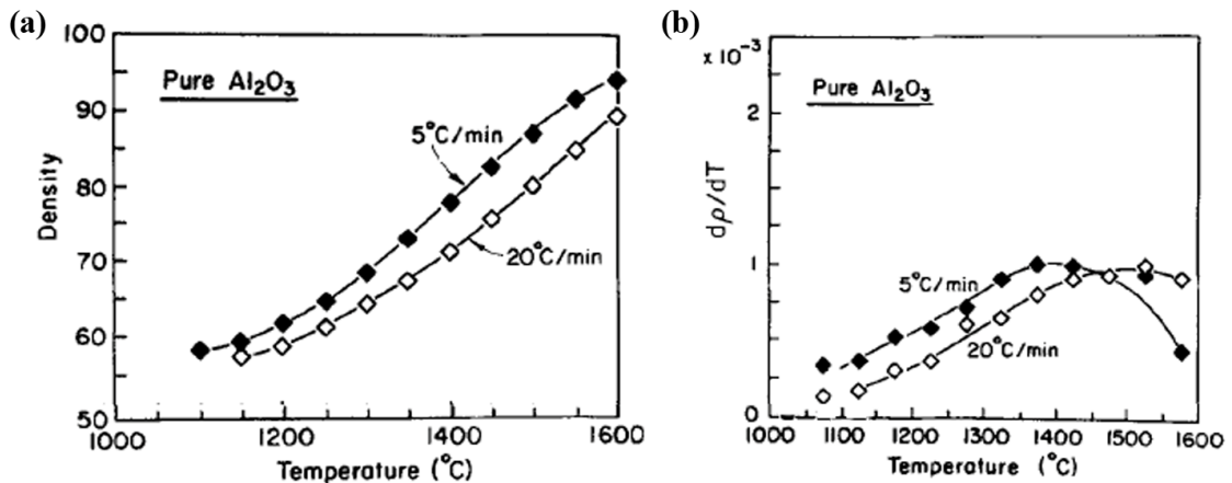
Figure 2.6. Relative density (a) and densification rate (b) versus temperature graphs of alumina (Source: Wang and Raj 1990).
