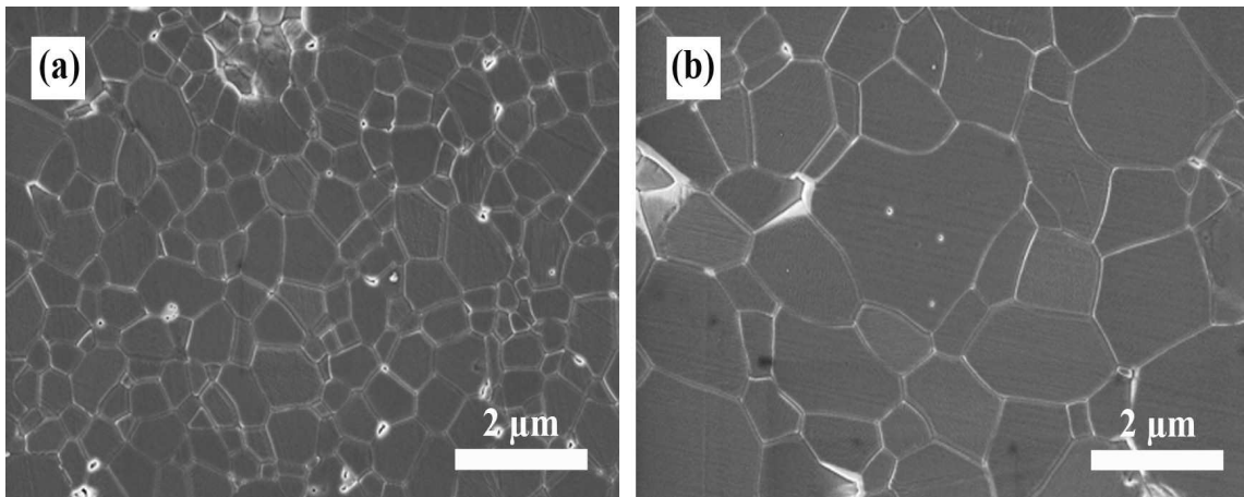
Figure 3.15. SEM images of polished and thermal etched surfaces of sintered powder specimens (a) alumina A and (b) alumina B (CIP 250 MPa), treated with 1°C/min heating rate for 1 hour soaking time at 1500°C.
