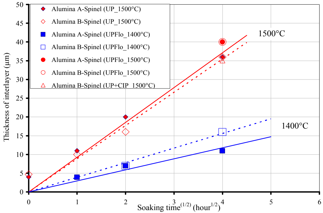
Figure 6.7. Effect of soaking time, pressing method and temperature on the interlayer thickness of alumina – spinel co-sintered bi-materials.
