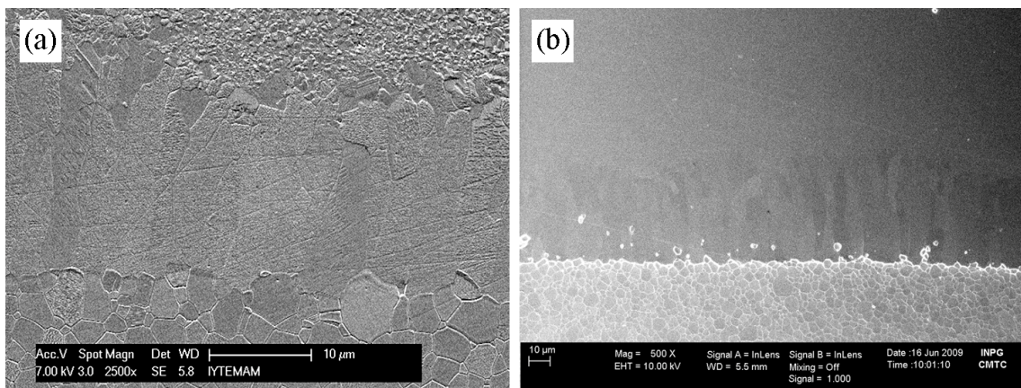
Figure 5.16. SEM images of alumina B – spinel bi-materials produced by (a) single-action mode and (b) floating die mode, of uniaxial pressing followed by cold isostatic pressing at 250 MPa. (Spinel part at the top in all photos). Co-sintering conditions: (a) 1°C/min up to 1580°C, (b) 1500°C for 16 hours.
