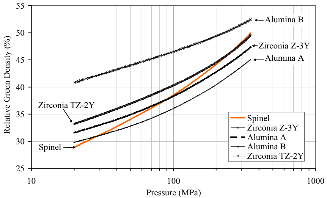
Figure 3.6. The compaction diagrams of powders with single action mode uniaxial pressing.
