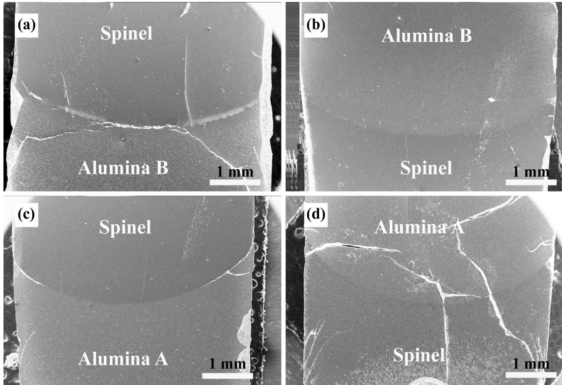
Figure 5.13. Compaction order of alumina and spinel bi-combinations, produced by single-action mode of uniaxial pressing at 250 MPa (Co-UP) (a) alumina B – spinel bi-material, (b) spinel – alumina B bi-material, (c) alumina A – spinel bi-material, (d) spinel – alumina A bi-material. Sintering conditions : 3.3°C/min up to 1580°C.
