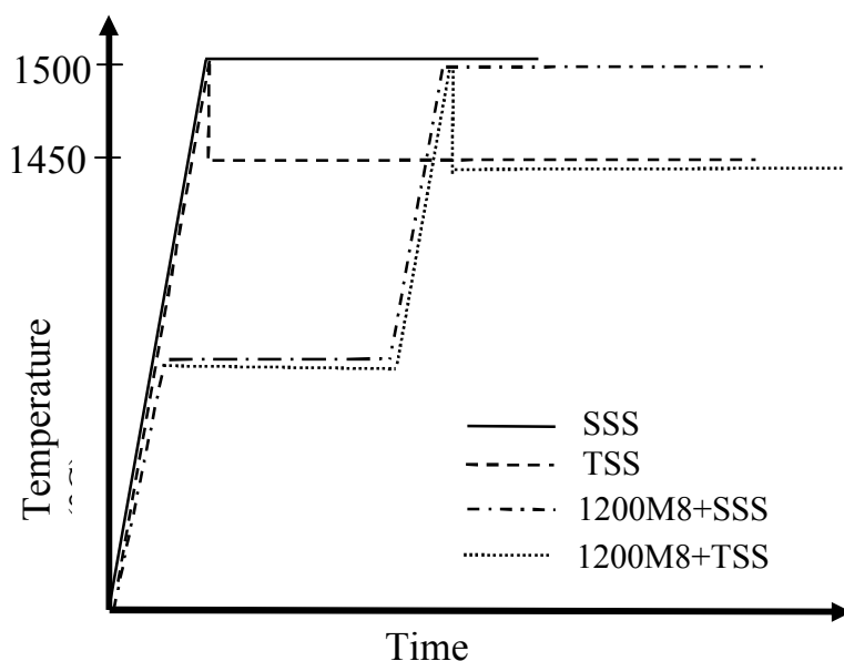
Figure 4.23. Heating regimes used in two-step sintering experiments as well as in the isothermal sintering and combination of precoarsening and single or two steps sintering tests.
