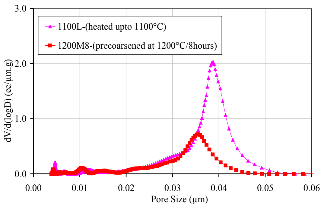
Figure 4.20. Effect of pretreatment on the pore-size distribution of spinel samples (mercury porosimetry).
