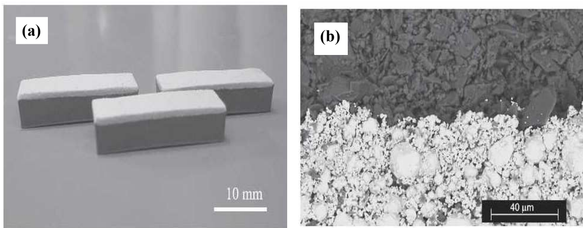
Figure 2.13. W/Al 2 O 3 bilayer specimens, (a) a macroscopic view and (b) a micrograph of the interfacial region (Source: Boonyongmaneerat and Schuh 2006).
