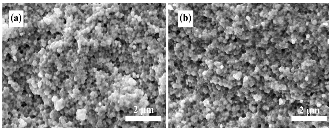
Figure 3.18. SEM micrographs of sintered zirconia TZ-2Y powder specimens, compacted at different pressures of (a) CIP 150 MPa and (b) CIP 250 MPa, were sintered at 1500°C with 1°C/min heating rate.
