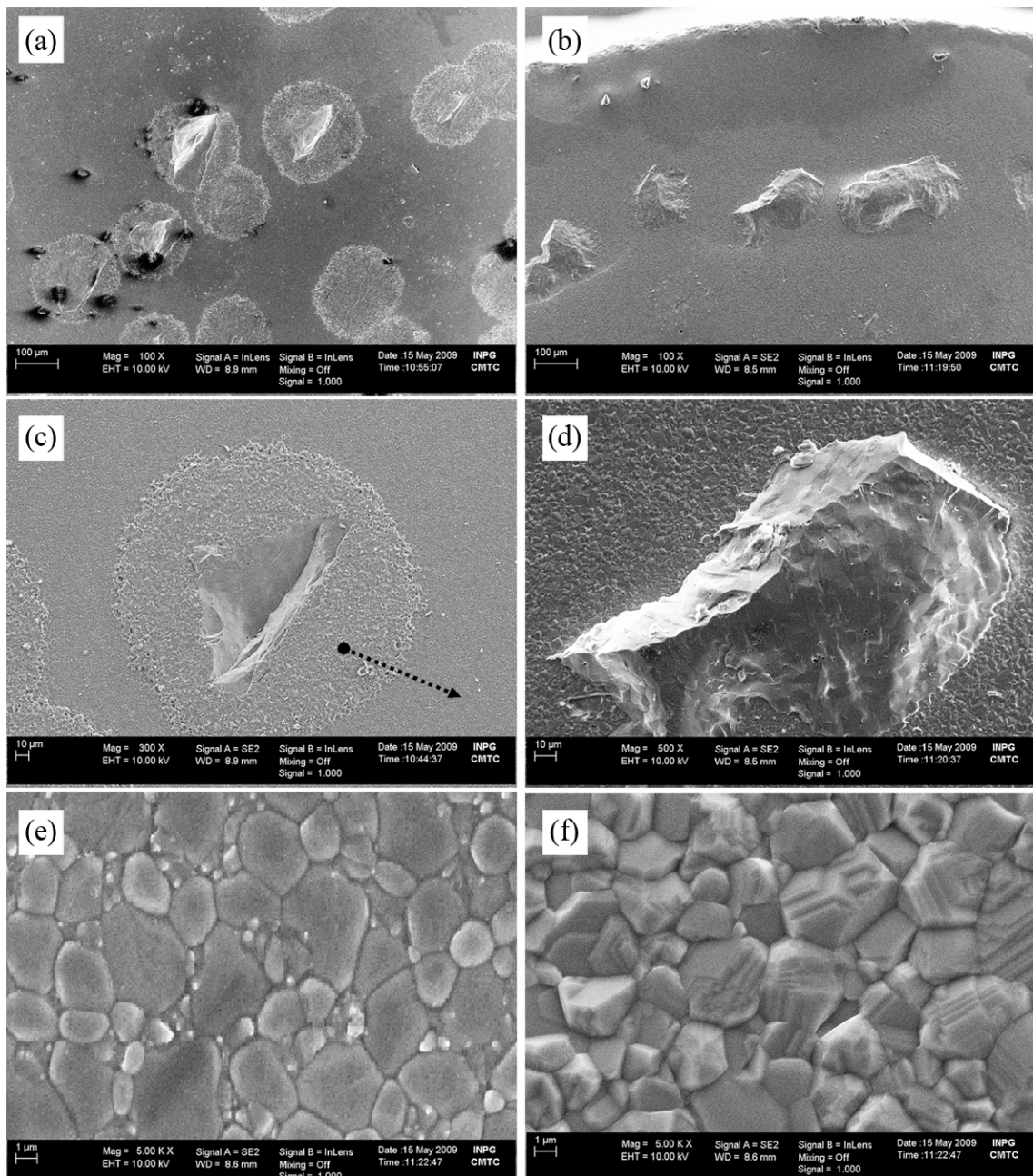
Figure 6.14. The SEM images of surfaces of predensified alumina and spinel end-members (Exp. No 1) (a), (c) and (e) alumina, (b), (d) and (f) spinel.
