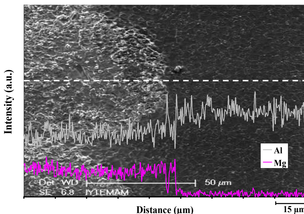
Figure 6.18. Line EDS analysis of the contact surface of alumina end-member after diffusion couple experiment 2.
