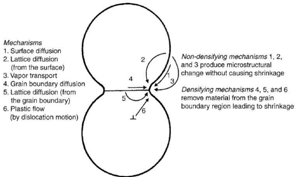
Figure 2.3. Six different mechanisms of sintering in polycrystalline materials (Source: De Jonghe and Rahaman 2003).
