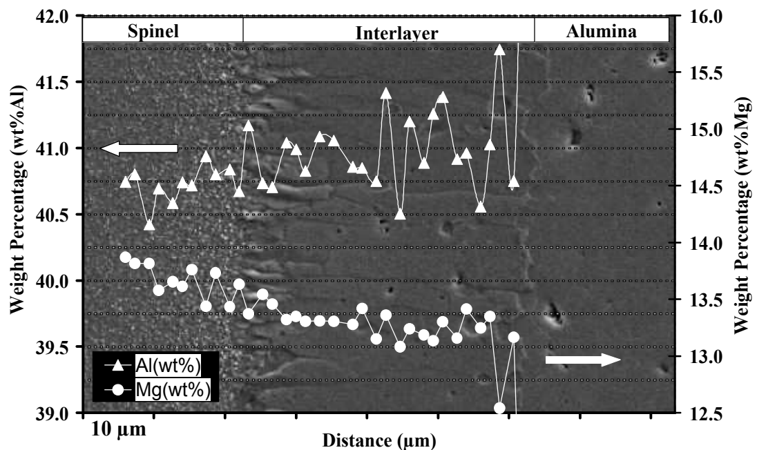
Figure 6.3. WDS analysis of the interlayer between spinel and alumina. Mg concentration slightly decreases from left to right. Al concentration increases in the same direction. Alumina A – spinel co-sintered samples (1500°C, 16 hours).
