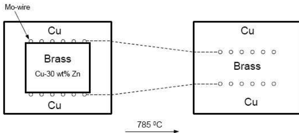
Figure 2.14. Schematic representation of a cross-section of the diffusion couples before and after annealing at 785°C (Source: Smigelkas and Kirkendall 1947).
