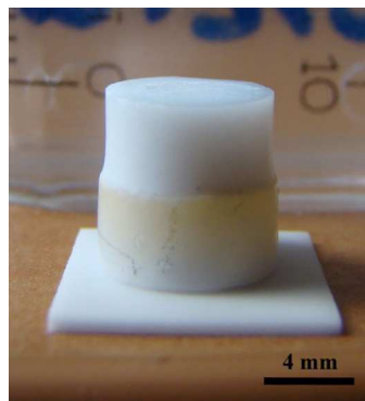
Figure 5.3. Photograph of a co-sintered alumina – spinel bi-material (1500°C – 4 hours) : the upper part is the spinel part.
