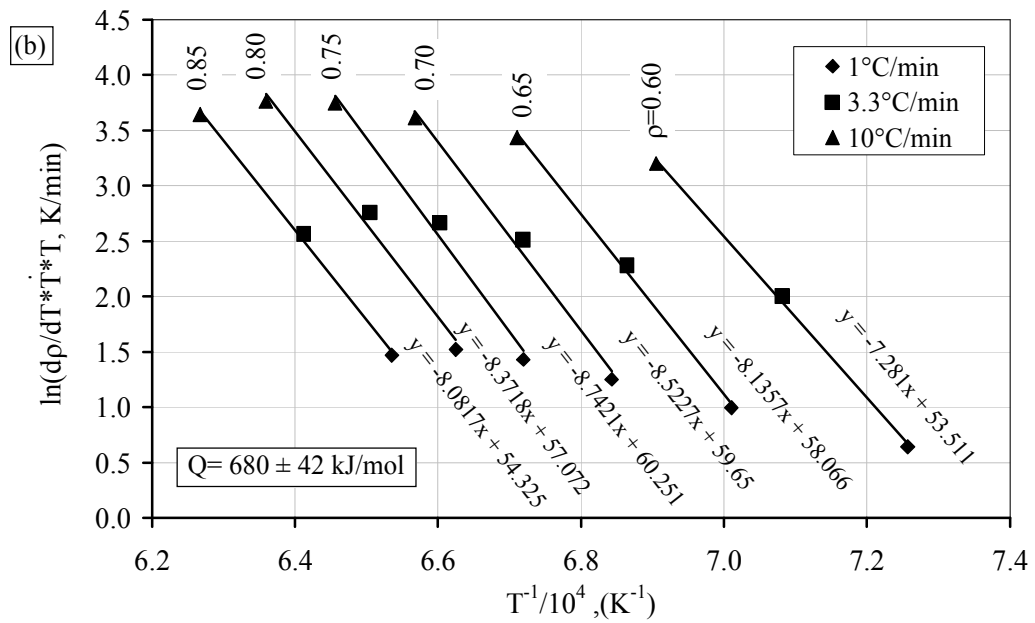
Figure 3.20. Arrhenius plots of constant heating rate sintering for pellets (CIP 250 MPa) of alumina A and (b) alumina B.
