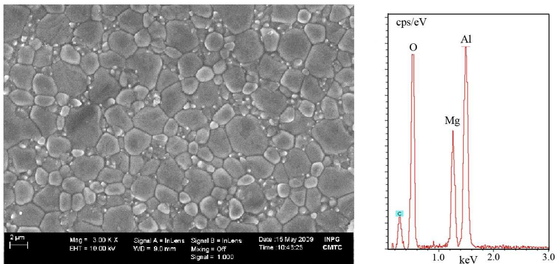
Figure 6.17. Point EDS analysis of a grain boundary of the alumina in a region out of nodules “matrix area”. Image obtained from surface of alumina end-member away from nodules (in Exp. No 1).
