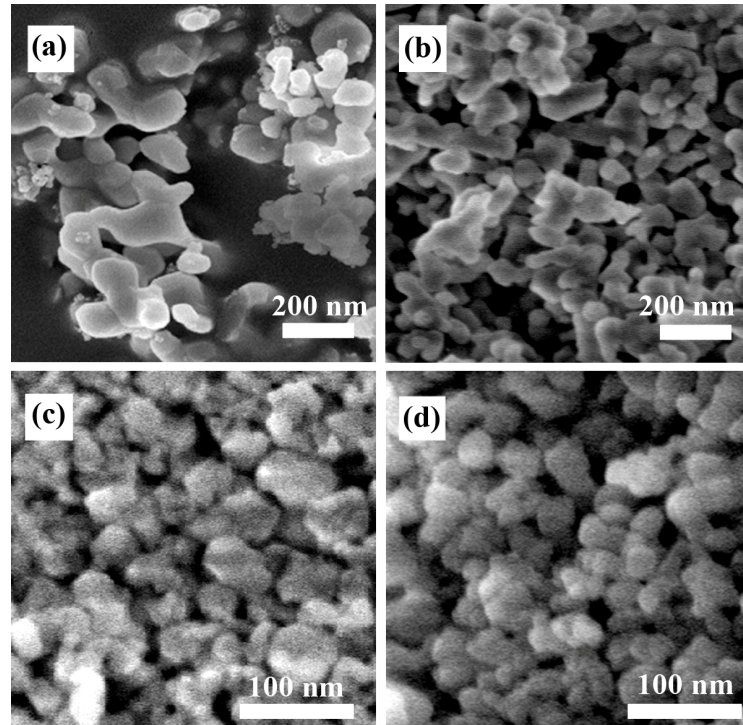
Figure 3.4. The primary particles of powders SEM images of (a) alumina A, (b) alumina B, (c) zirconia Z-3Y and (d) zirconia TZ-2Y.
