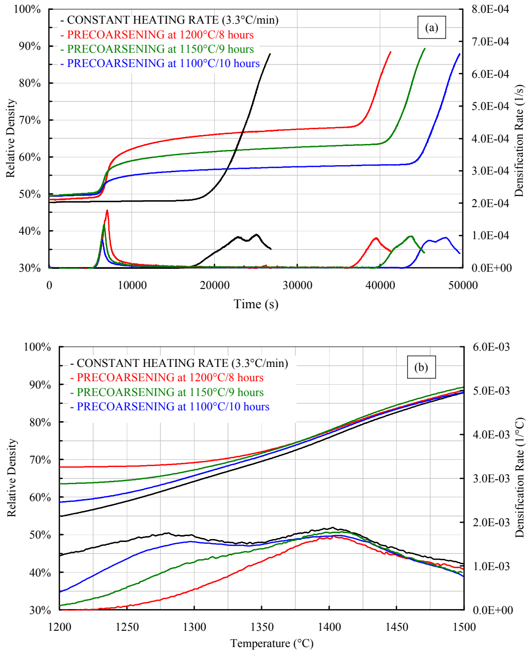
Figure 4.18. Densification and densification rate curves during sintering at a heating rate of 3.3°C/min for powder compacts of spinel with and without coarsening pre-treatments (a) The upper and lower curves are the relative densities, \rho , and their time derivatives, d\rho/dt , respectively respect to time (b) The upper and lower curves are the relative densities, and their temperature derivatives, d\rho/dT , respectively respect to temperature from 1200 to 1500°C.
