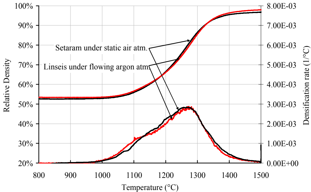
Figure 3.12. Comparison of the dilatometers and atmosphere effects on the densification and densification rate curves for powder compacts of alumina B (CIP 250 MPa and sintered with a 3.3 °C/min heating rate up to 1500°C).
