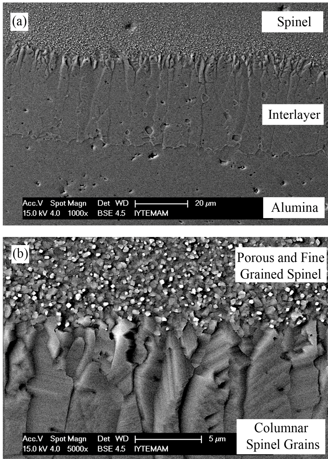
Figure 6.1. Interface microstructure of spinel – alumina A bi-material co-sintered for 16 hours at 1500°C with 3.3°C/min heating rate: (a) general view (b) a closer view of the porous and fine grained parent spinel and in-situ grown columnar grained spinel.
