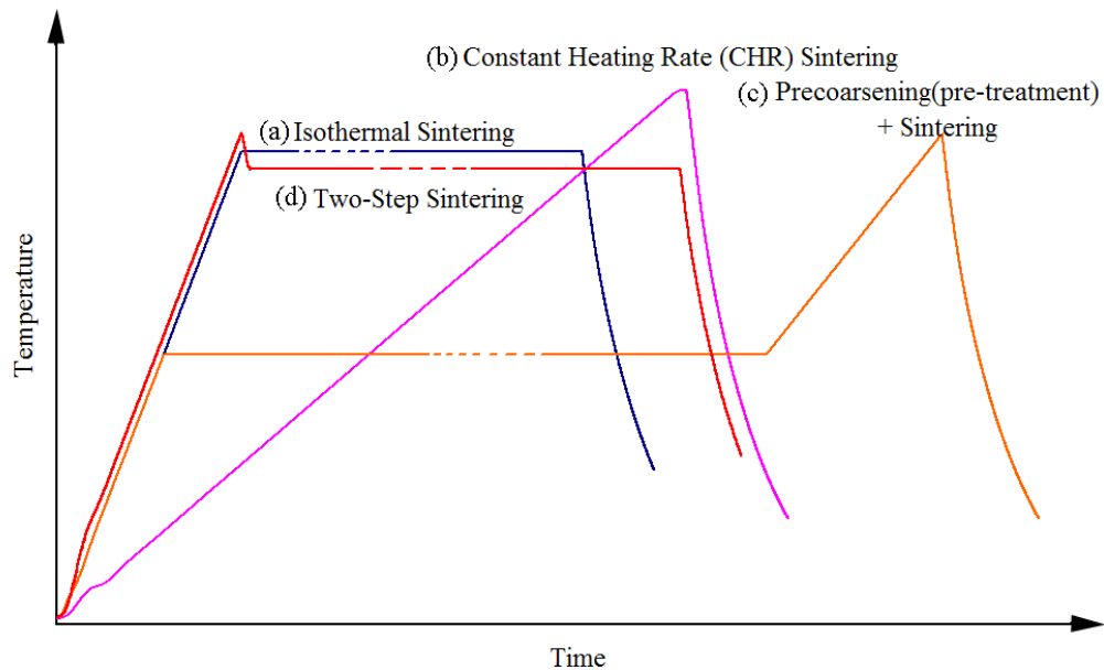
Figure 2.4. Sketch of the temperature-time schedule in a) isothermal, b) constant heating rate c) precoarsening (pretreatment) and d) two-step sintering.
