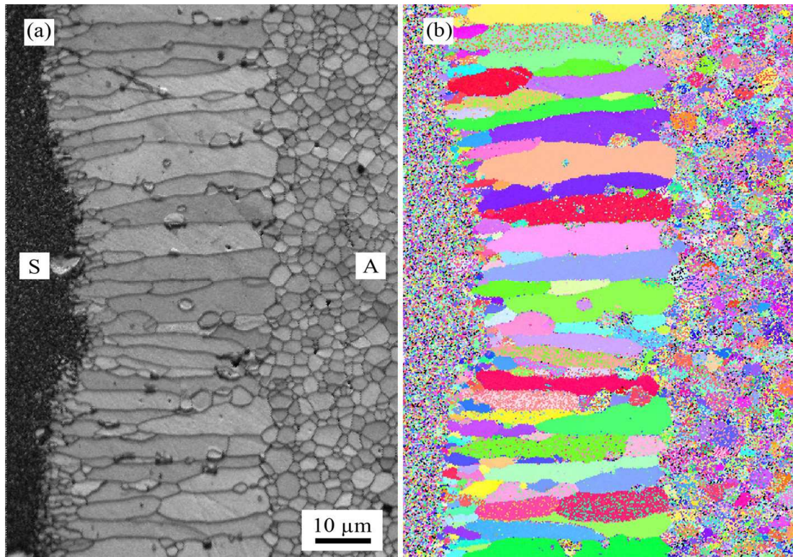
Figure 6.4. (a) Secondary electron SEM image and (b) EBSD image of interlayer of alumina A – spinel bi-material co-sintered at 1500°C for 16 hours.
