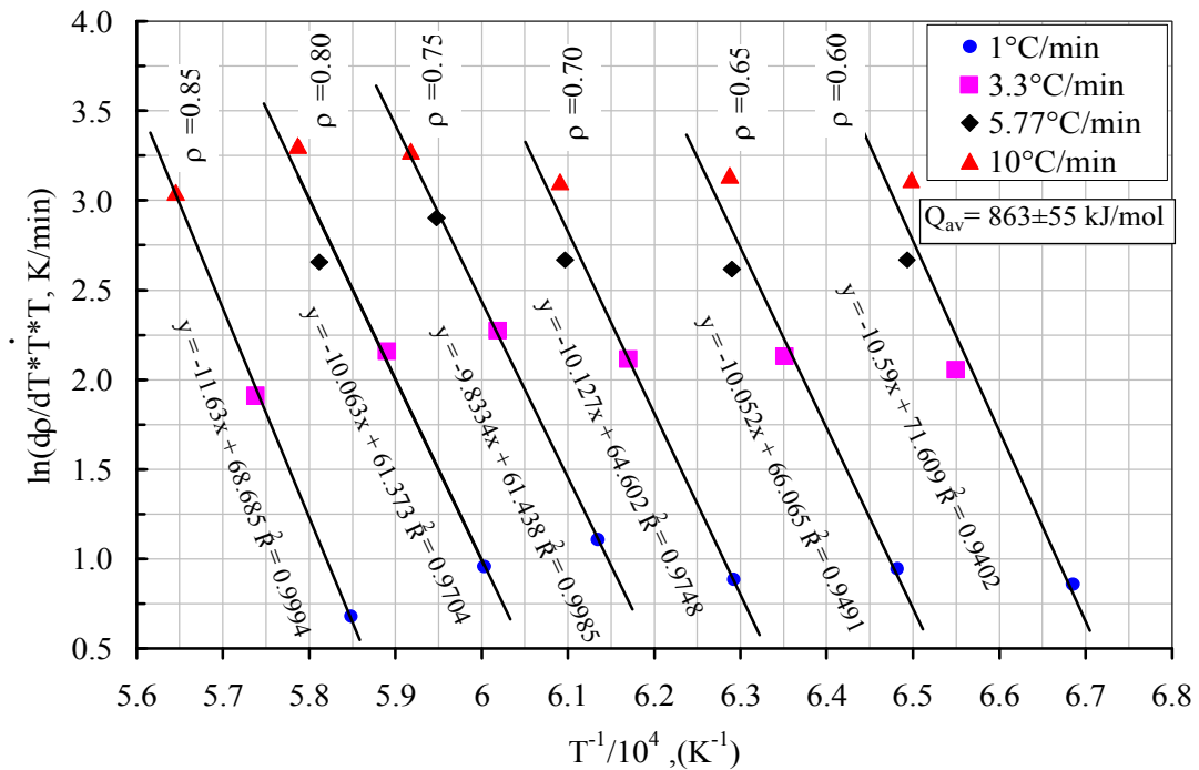
Figure 4.13. Arrhenius plots at various relative densities of powder compacts of spinel; from data of constant heating rate sintering tests.
