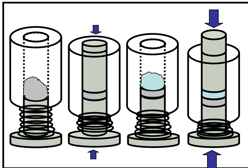
Figure 5.2. Schematic illustration of co-pressing method with floating die mode of pressing (Co-UPFlo).
