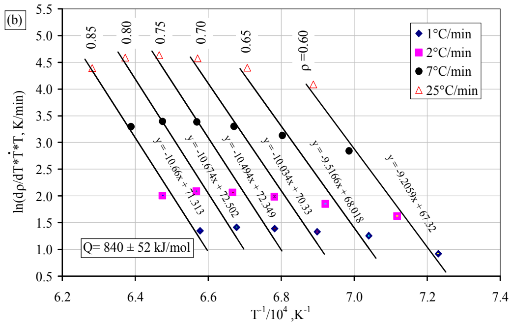
Figure 3.21. Arrhenius plots of constant heating rate sintering for pellets (CIP 250 MPa) of (a) zirconia Z-3Y and (b) zirconia TZ-2Y.
