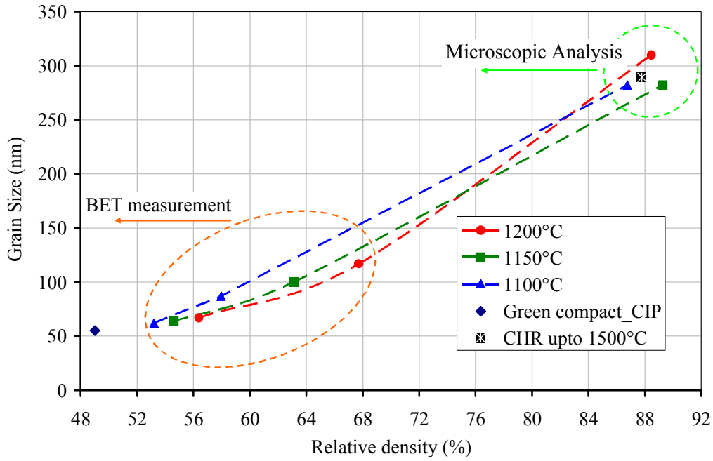
Figure 4.22. Effect of pretreatment on sintering path of spinel compacts : grain size versus relative density.
