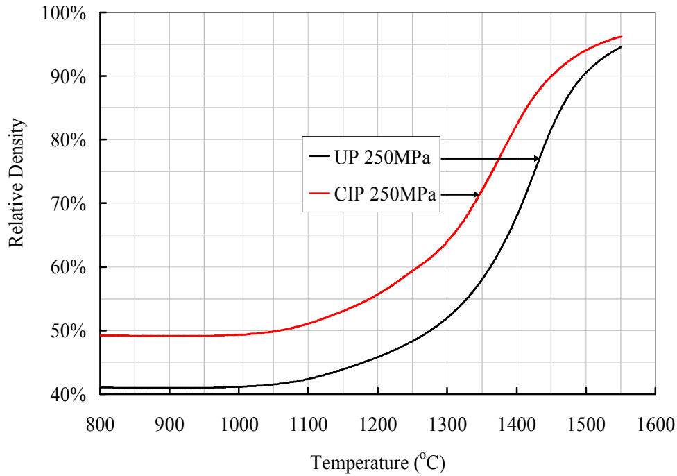
Figure 3.19. Effect of compaction process on the sintering of alumina A compacts, sintered with 3.3°C/min constant heating rate up to 1550°C.
