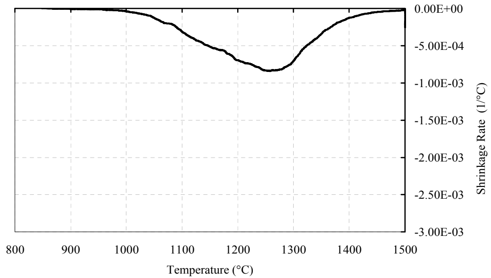
Figure 3.9. Shrinkage rate curve for powder compacts of alumina B (CIP 250 MPa) during sintering at a heating rate of 3.3°C/min.
