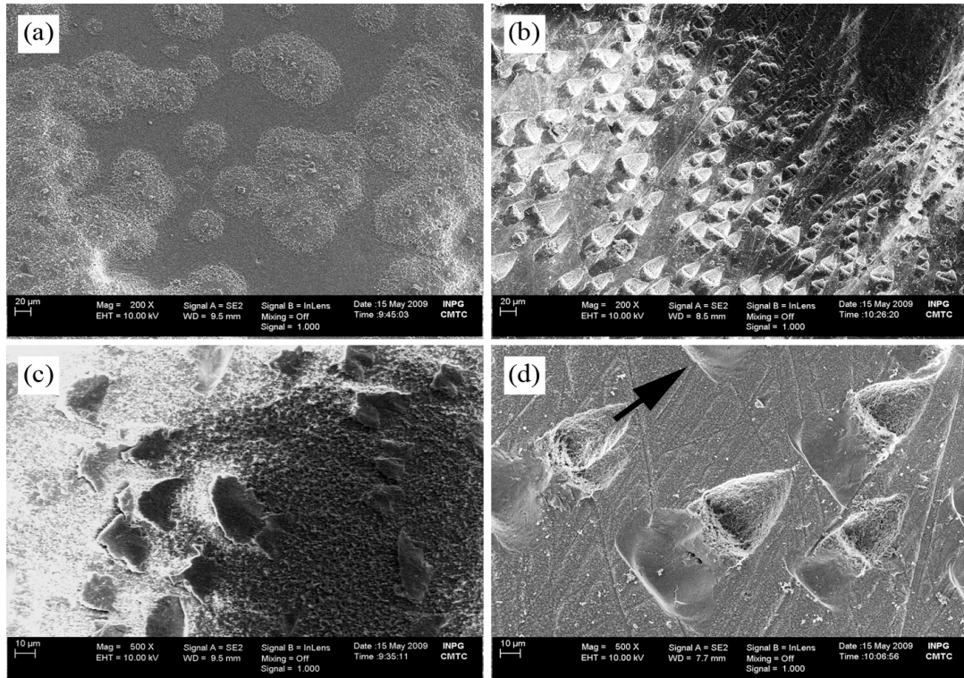
Figure 6.15. The SEM images of surfaces of the predensified alumina and spinel green compact end-members (a) and (c) alumina, (b) and (d) spinel.
