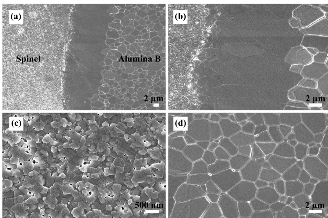
Figure 5.14. Spinel – alumina B bi-material, produced by single-action mode of uniaxial pressing at 250 MPa (Co-UP), (a) interlayer, (b) higher magnification of the interlayer, (c) spinel region close to interface, (d) alumina B region. Co-sintering conditions : 3.3°C/min up to 1580°C.
