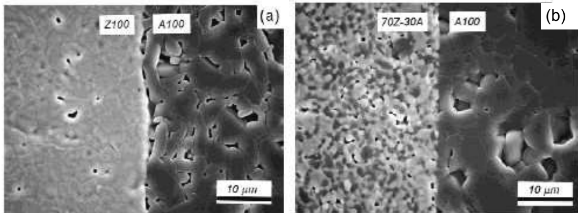
Figure 2.12. SEM micrograph showing the microstructure of (a) A100/Z100, and (b) A100/Z70 symmetric laminates (Source : Cai, et al. 1997a).
