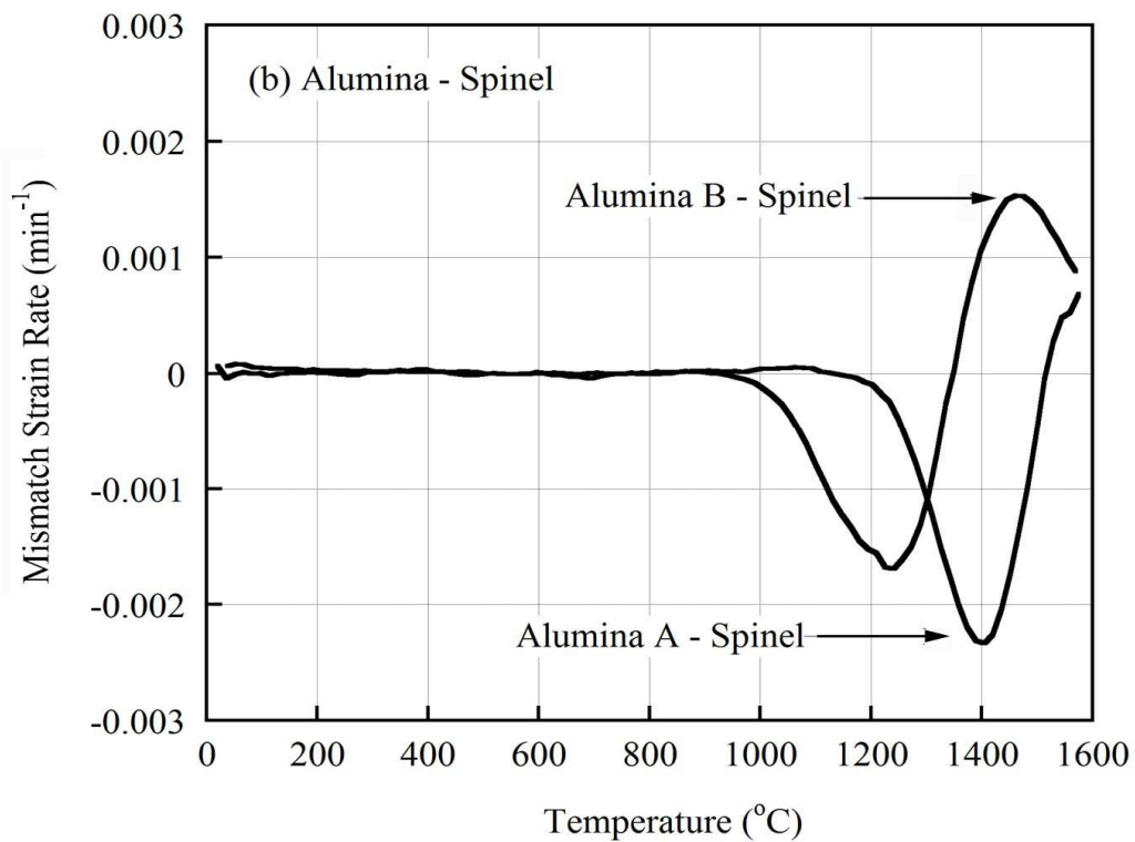
Figure 5.6. Mismatch strain rates of individual powder compacts (UP 250 MPa) of (a) alumina – zirconia, (b) alumina – spinel sintered up to 1580°C with heating rate of 3.3°C/min.
