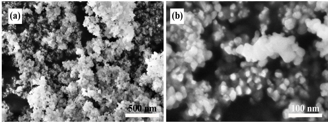
Figure 4.2. SEM images of spinel powder with different magnifications.
