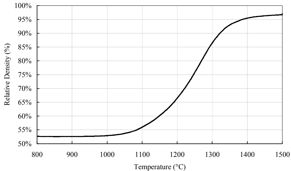
Figure 3.10. Relative density curve for powder compacts (CIP 250 MPa) of alumina B during sintering at a heating rate of 3.3°C/min.
