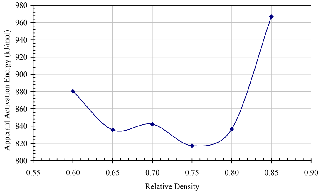
Figure 4.14. Apparent activation energy for densification versus relative density.
