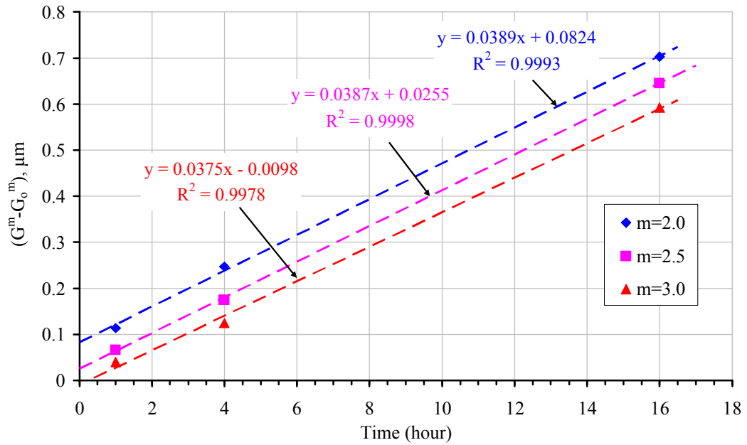
Figure 4.11. Grain growth laws at 1500°C of sintered spinel material.
