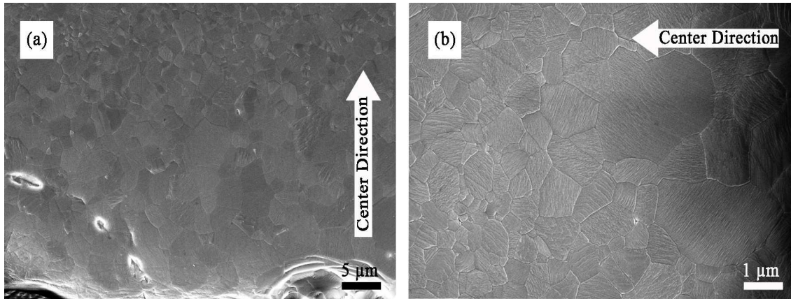
Figure 4.12. SEM images of polished cross sections of a 96% dense sintered spinel samples close to their outer edges (10°C/min at 1500 C for 10 hours).
