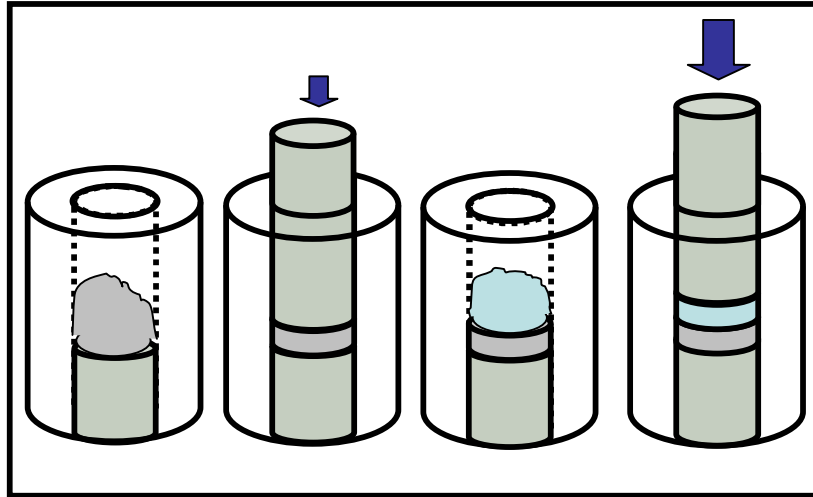
Figure 5.1. Schematic illustration of uniaxial single action co-pressing method (Co-UP).
