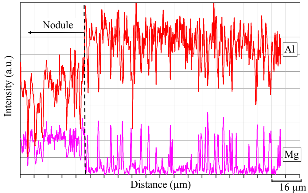
Figure 6.16. Line EDS analysis of contact surface of alumina (Exp. no 1). The surface of the nodule was richer in Mg compared to the rest of the surface.
