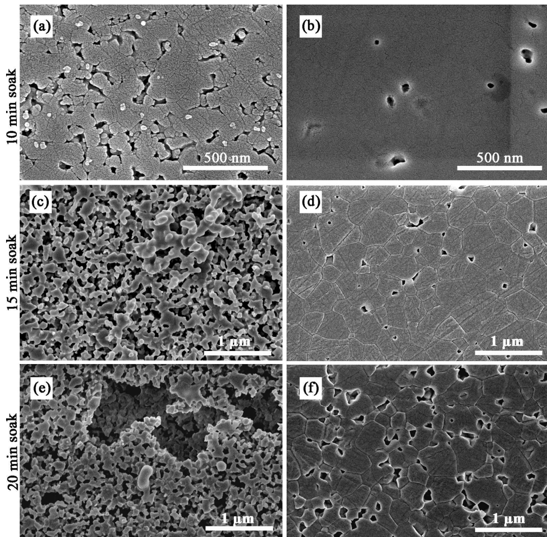
Figure 4.6. Surfaces of chemically etched spinel ceramics; (a), (c), (e) 85% relative density and (b), (d), (f) 99% relative density, they were held 10, 15 and 20 min inside the hot acid from top row to bottom row, respectively.
