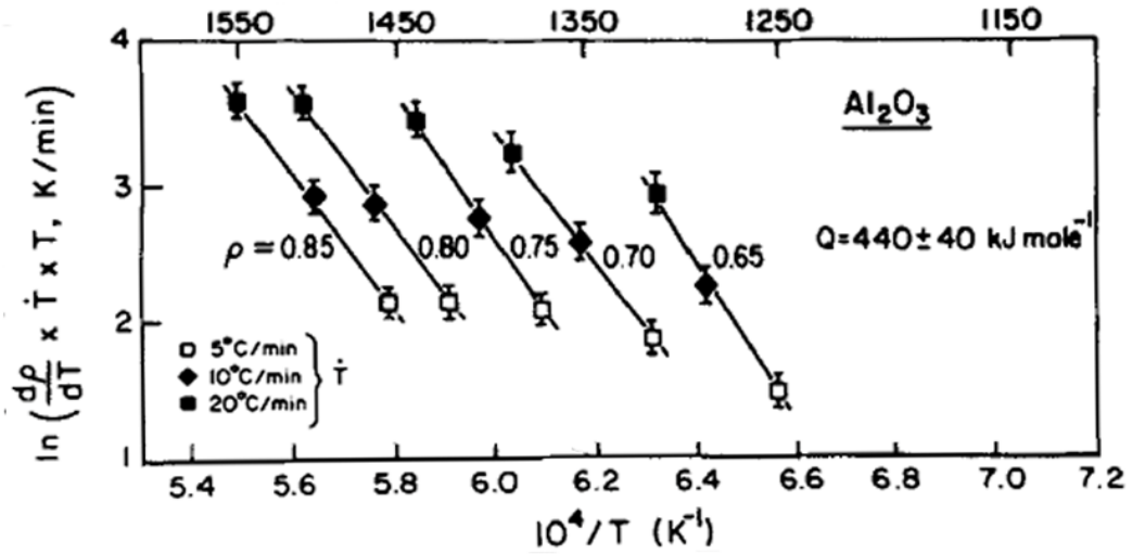
Figure 2.7. Arrhenius plots of alumina and the estimated activation energy using the method described in the text (Source: Wang and Raj 1990).
