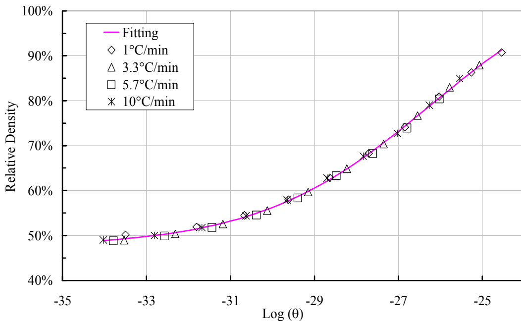
Figure 4.15. Master Sintering Curve of spinel compacts : Relative density as a function of the master sintering variable (cold pressing conditions : UP 50 MPa + CIP 250 MPa).
