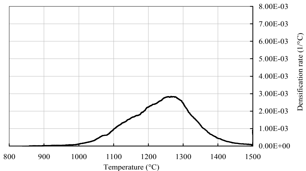
Figure 3.11. Densification rate curve for powder compacts of alumina B (CIP 250 MPa) during sintering at a heating rate of 3.3°C/min.
