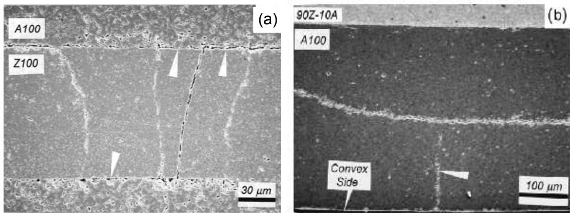
Figure 2.11. Typical defects observed in the symmetric laminates: (a) debonding cracks and (b) channel cracks (Source : Cai, et al. 1997a).
