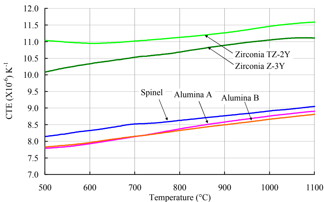
Figure 5.11. Thermal Expansion Coefficients of mono-materials up to 1100°C. Dilatometric data obtained with nearly fully dense samples during the heating step of a thermal cycle (10°C/min).
