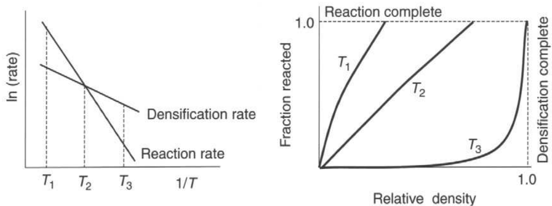
Figure 2.2. Schematic relationship between densification rate and reaction rate as a function of temperature T , and the resulting process trajectory. If the reaction rate is fast compared to densification, complete reaction can occur with limited densification (Source: Yangyun and Brook 1985).
