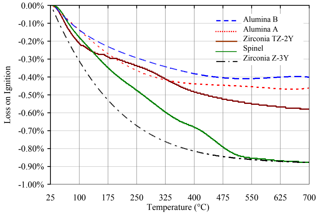
Figure 3.5. TGA results of the powders.
