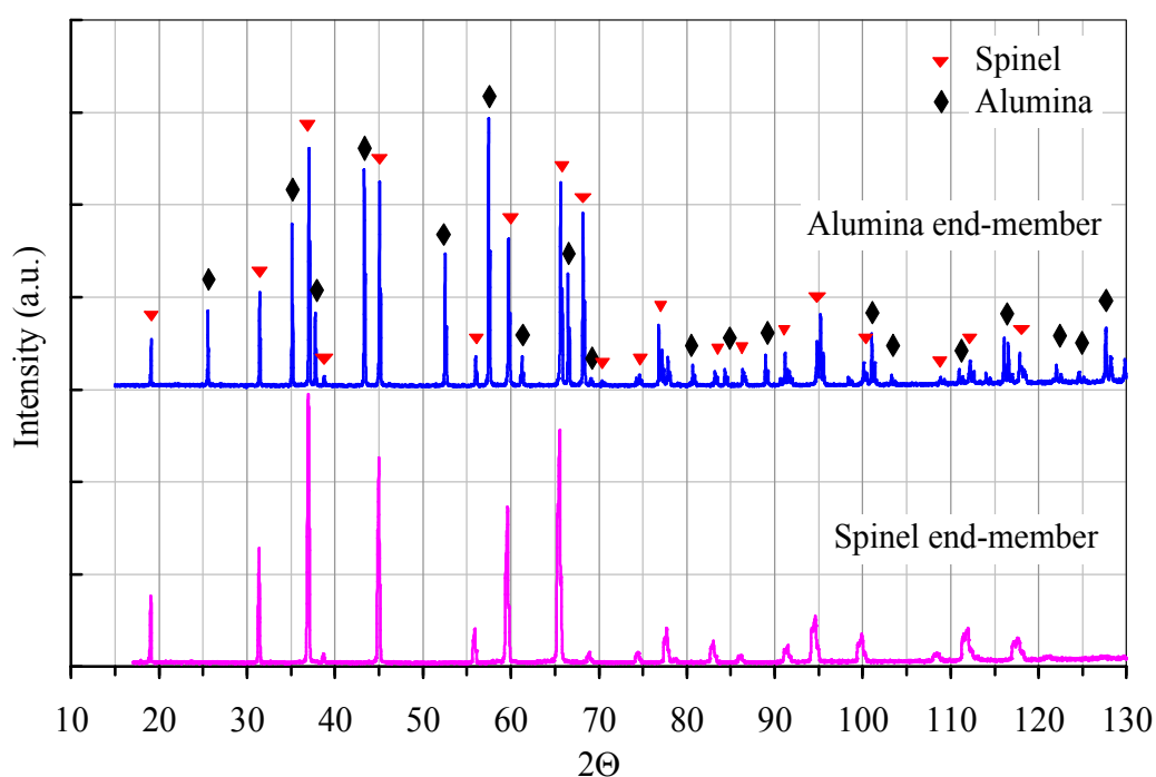
Figure 6.19. The XRD patterns of alumina and spinel end-members after diffusion couple test n°1.
