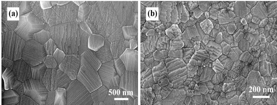
Figure 4.3. Thermally etched surface of spinel ceramics (a) spinel has 99% relative density and (b) spinel has 85% relative density.
