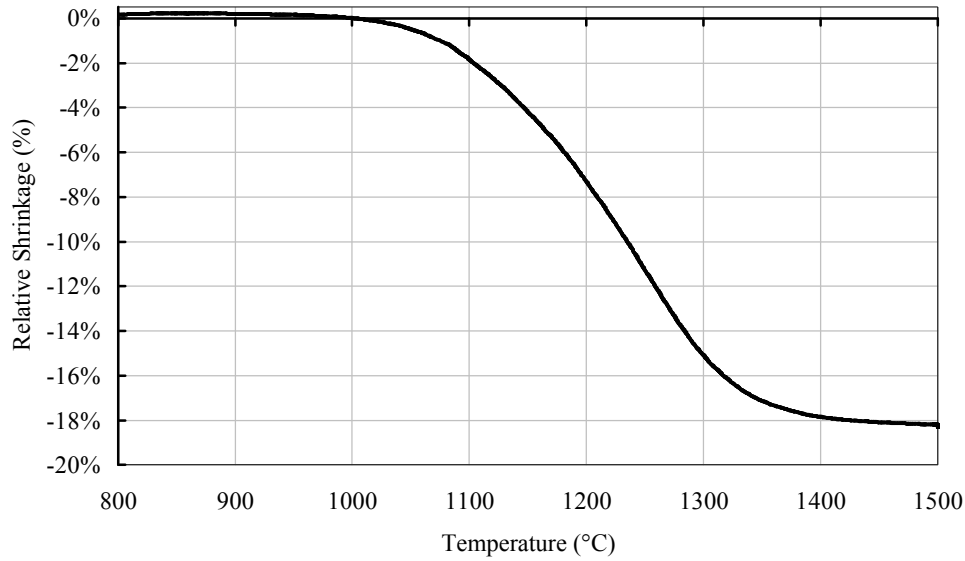
Figure 3.8. Relative shrinkage curve for powder compacts (CIP 250 MPa) of alumina B during sintering at a heating rate of 3.3°C/min.
