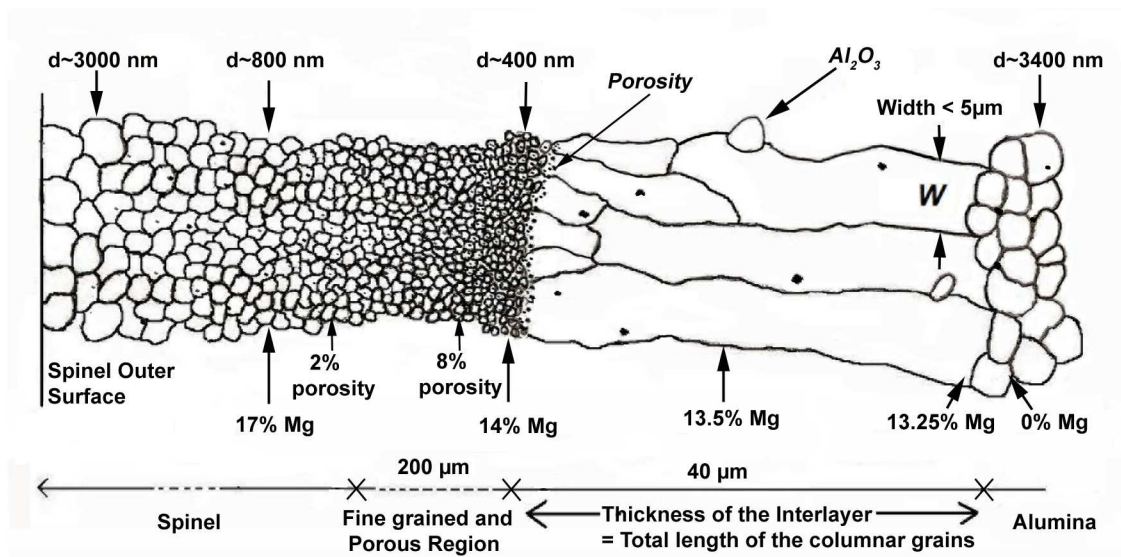
Figure 6.2. Schematic illustration of bi-material (alumina A – spinel) microstructure co-sintered for 16 hours at 1500°C.
