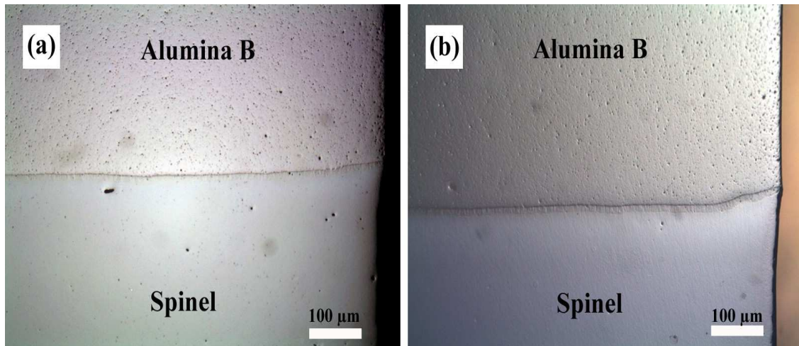
Figure 5.9. Optical Microscope image of bonding regions of spinel – alumina B bi-materials, produced by single-action mode of uniaxial pressing at 100 MPa followed by cold isostatic pressing at 250 MPa (Co-UP+CIP). They were co-sintered at 1500°C for (a) 4 and (b) 16 hours.
