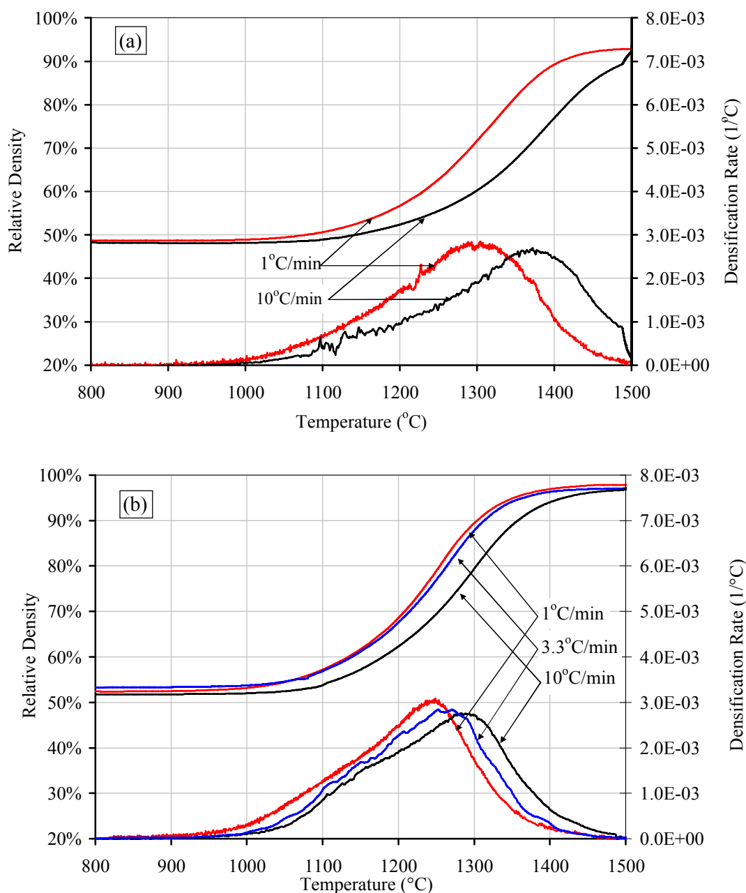
Figure 3.13. Densification curves during sintering at heating rates of 1, 3.3 and 10°C/min for powder compacts of (a) alumina A and (b) alumina B. The upper and lower curves in all (a) and (b) are the relative densities, \rho , and their temperature derivatives, d\rho/dT , respectively (all the samples were CIPed at 250 MPa).
