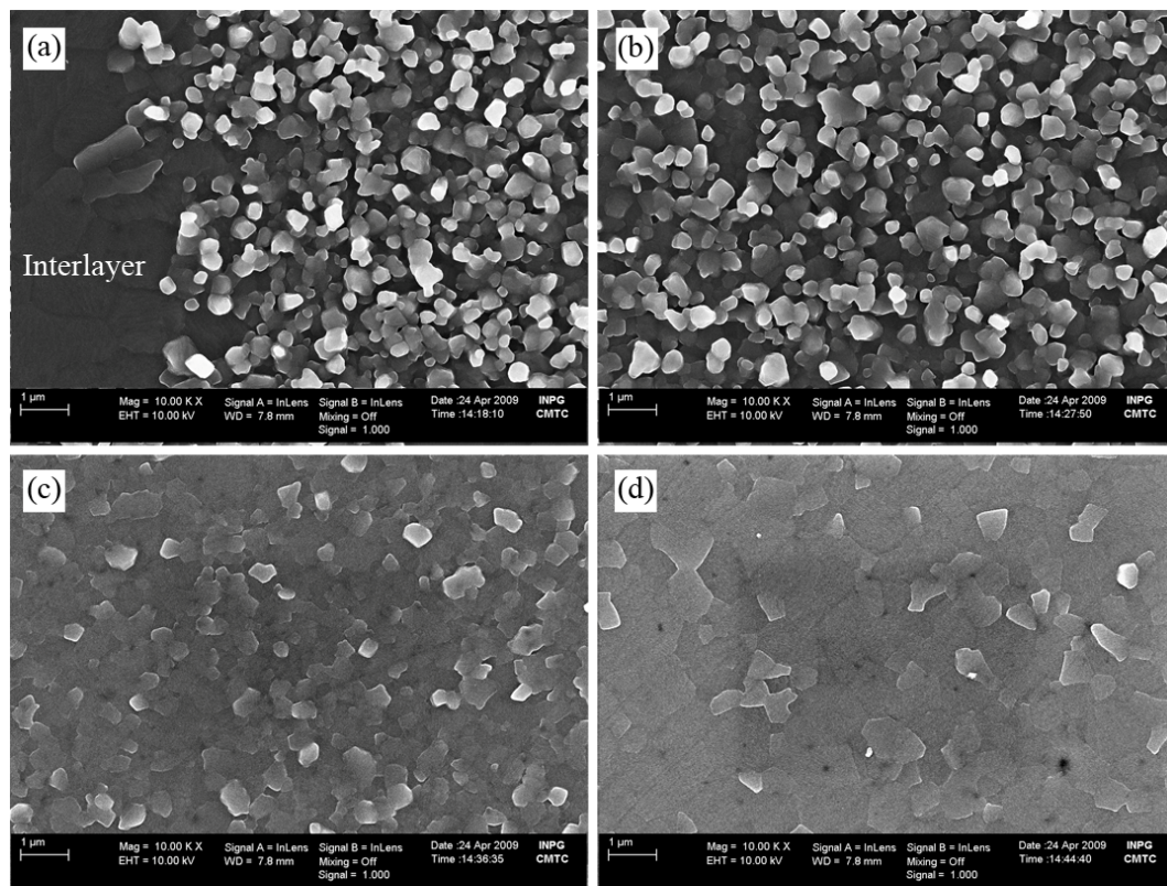
Figure 6.5. Porous region in parent spinel end-member in alumina B – spinel bi-material (a) near the interlayer, (b) 40 \mu\text{m} , (c) 90 \mu\text{m} , and (d) 360 \mu\text{m} away from the interlayer into bulk of the parent spinel. The bi-material was co-sintered at 1500°C for 16 hours with 3.3°C/min heating rate.
