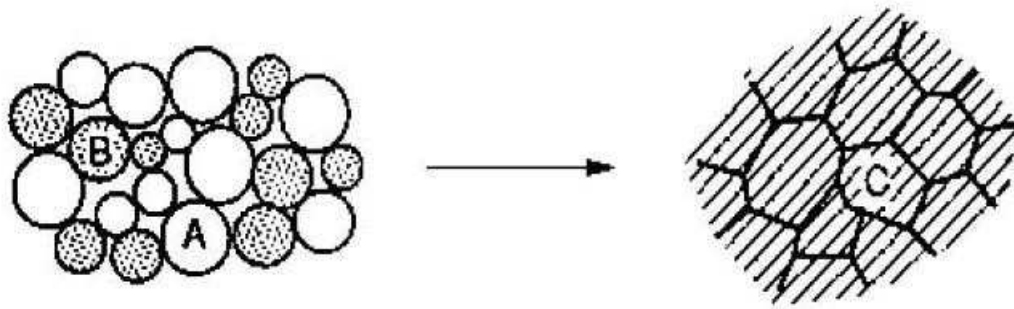
Figure 2.1. Schematic diagram illustrating the production of, a single-phase solid, C, by reaction sintering of a compacted mixture of two powders, A and B (Source: Yangyun and Brook 1985).
