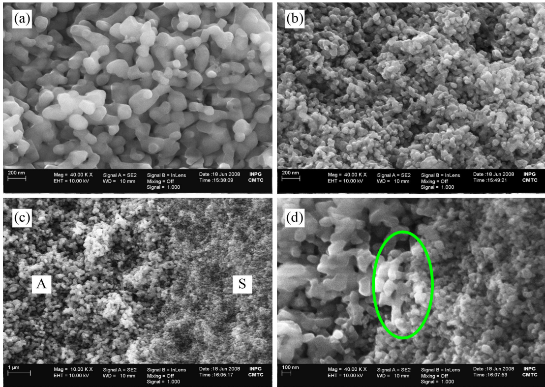
Figure 6.8. SEM image of the fracture surface of alumina – spinel bi-material co-sintered at 1150°C for 16 hours. (a) and (b) show the initial stage sintering of alumina and spinel part, (c) and (d) the interface region between alumina and spinel at different magnifications. A: alumina and S: spinel.
