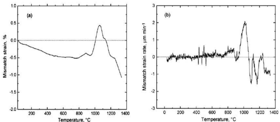
Figure 2.10. Mismatch strain (a) and strain rate (b) between 17-4PH and 316L stainless steel layers during non-isothermal sintering in hydrogen. (Source : Simchi, et al. 2006a).
