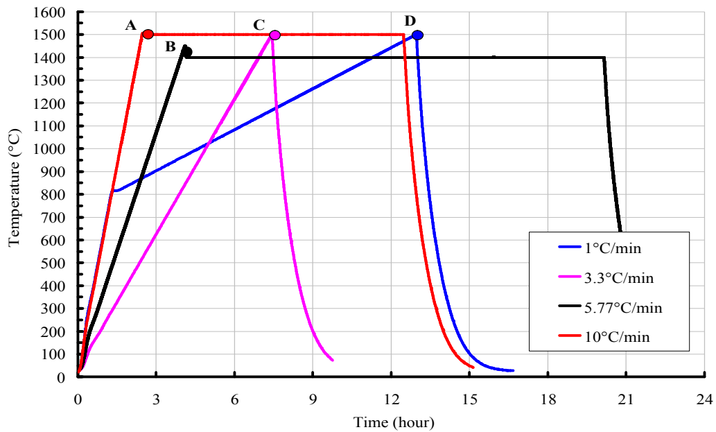
Figure 4.7. Temperature versus time schedules of sintering tests.
