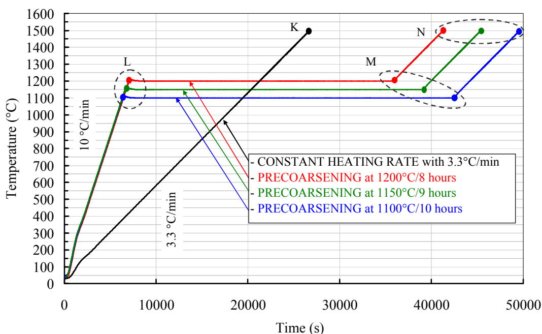
Figure 4.17. Heating schedules of precoarsening treatments on spinel compacts. Sample K was heated at constant heating rate (3.3°C/min) up to 1500°C. Samples of the group L were heated at 1100°C, 1150°C and 1200°C and were cooled without a soaking time. Samples of the group M were soaked at these temperatures for 8-10 hours and then cooled. Samples of the group N after same group M soaking time were directly heated at a rate of 3.3°C/min up to 1500°C and cooled without soaking time at 1500°C.
