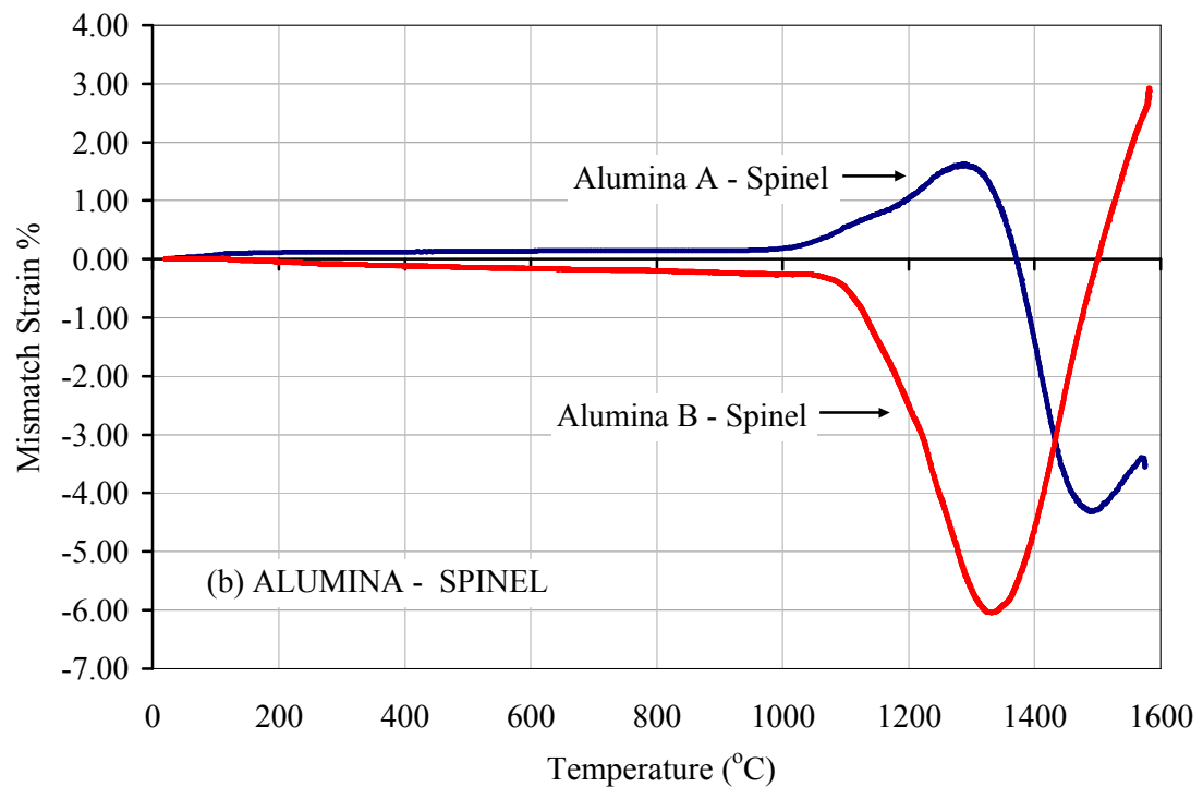
Figure 5.5. Mismatch strains of individual powder compacts of (a) alumina – zirconia, alumina – spinel, (UP 250 MPa) sintered at 1580°C with heating rate of 3.3°C/min.
