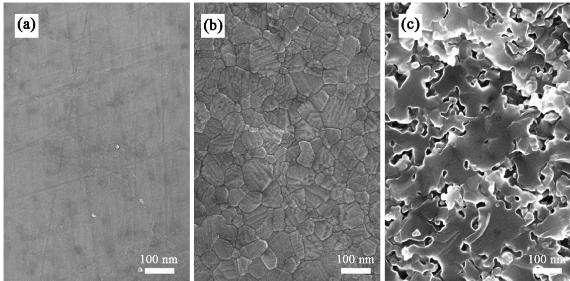
Figure 4.5. Scanning electron micrographs of (a) polished, (b) polished and thermally etched and (c) fractured surfaces of spinel ceramic sintered at 10°C/min until 1350°C for 10 hours, the specimen has the final relative density of 85%.
