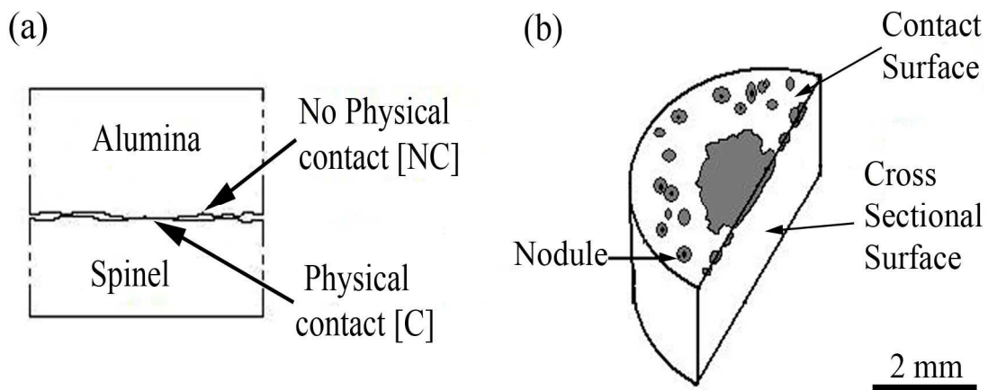
Figure 6.12. Illustration of diffusion couple test sample (a) before and (b) after thermal treatment (alumina A – spinel sintered at 1500°C for 16 hours).
