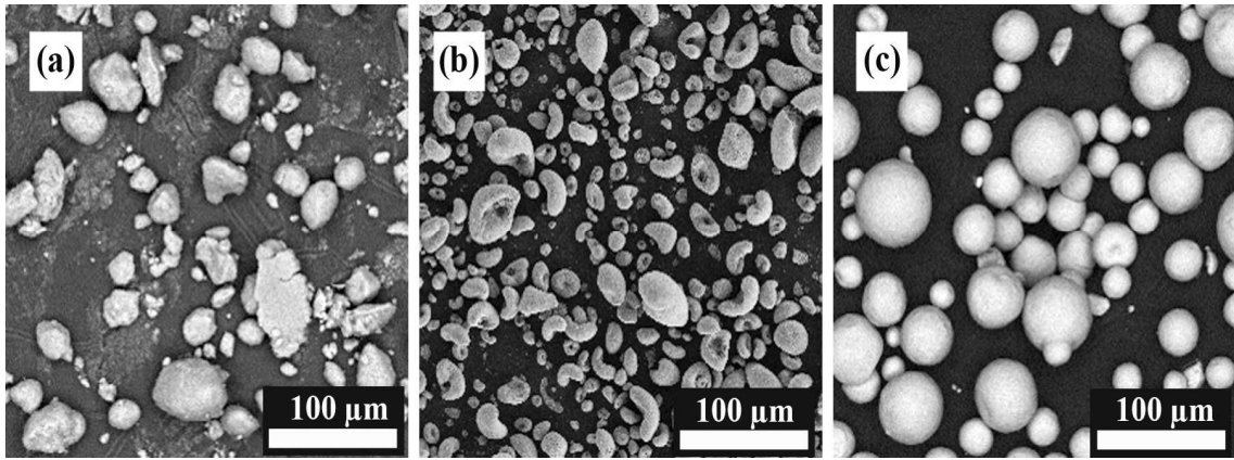
Figure 3.2. SEM images of the powders (a) alumina B, (b) zirconia Z-3Y and (c) zirconia TZ-2Y.
