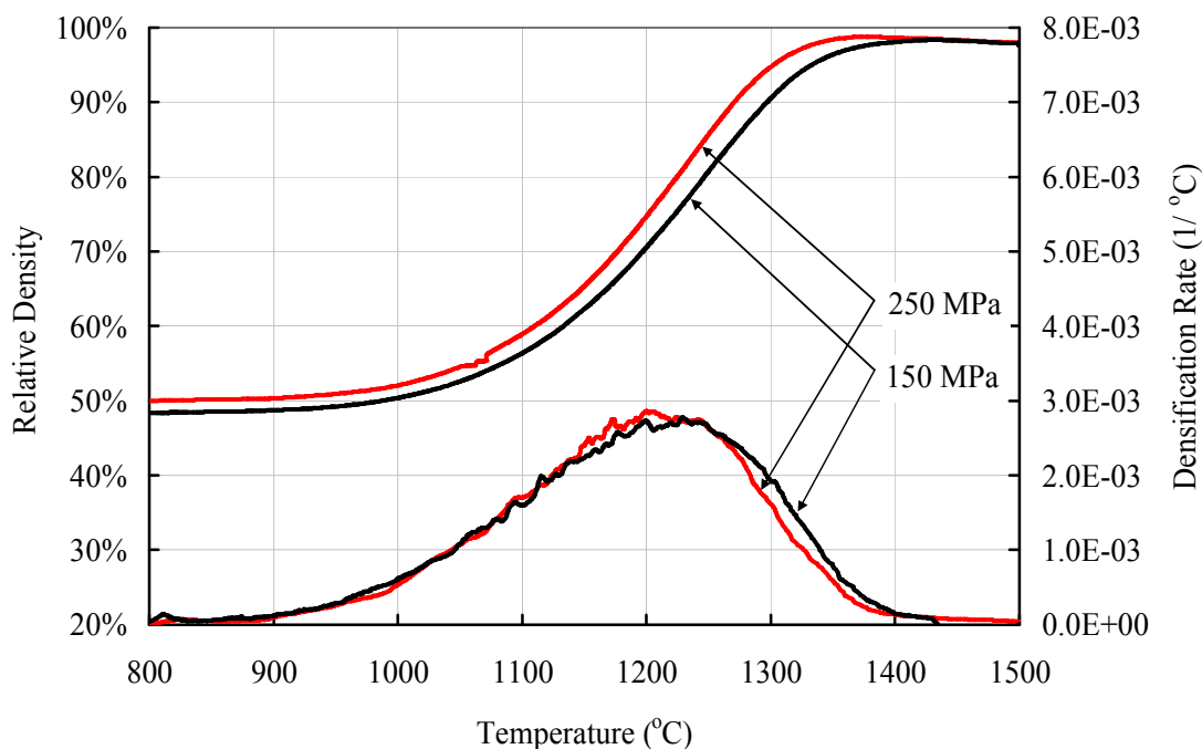
Figure 3.17. Effect of CIP compaction pressure on the sintering of zirconia TZ-2Y, 1°C/min heating rate.
