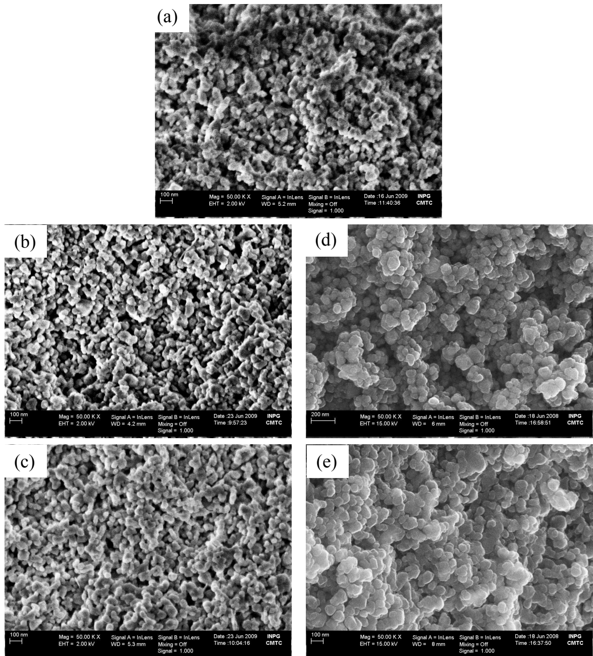
Figure 4.19. Scanning electron micrographs of fracture surfaces of spinel compacts showing the effect of the pretreatment on the microstructure before the sintering step at high temperature: (a) as compacted, (b) and (c) heated at 10°C/min until 1100°C (1100L) and 1200°C (1200L), respectively (d) and (e) pre-treated at 1100°C for 10 hours (1100M10) and at 1200°C for 8 hours (1200M8), respectively.
