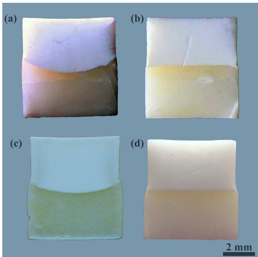
Figure 5.8. Shape of alumina B – spinel bi-materials, produced by different co-pressing techniques at final pressure of 250 MPa (a) Co-UP, (b) Co-UPFlo, (c) Co-UP+CIP and (d) Co-UPFlo+CIP. (Spinel part at the top in all photos) Co-sintering conditions : 1°C/min up to 1580°C.
